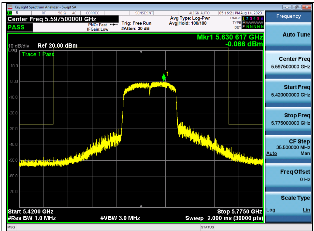
Test_Graph_802.11ac80_ANT1_5610_MCS9_Frequency Band 3
