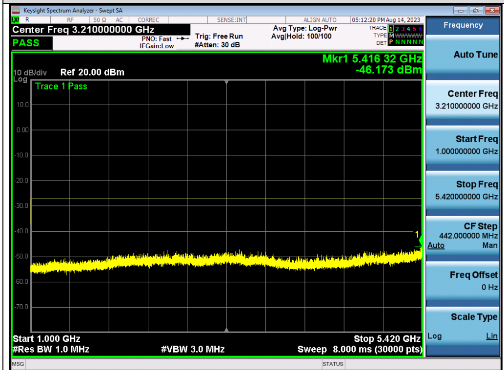
Test_Graph_802.11ac80_ANT1_5530_MCS9_Frequency Band 2
