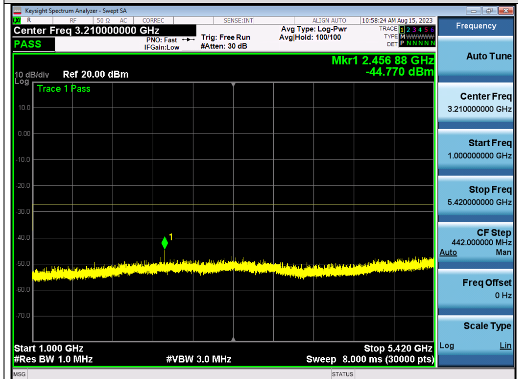
Test_Graph_802.11a_ANT2_5700_6Mbps_Frequency Band 2
