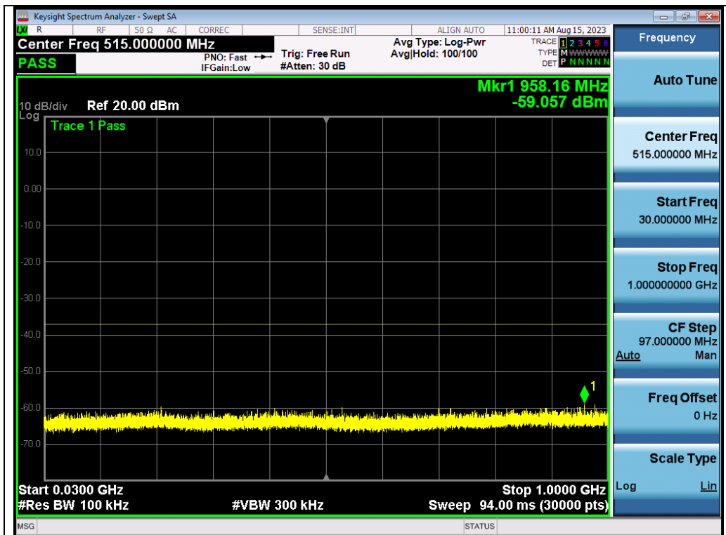
Test_Graph_802.11a_ANT2_5500_6Mbps_Frequency Band 1
