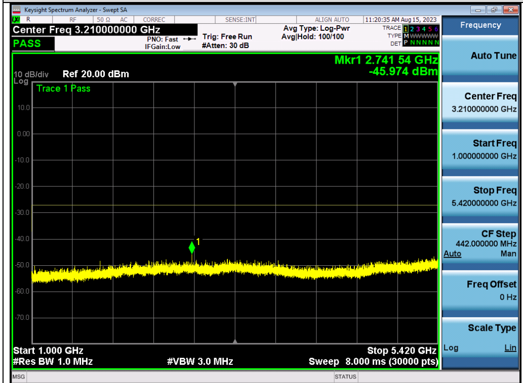
Test_Graph_802.11ac80_ANT2_5530_MCS9_Frequency Band 2
