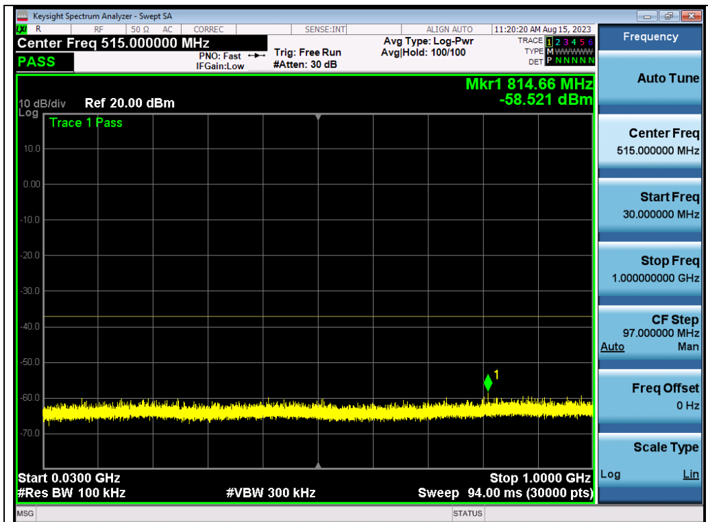
Test_Graph_802.11ac80_ANT2_5530_MCS9_Frequency Band 1
