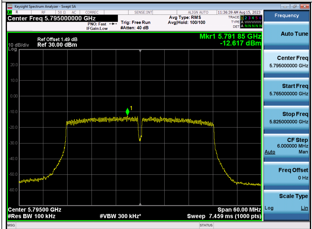
Test_Graph_802.11n40_ANT2_5795_MCS0_PSD
