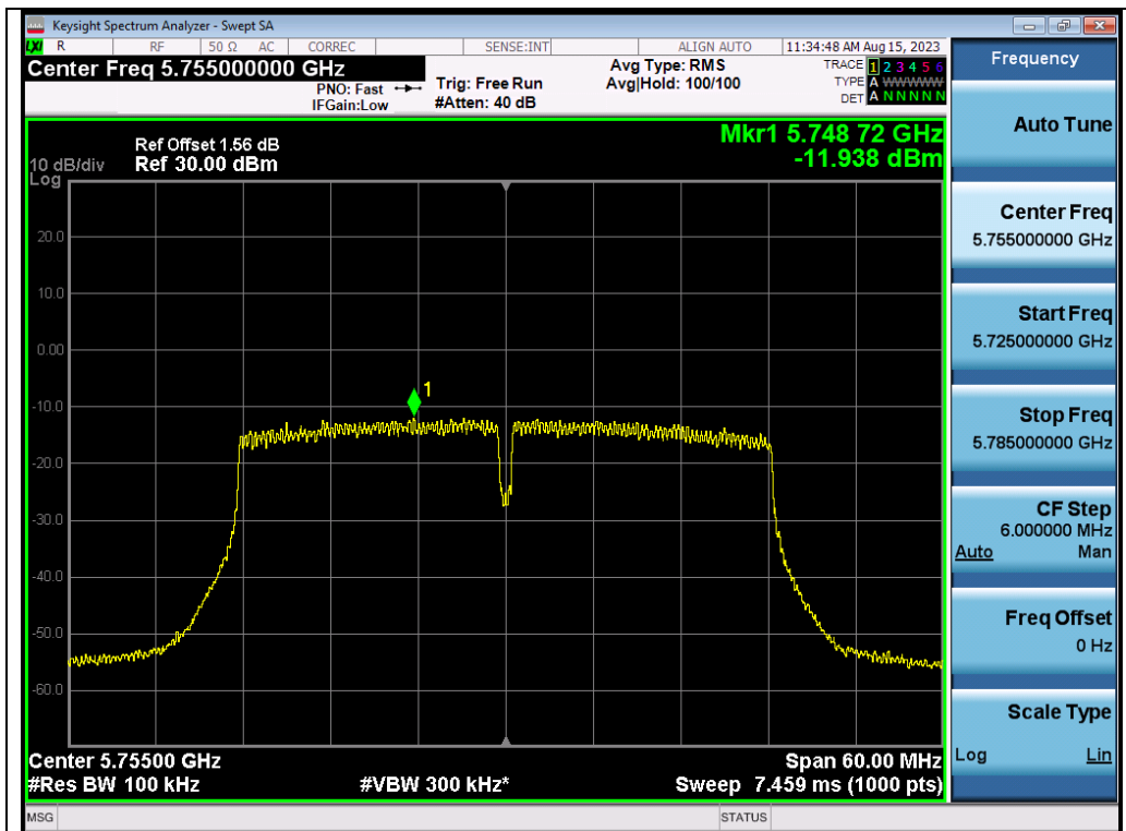
Test_Graph_802.11n40_ANT2_5755_MCS0_PSD
