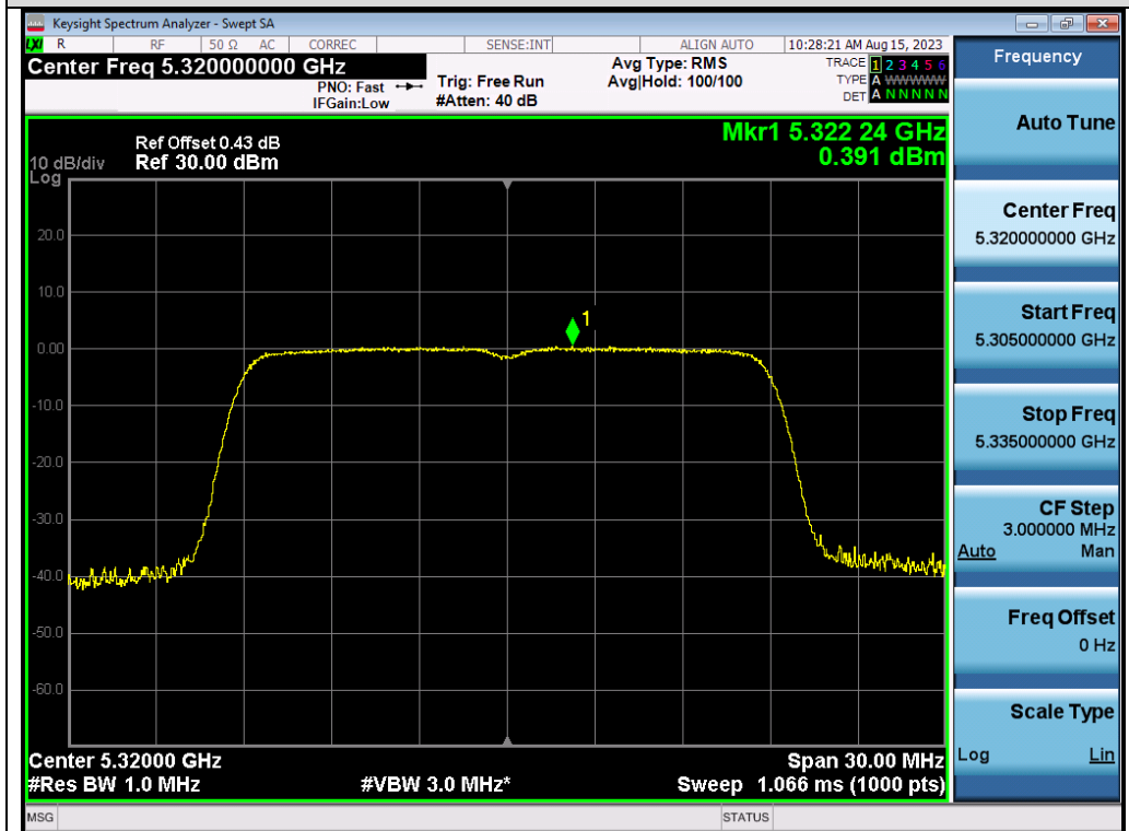
Test_Graph_802.11n20_ANT2_5320_MCS0_PSD
