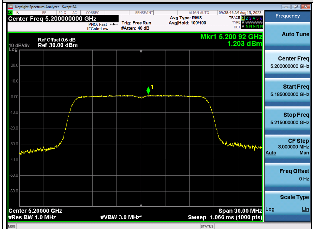
Test_Graph_802.11a_ANT2_5200_6Mbps_PSD
