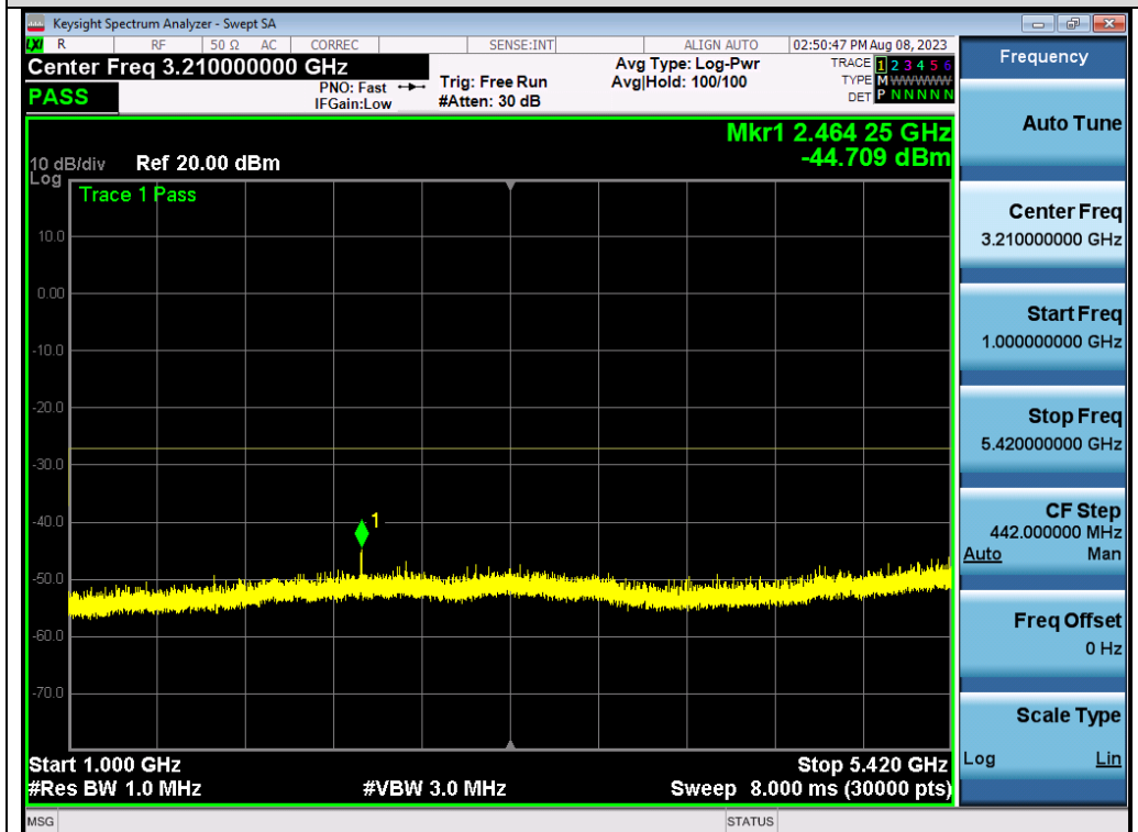
Test_Graph_802.11n40_ANT2_5670_MCS0_Frequency Band 2
