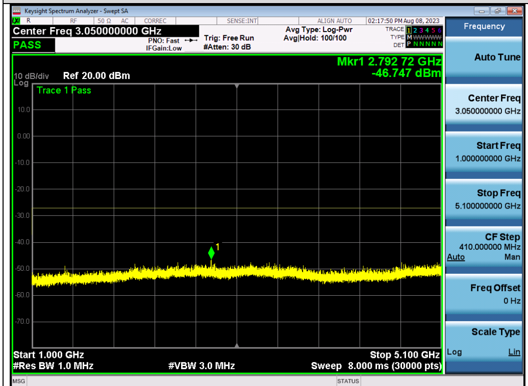
Test_Graph_802.11n40_ANT2_5310_MCS0_Frequency Band 2
