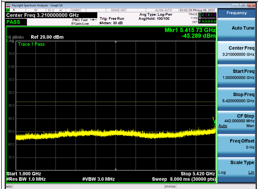
Test_Graph_802.11ac80_ANT2_5610_MCS9_Frequency Band 2
