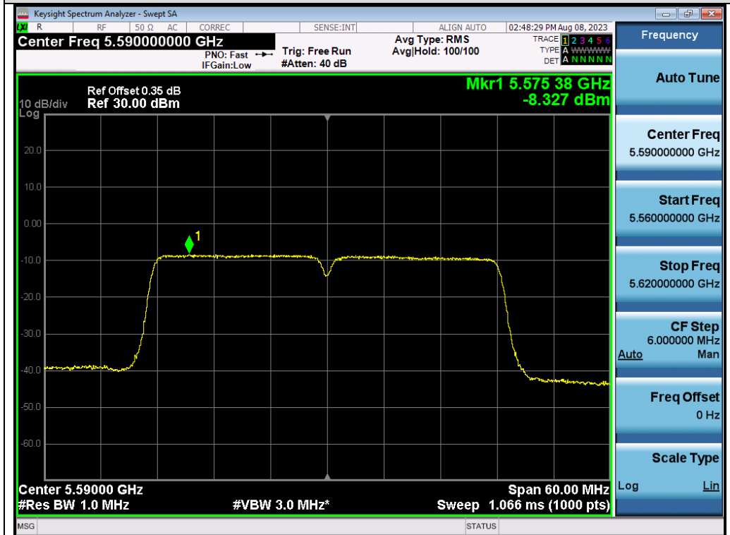
Test_Graph_802.11n40_ANT2_5590_MCS0_PSD
