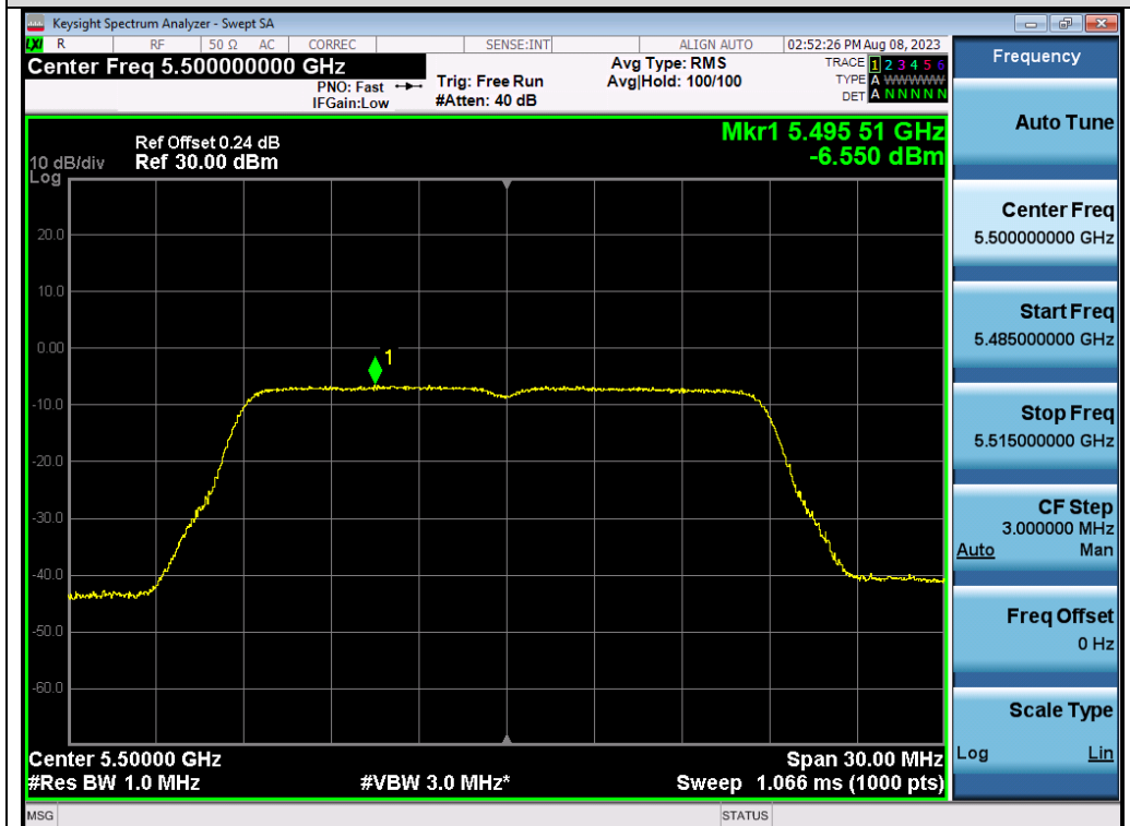
Test_Graph_802.11ac20_ANT2_5500_MCS0_PSD
