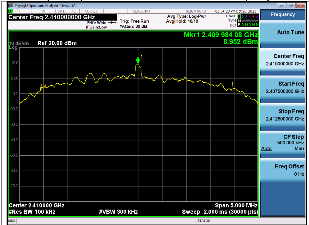
Test_Graph_GFSK_ANT1_2410_Reference Level
