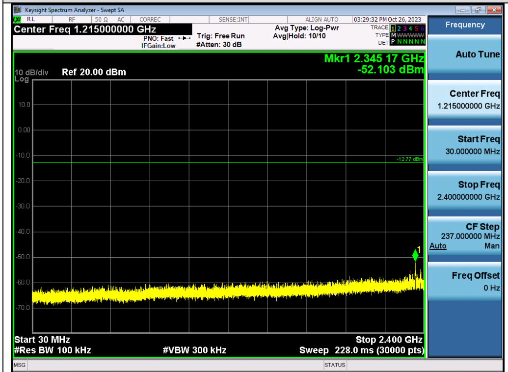
Test_Graph_GFSK_ANT1_2473_Lower Band Emissions
