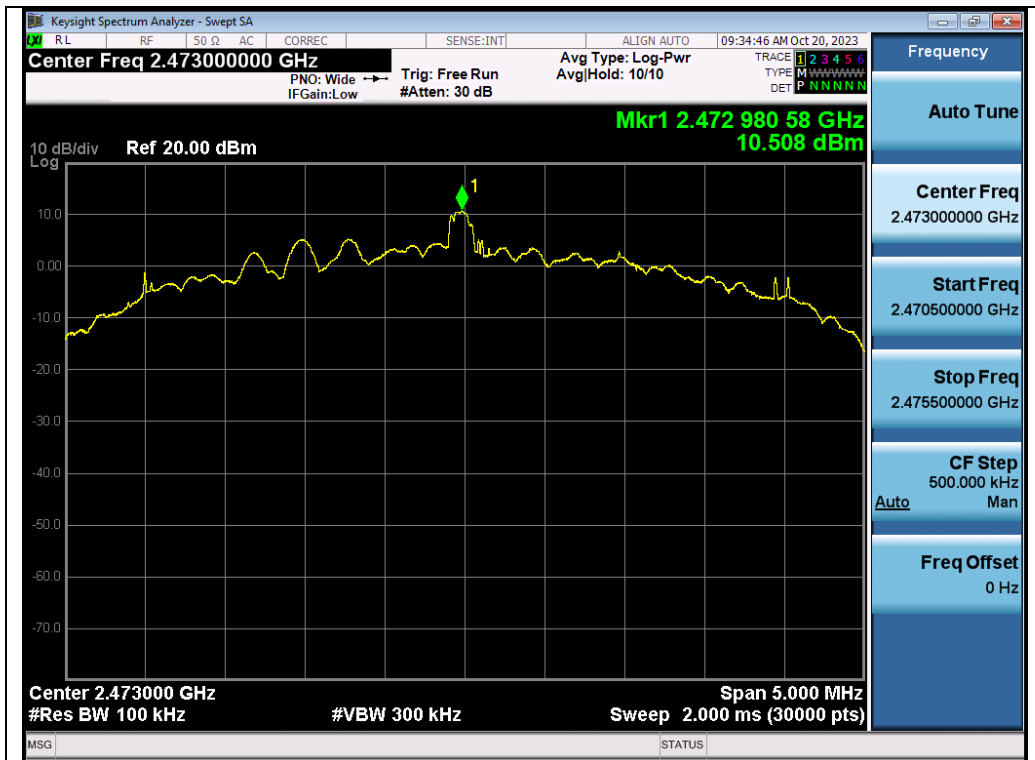
Test_Graph_GFSK_ANT1_2473_Reference Level
