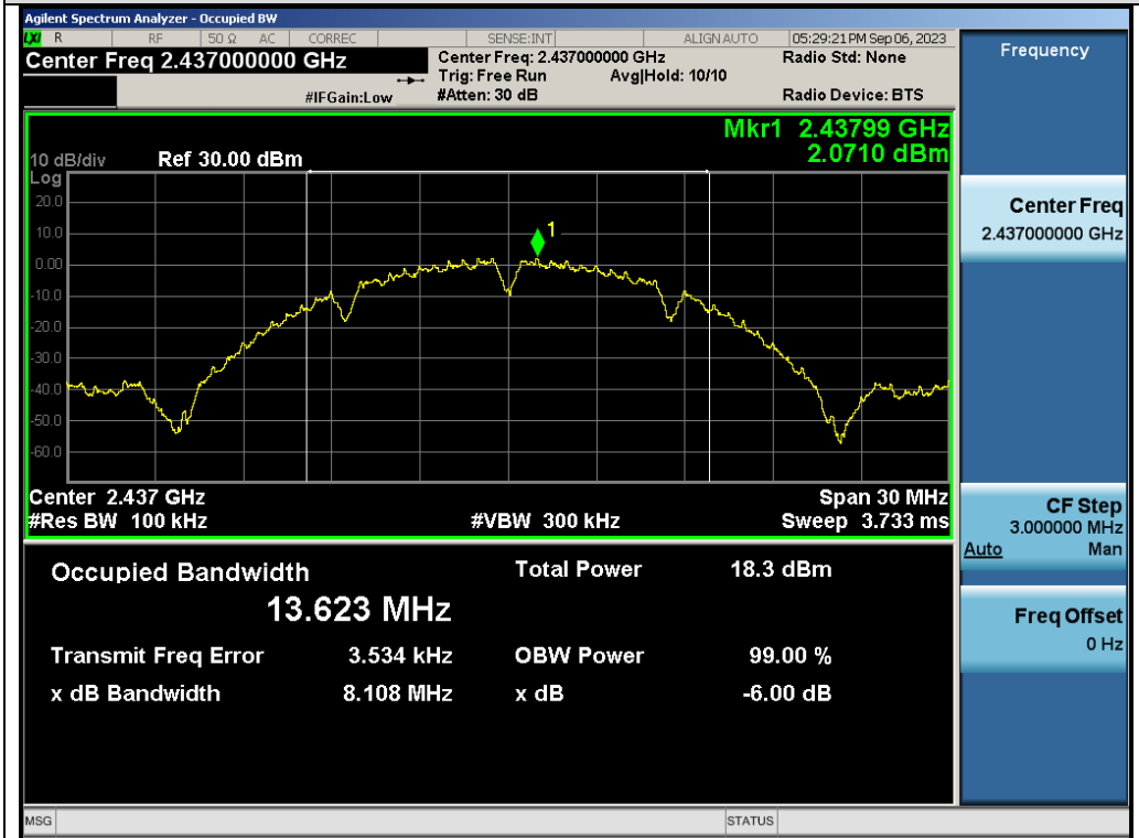
Test_Graph_802.11b_ANT1_2437_1Mbps_DTBSW
