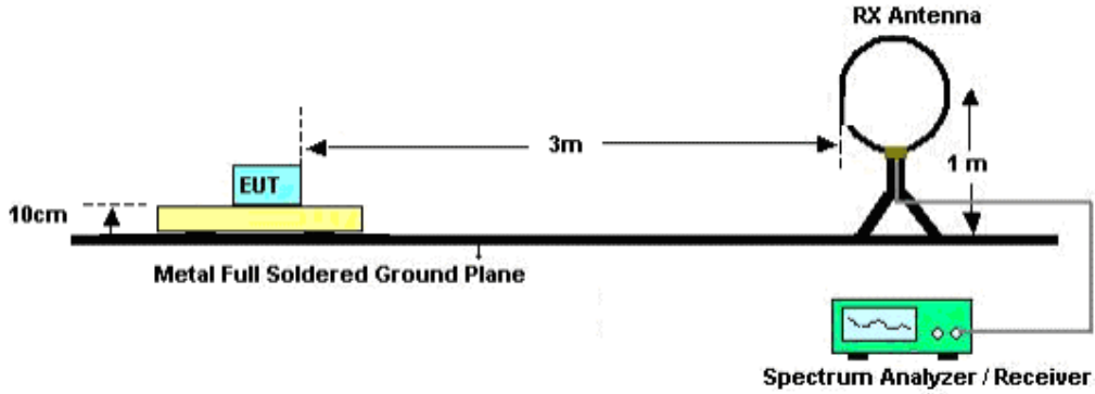
Radiated Emission Test Setup 30MHz-1000MHz
