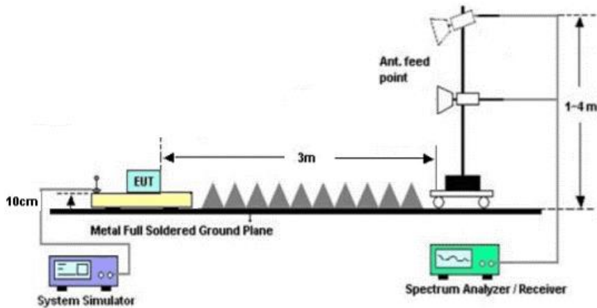
Radiated Emission Test Setup Above 1000MHz
