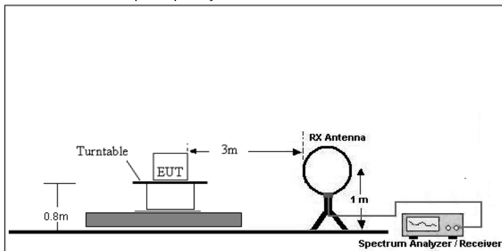
(A) Radiated Emission Test-Up Frequency Below 30MHz
