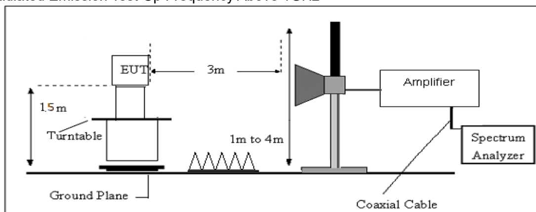
(C) Radiated Emission Test-Up Frequency Above 1GHz
