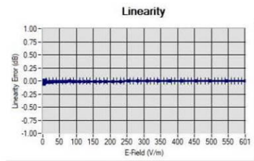
Linearity: \pm 1.48\% ( \pm 0.06 dB)
