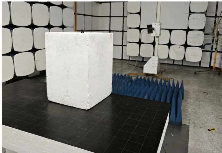
Radiated emission above 1GHz
