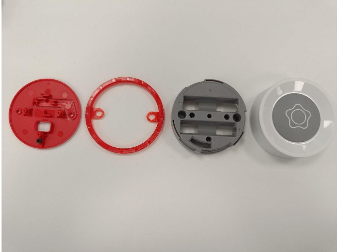
Figure 2 SPB Internal Parts - 1
