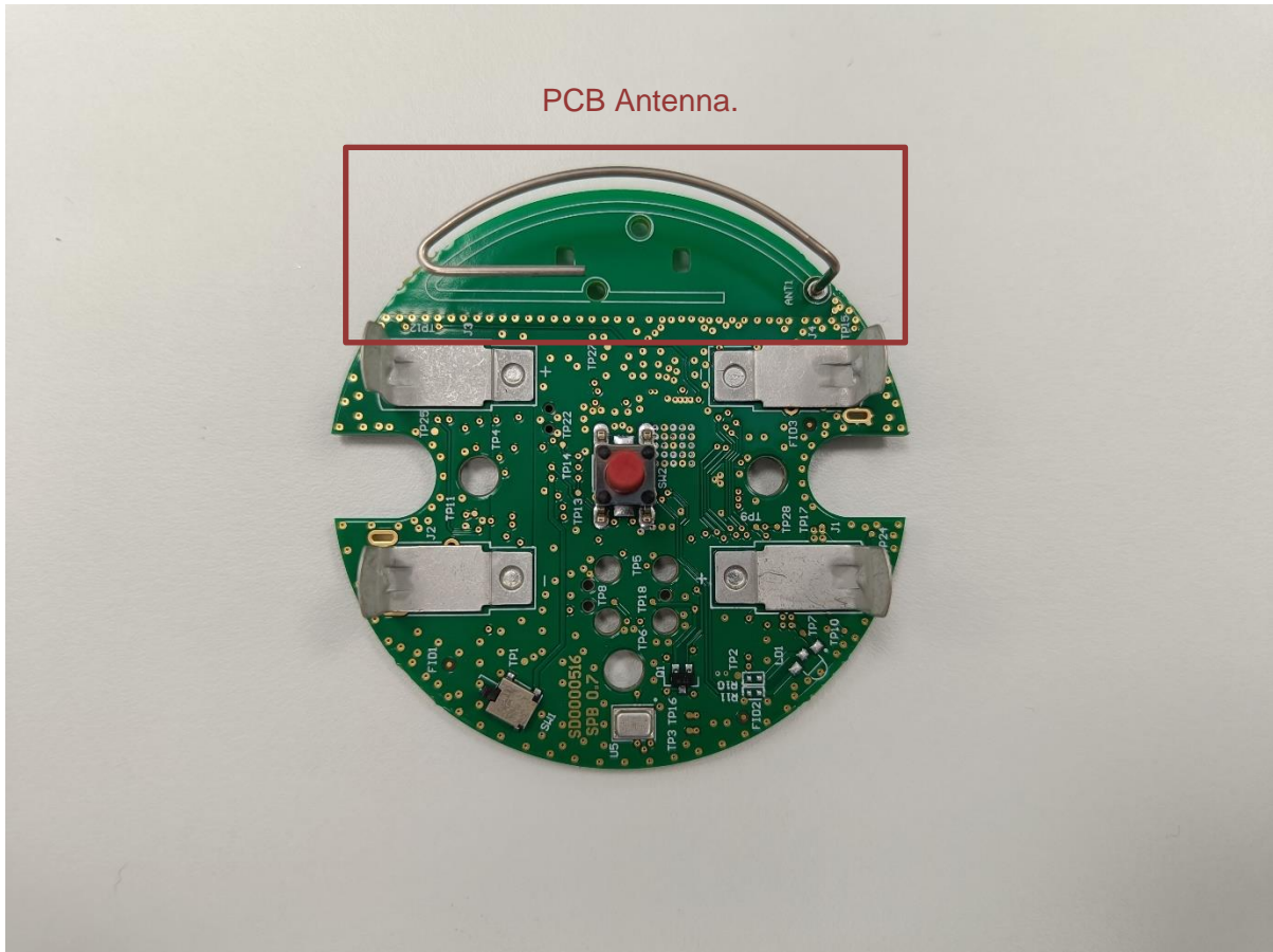
Figure 4 SPB PCB top
