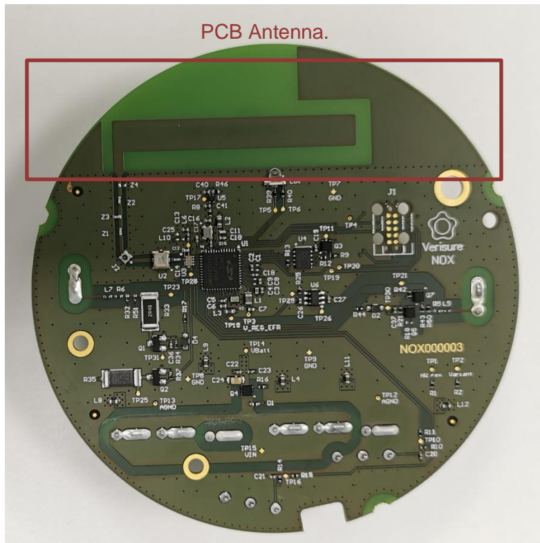
Figure 4 NOX PCB top
