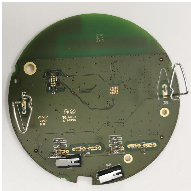
Figure 5 NOX PCB bottom
