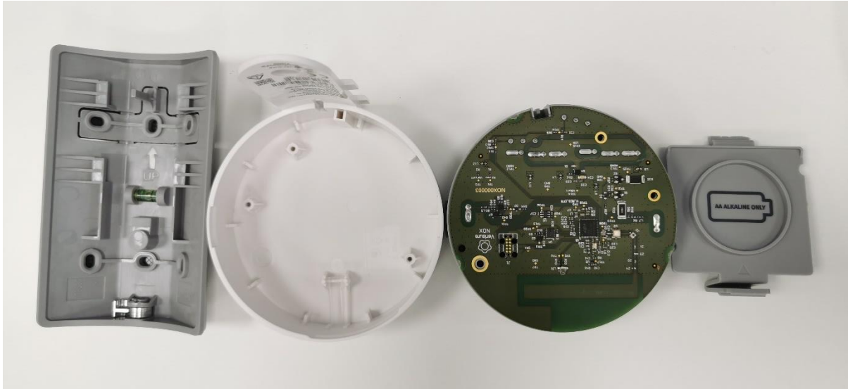
Figure 2 NOX electronic Internal Parts – 1
