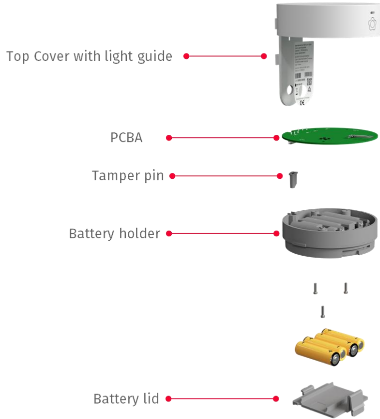
Figure 3 NOX electronic module
