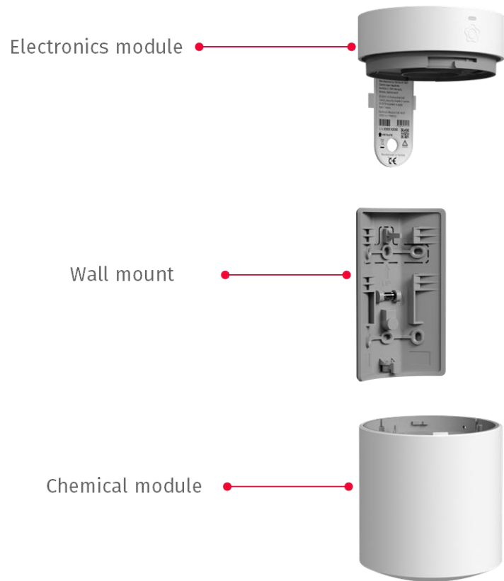
Figure 2 NOX part assembly
