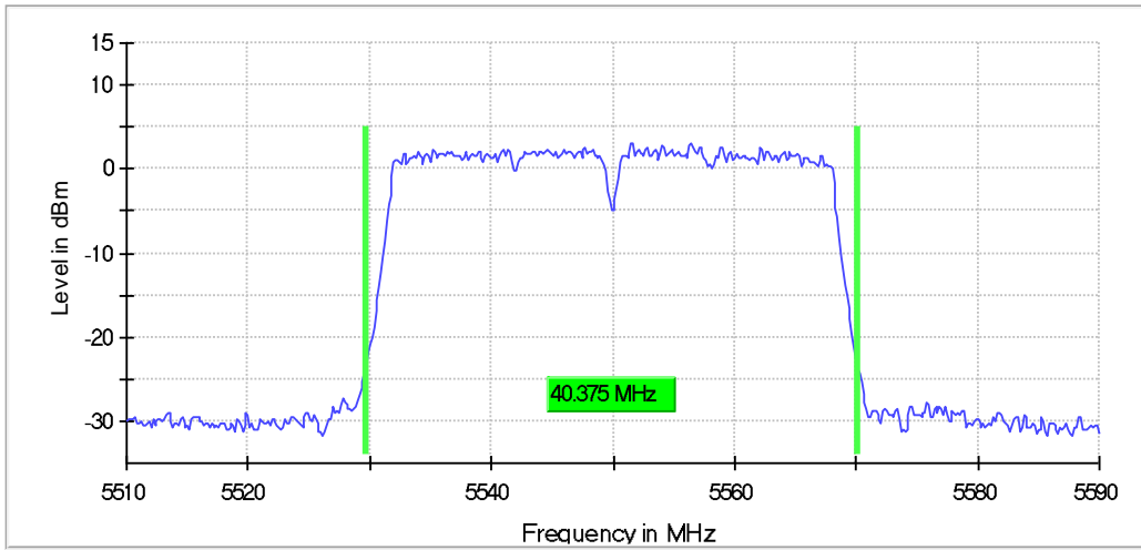
26dB Bandwidth
