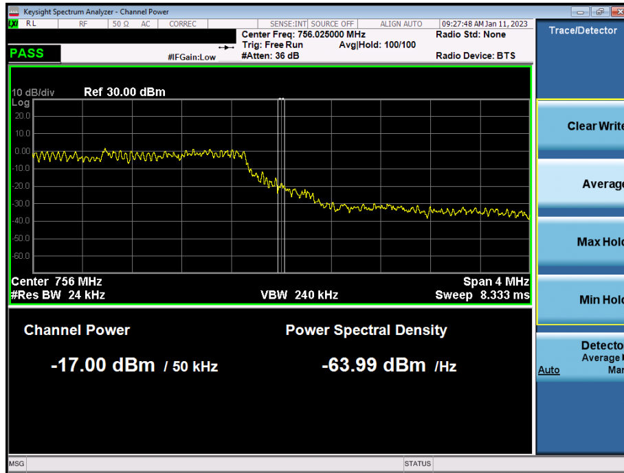
Plot 7-48. Upper Band Edge Plot (LTE Band 13- 5MHz QPSK – Full RB)
