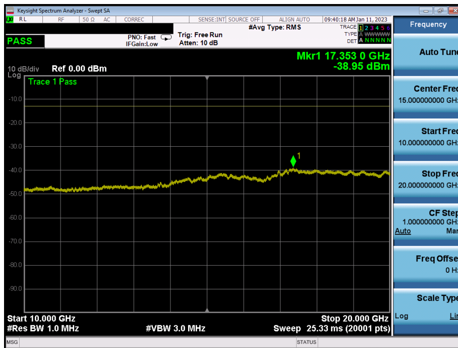
Plot 7-18. Conducted Spurious Plot (LTE Band 66 - 5MHz - Full RB - Mid Channel)
