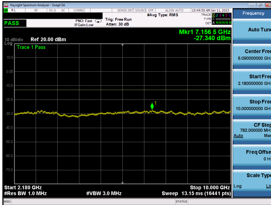
Plot 7-17. Conducted Spurious Plot (LTE Band 66 - 5MHz - Full RB - Mid Channel)
