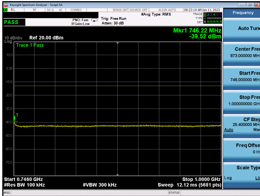
Plot 7-26. Conducted Spurious Plot (LTE Band 12 - 5MHz - Full RB - Mid Channel)
