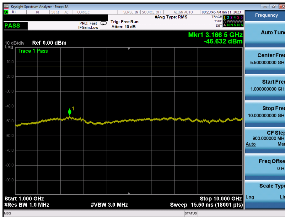
Plot 7-27. Conducted Spurious Plot (LTE Band 12 - 5MHz - Full RB - Mid Channel)
