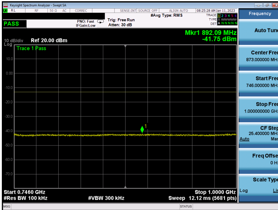
Plot 7-23. Conducted Spurious Plot (LTE Band 12 - 5MHz - Full RB - Low Channel)
