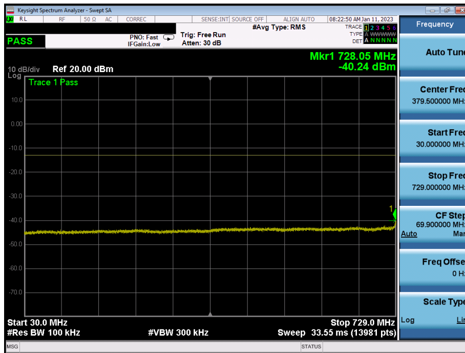
Plot 7-25. Conducted Spurious Plot (LTE Band 12 - 5MHz - Full RB - Mid Channel)
