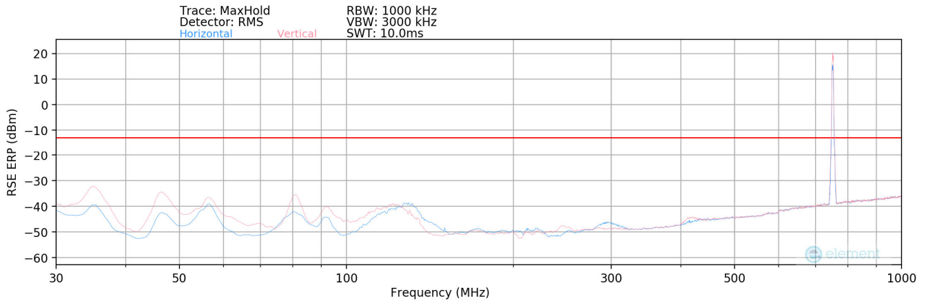
Plot 7-57. Radiated Spurious Plot (LTE Band 13- LTE Band 2)- Below 1GHz
