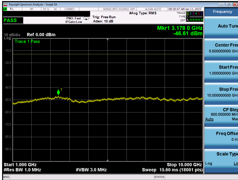
Plot 7-30. Conducted Spurious Plot (LTE Band 12 - 5MHz - Full RB - High Channel)
