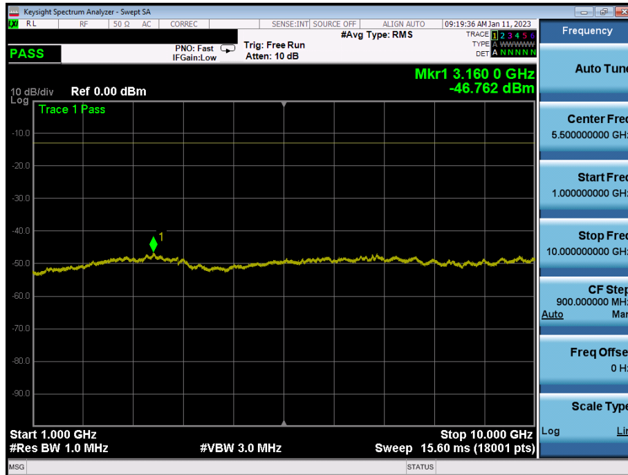
Plot 7-39. Conducted Spurious Plot (LTE Band 13 - 5MHz - Full RB - High Channel)
