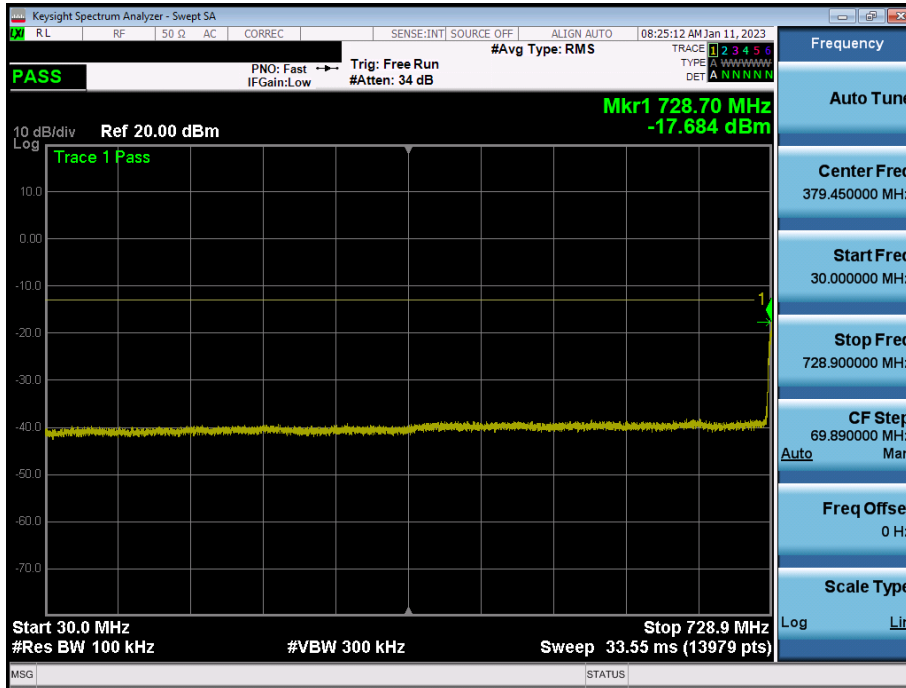
Plot 7-22. Conducted Spurious Plot (LTE Band 12 - 5MHz - Full RB - Low Channel)
