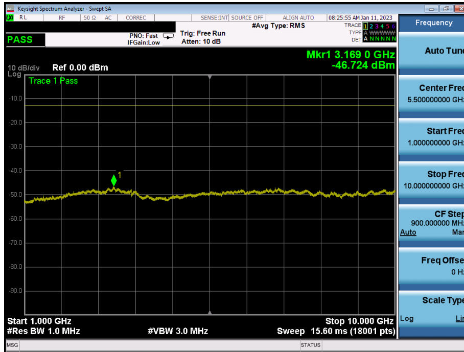
Plot 7-24. Conducted Spurious Plot (LTE Band 12 - 5MHz - Full RB - Low Channel)
