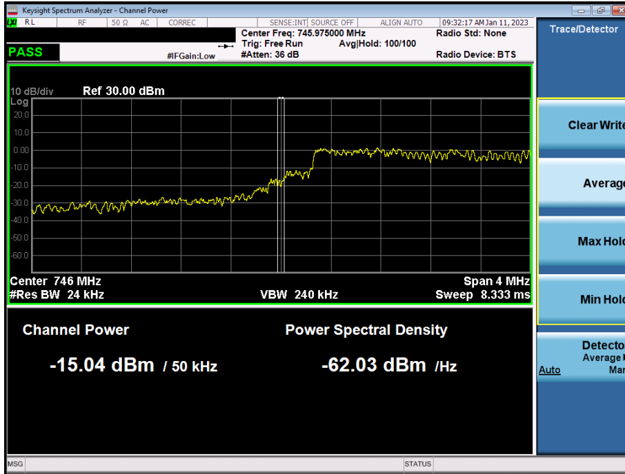
Plot 7-46. Lower Band Edge Plot (LTE Band 13- 5MHz QPSK – Full RB)
