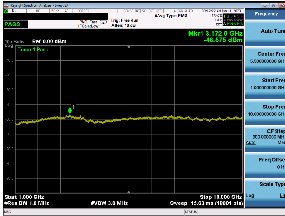
Plot 7-33. Conducted Spurious Plot (LTE Band 13 - 5MHz - Full RB - Low Channel)
