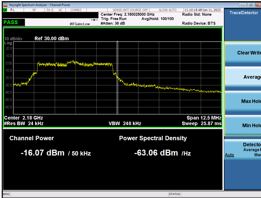
Plot 7-42. Upper Band Edge Plot (LTE Band 66- 5MHz QPSK – Full RB)
