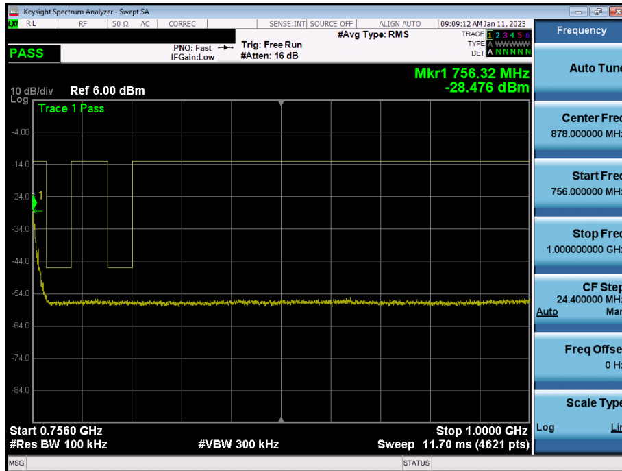
Plot 7-35. Conducted Spurious Plot (LTE Band 13 - 5MHz - Full RB - Mid Channel)
