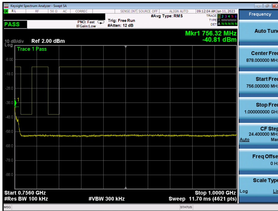
Plot 7-32. Conducted Spurious Plot (LTE Band 13 - 5MHz - Full RB - Low Channel)
