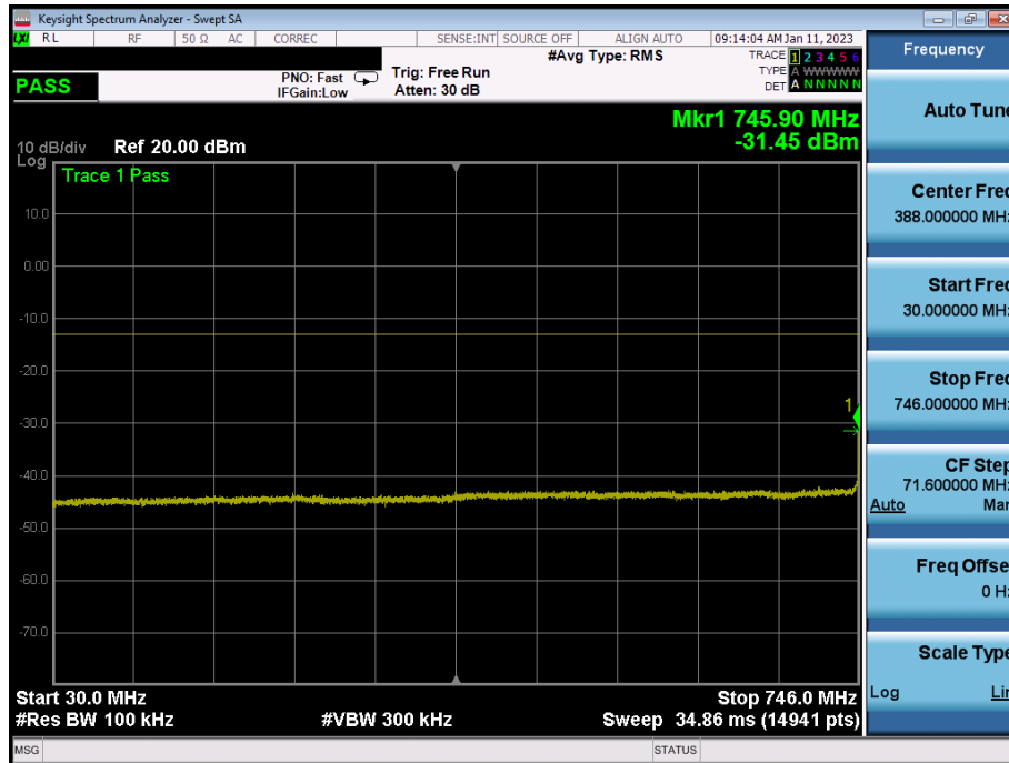
Plot 7-37. Conducted Spurious Plot (LTE Band 13 - 5MHz - Full RB - High Channel)
