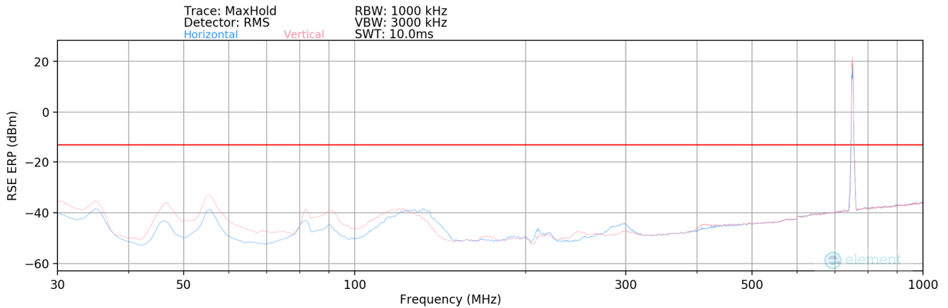
Plot 7-53. Radiated Spurious Plot (LTE Band 66- LTE Band 13)- Below 1GHz
