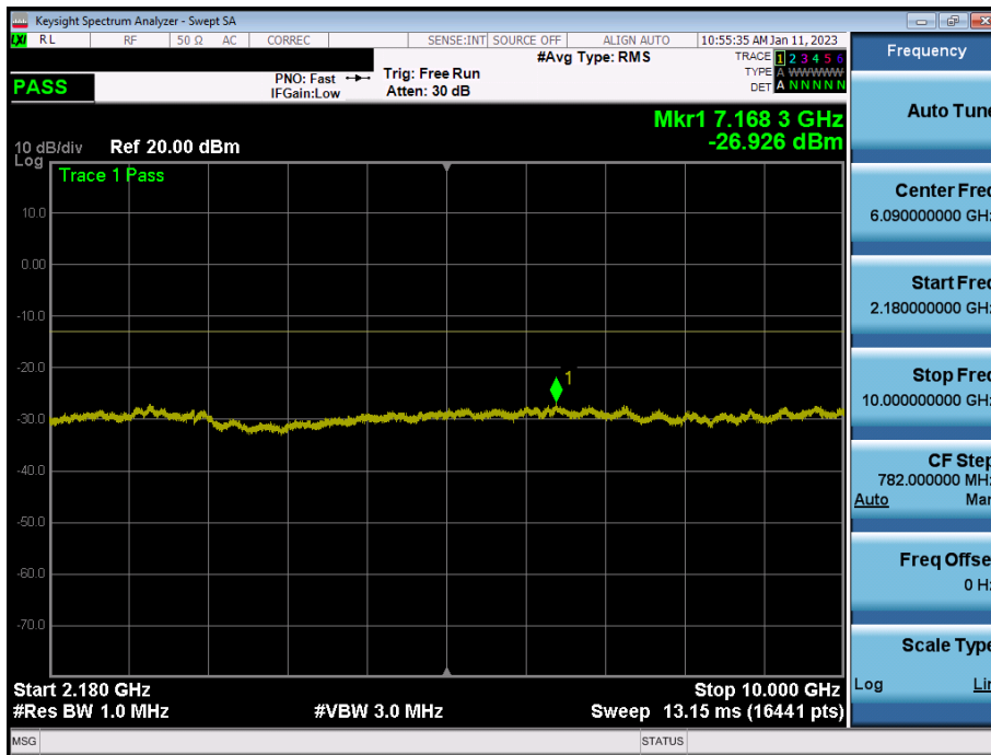
Plot 7-14. Conducted Spurious Plot (LTE Band 66 - 5MHz - Full RB - Low Channel)
