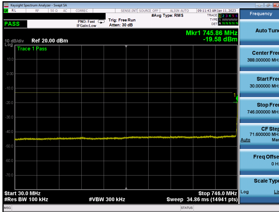
Plot 7-31. Conducted Spurious Plot (LTE Band 13 - 5MHz - Full RB - Low Channel)
