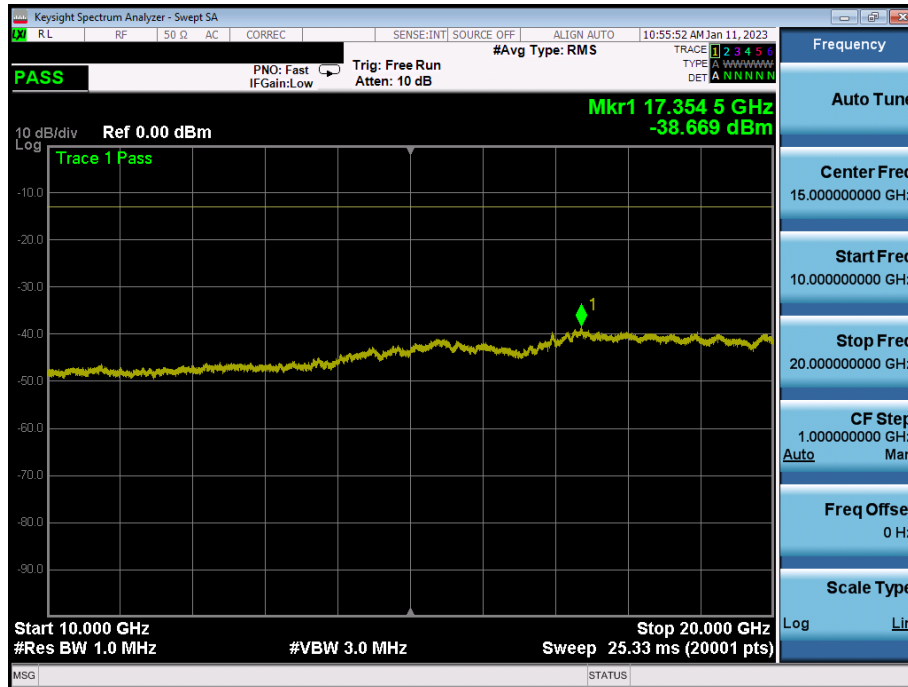
Plot 7-15. Conducted Spurious Plot (LTE Band 66 - 5MHz - Full RB - Low Channel)
