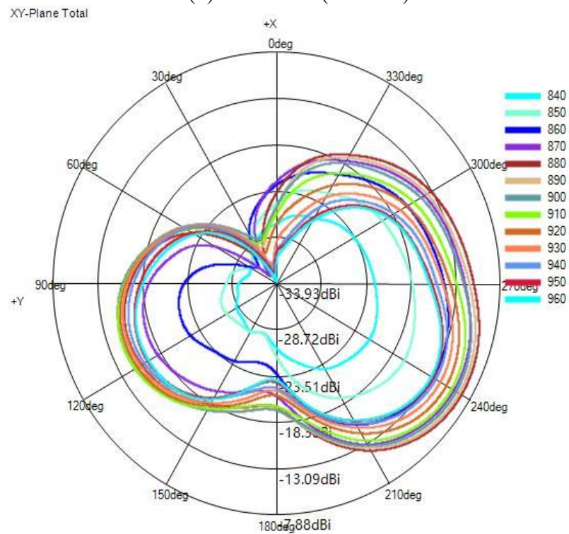
(3) X-Y Plane(unit:dBi):
