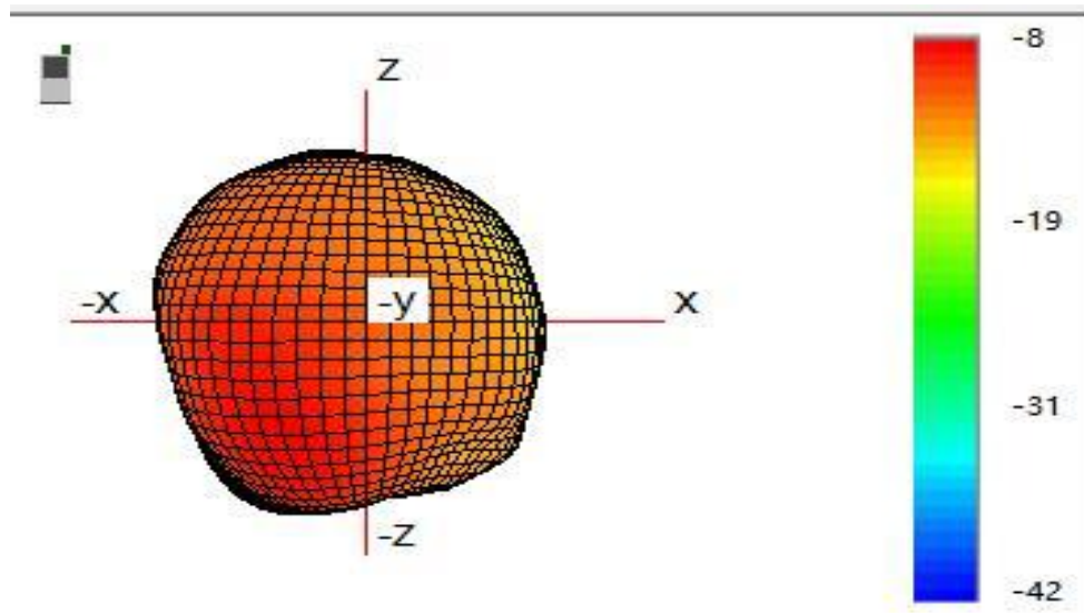
(4) Typical Free Space 3D Radiation Pattern at 880MHz(unit:dBi):
