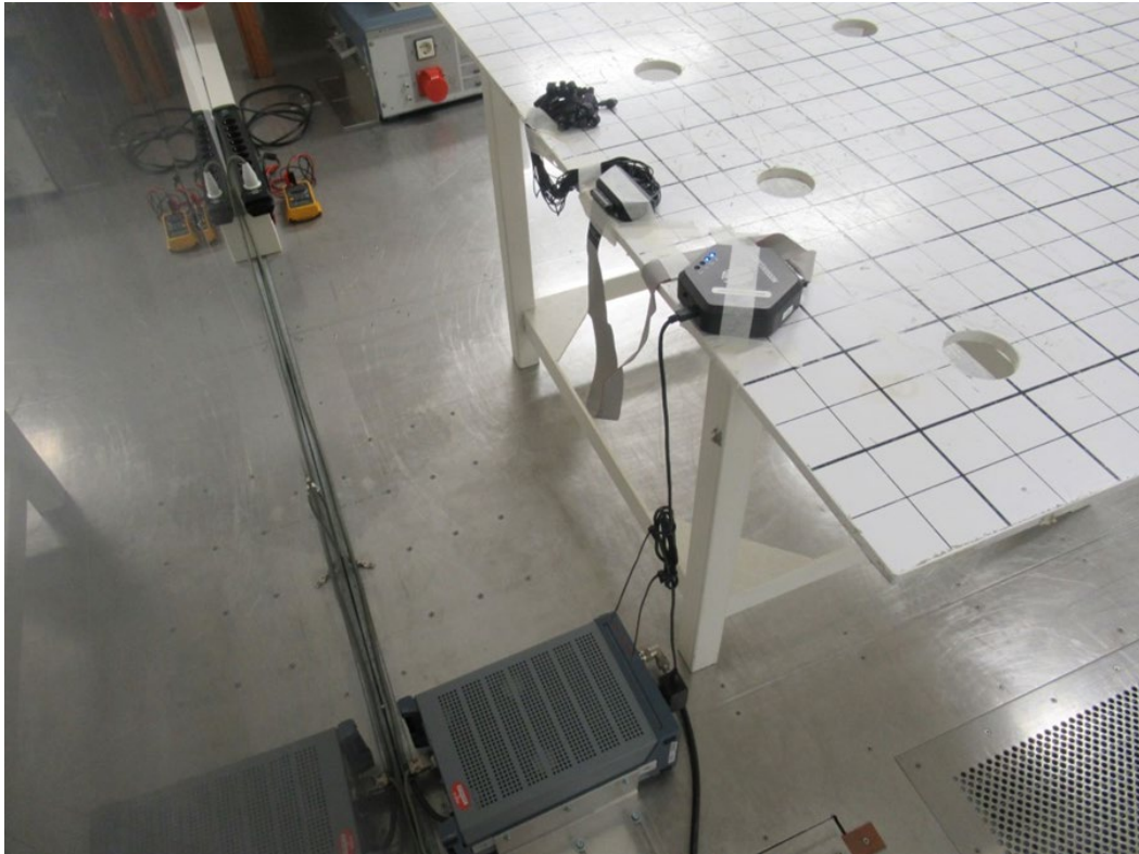
Photo 1: Conducted Test Setup from 150 kHz to 30 MHz
