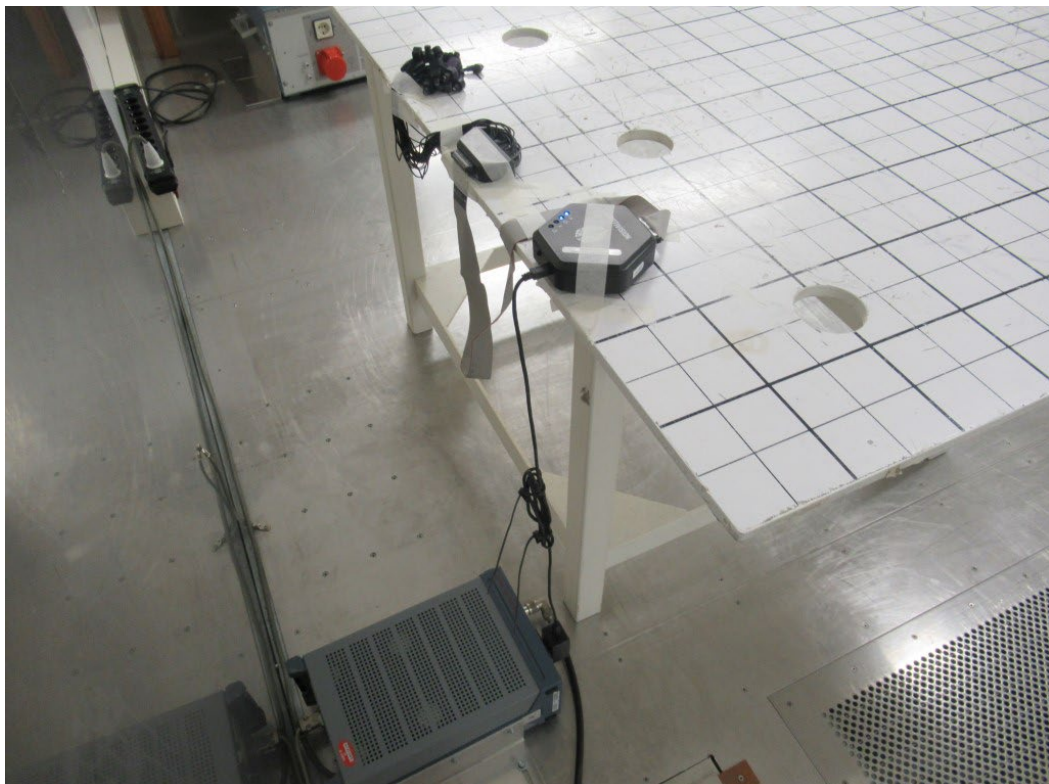
Photo 2: Conducted Test Setup from 150 kHz to 30 MHz
