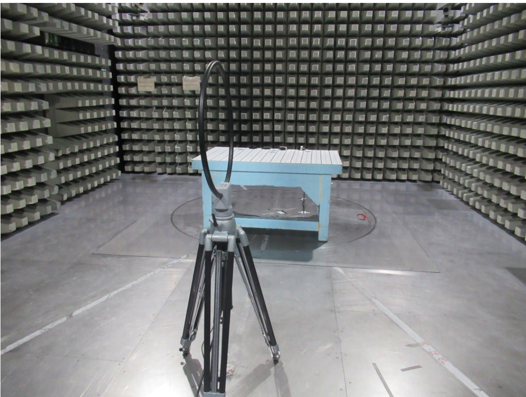
Photo 4: Radiated Test Setup from 9 kHz to 30 MHz
