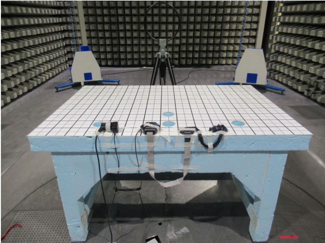
Photo 3: Radiated Test Setup from 9 kHz to 30 MHz
