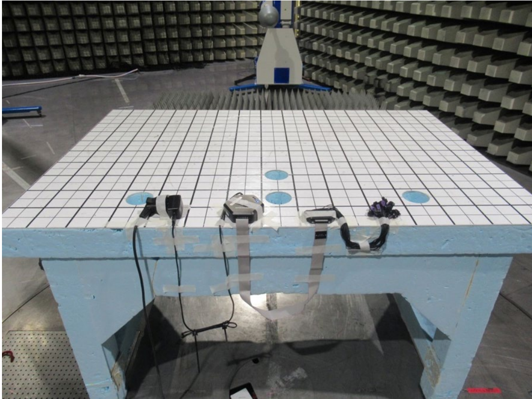
Photo 7: Radiated Test Setup from 1 GHz to 15 GHz
