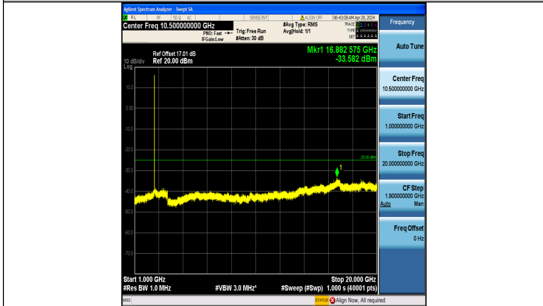
Band7_10MHz_QPSK_21400_50RB#0_1000~20000_1000~20000
