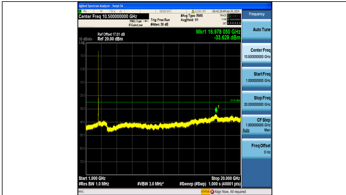
Band7_10MHz_16QAM_21100_50RB#0_1000~20000_1000~20000
