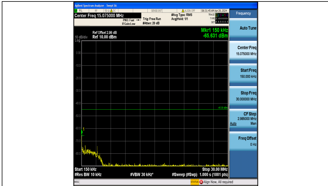
Band7_5MHz_16QAM_21100_25RB#0_0.15~30_0.15~30
