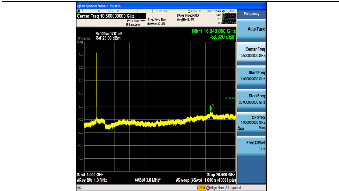
Band7_15MHz_16QAM_21100_75RB#0_1000~20000_1000~20000
