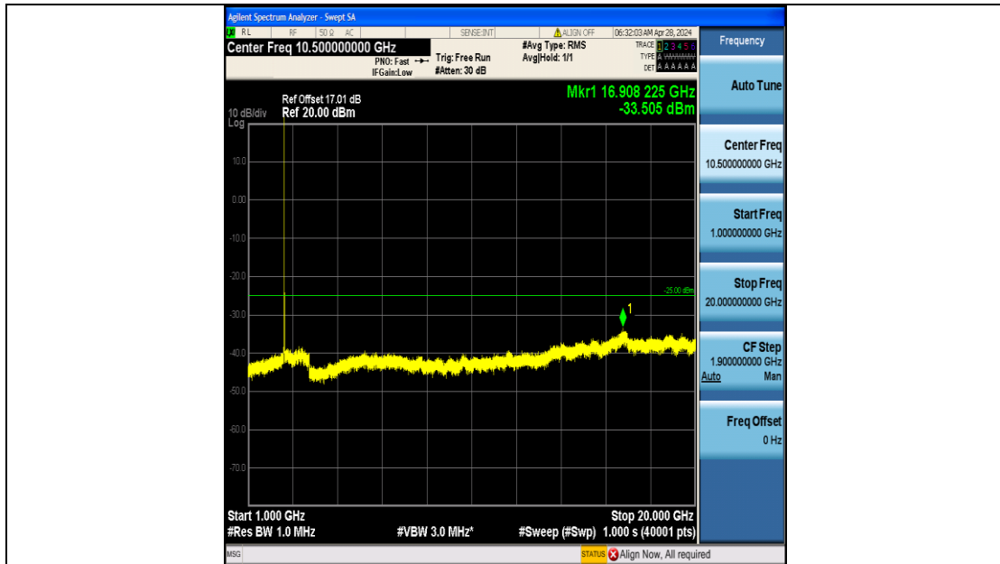
Band7_5MHz_16QAM_21100_25RB#0_1000~20000_1000~20000
