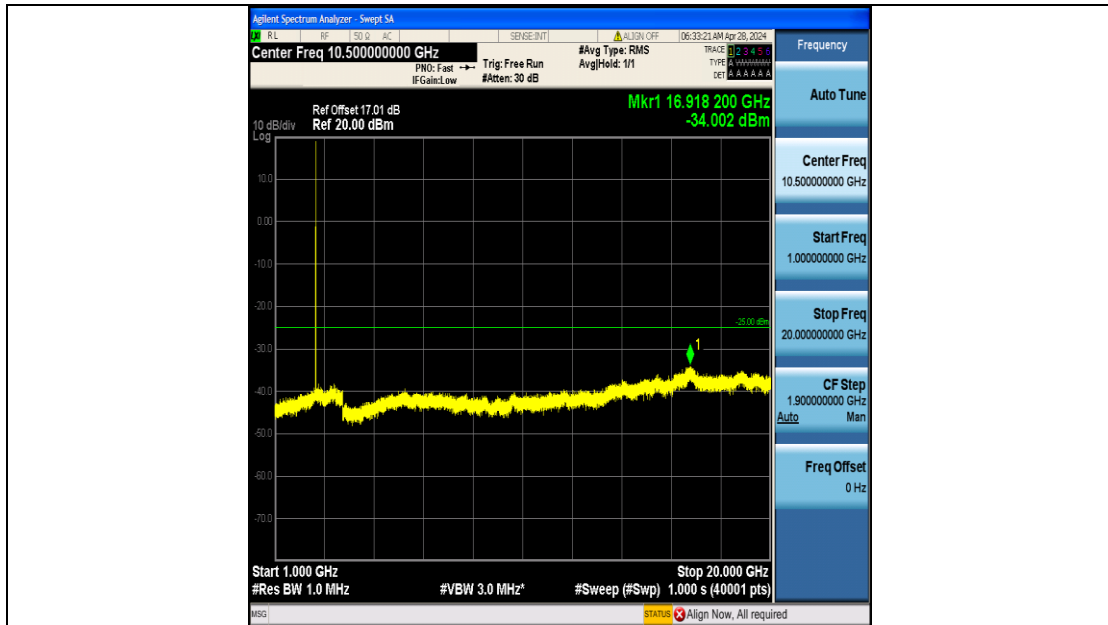
Band7_5MHz_16QAM_21425_25RB#0_1000~20000_1000~20000
