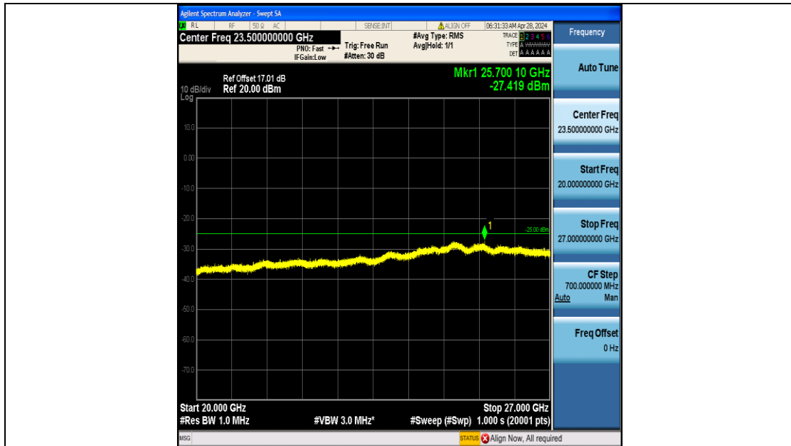
Band7_5MHz_QPSK_21100_25RB#0_20000~27000_20000~27000
