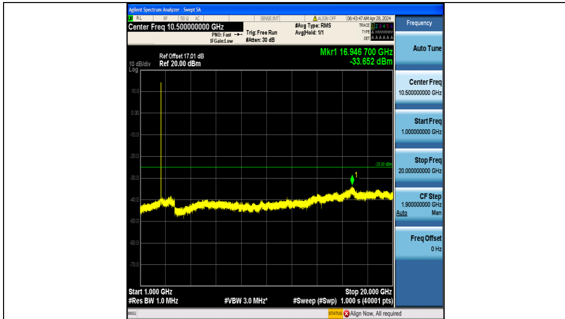
Band7_10MHz_16QAM_21400_50RB#0_1000~20000_1000~20000
