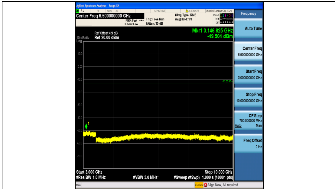
Band5_1.4MHz_QPSK_20525_6RB#0_3000~10000_3000~10000
