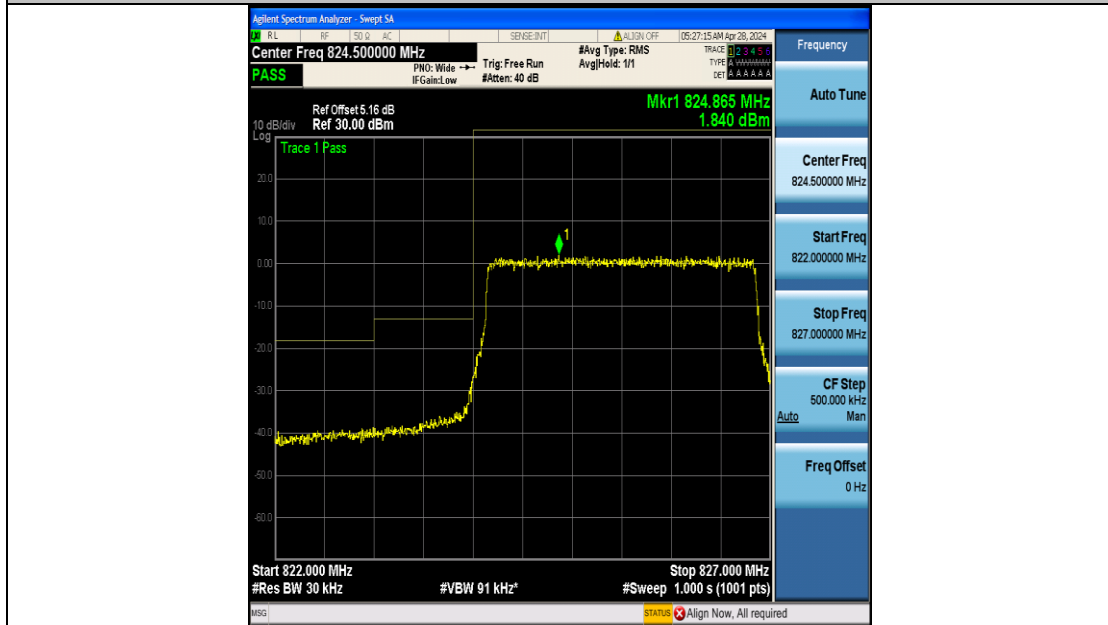
Band5_3MHz_QPSK_20415_15RB#0
