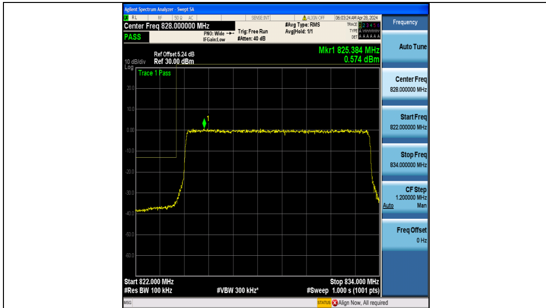
Band5_10MHz_16QAM_20450_50RB#0
