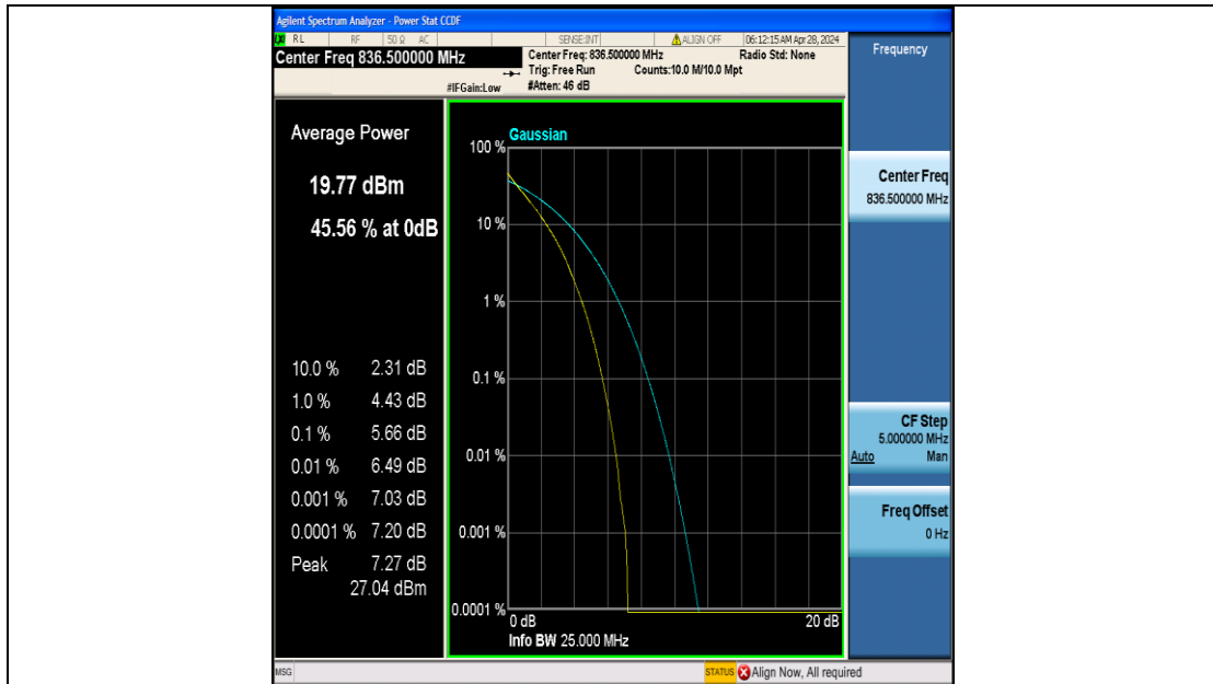
Band5-10MHz-QPSK-20525-50RB#0-PASS
