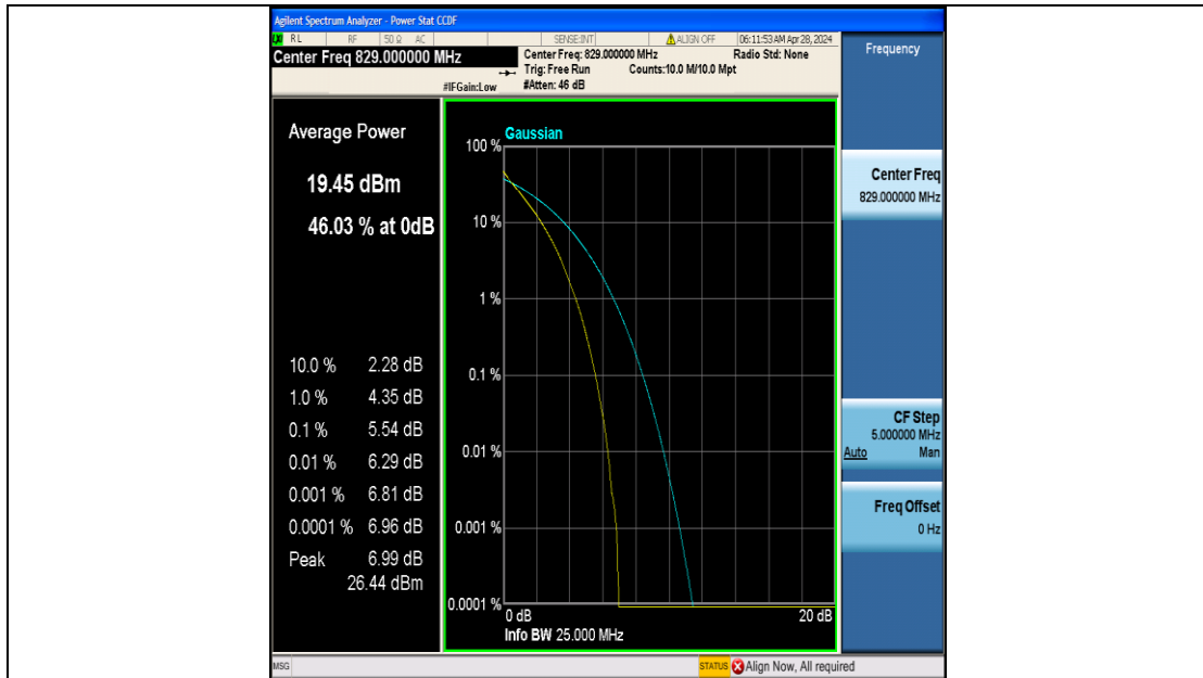
Band5-10MHz-QPSK-20450-50RB#0-PASS
