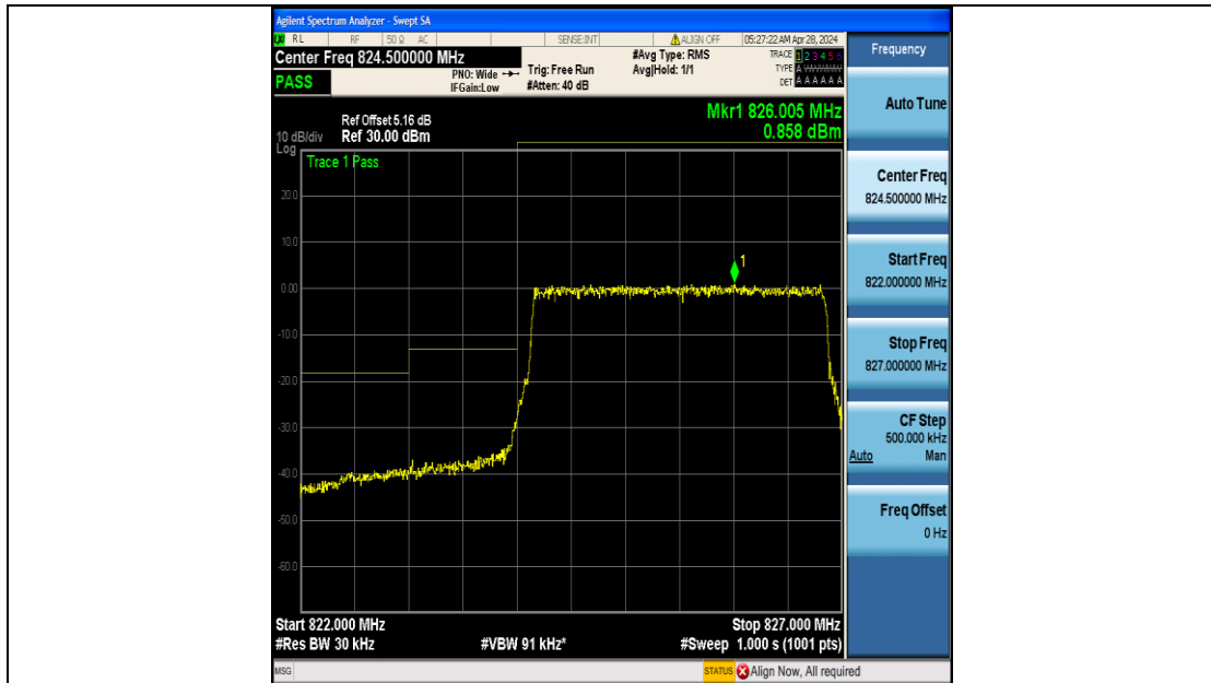
Band5_3MHz_16QAM_20415_15RB#0
