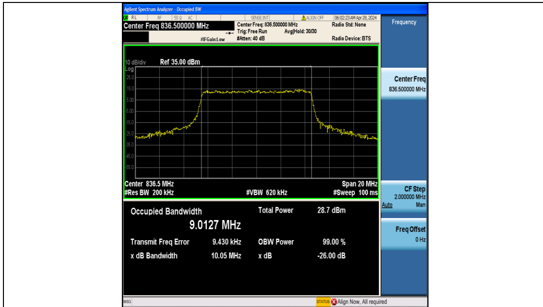
Band5-10MHz-QPSK-20525-50RB#0-PASS
