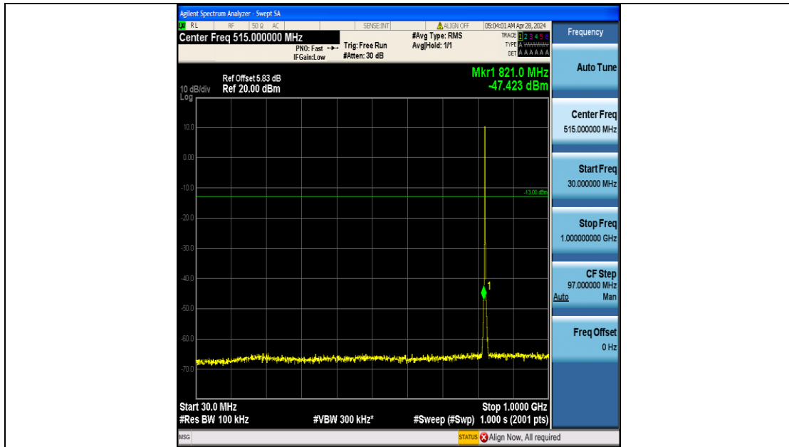
Band5_1.4MHz_QPSK_20407_6RB#0_30~1000_30~1000
