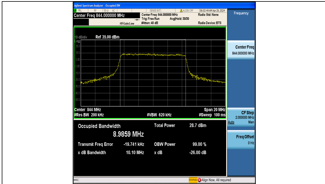
Band5-10MHz-QPSK-20600-50RB#0-PASS
