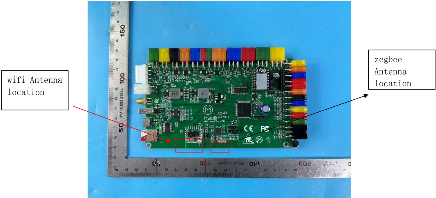
INTERNAL PHOTO OF SAMPLE PCB
