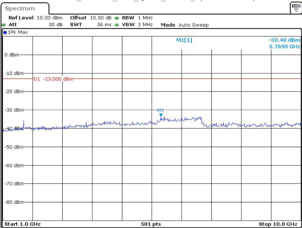
Band 26_1.4 MHz_Low_QPSK_RB1#0_2(1GHz-10GHz)
