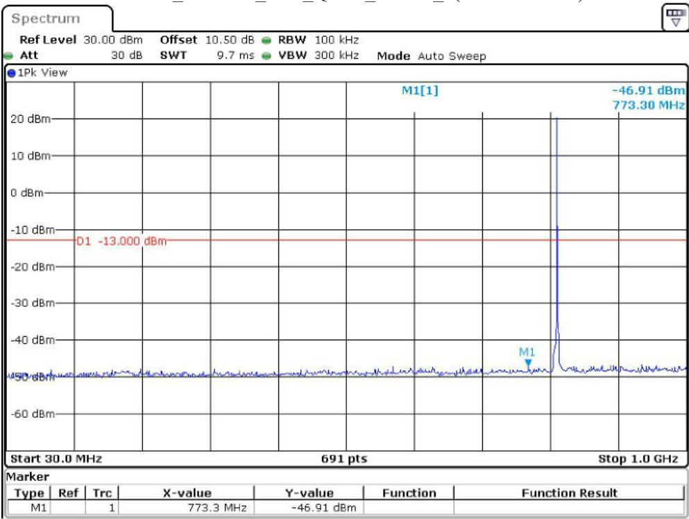
Band 26_1.4 MHz_Low_QPSK_RB1#0_1(30MHz-1GHz)
