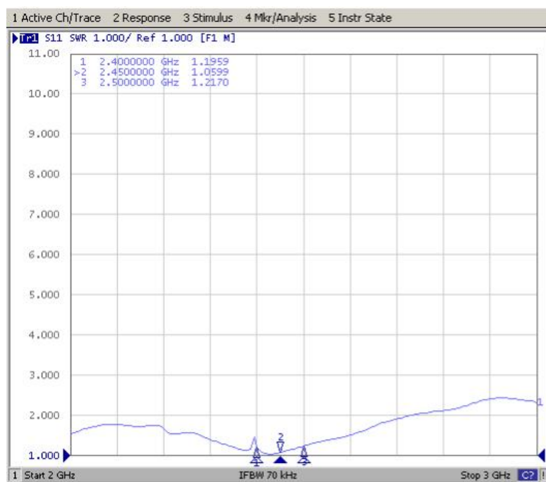
SWR
