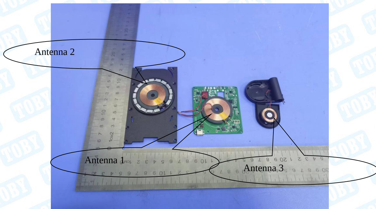
Photo 12 Appearance of PCB
