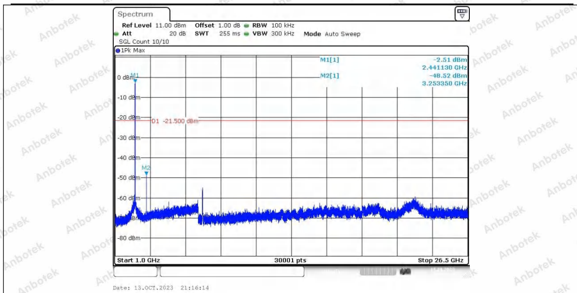
20M_Ant2_2440_0~Reference
