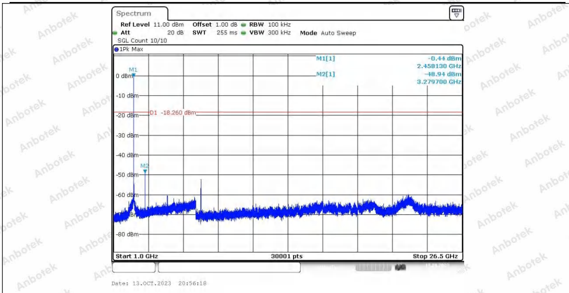
10M_Ant2_2460_0~Reference
