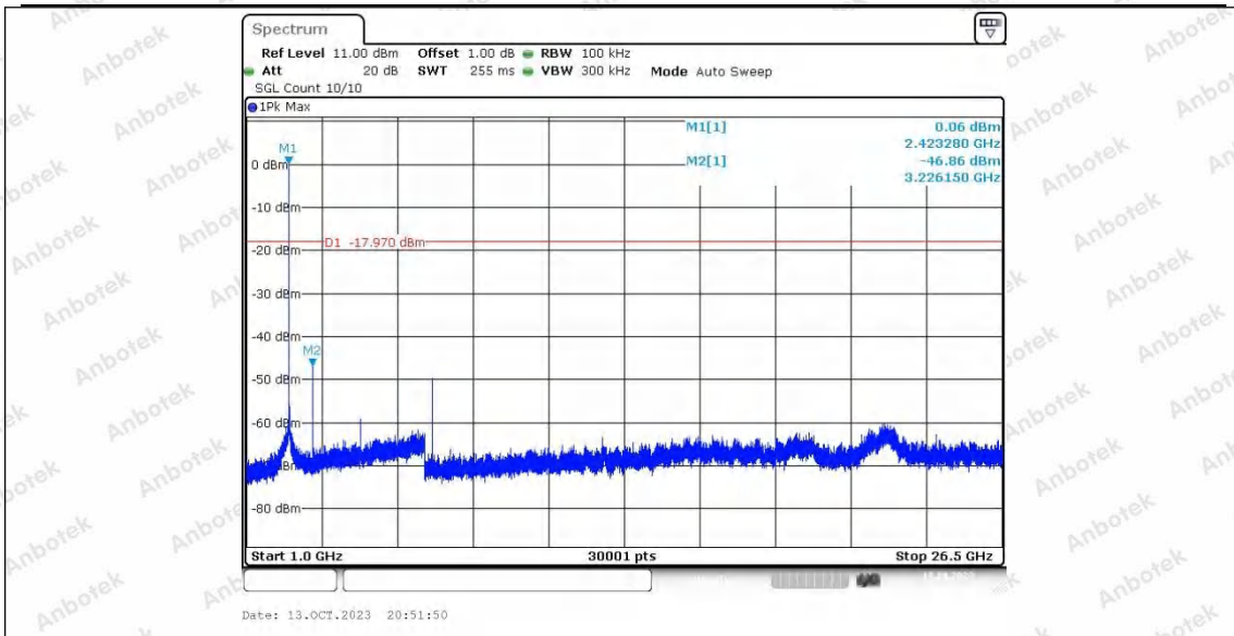
10M_Ant2_2420_0~Reference
