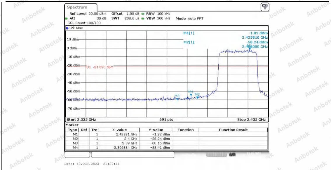
20M_Ant2_Low_2420
