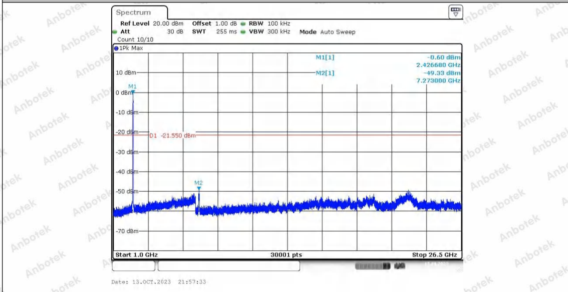
40M_Ant1_2440_0~Reference
