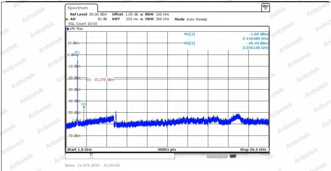
40M_Ant2_2420_0~Reference
