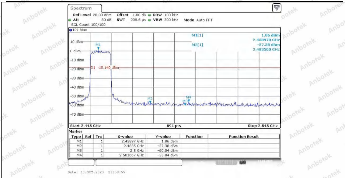
10M_Ant2_High_2460
