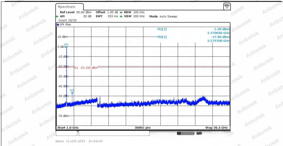
40M_Ant2_2460_0~Reference
