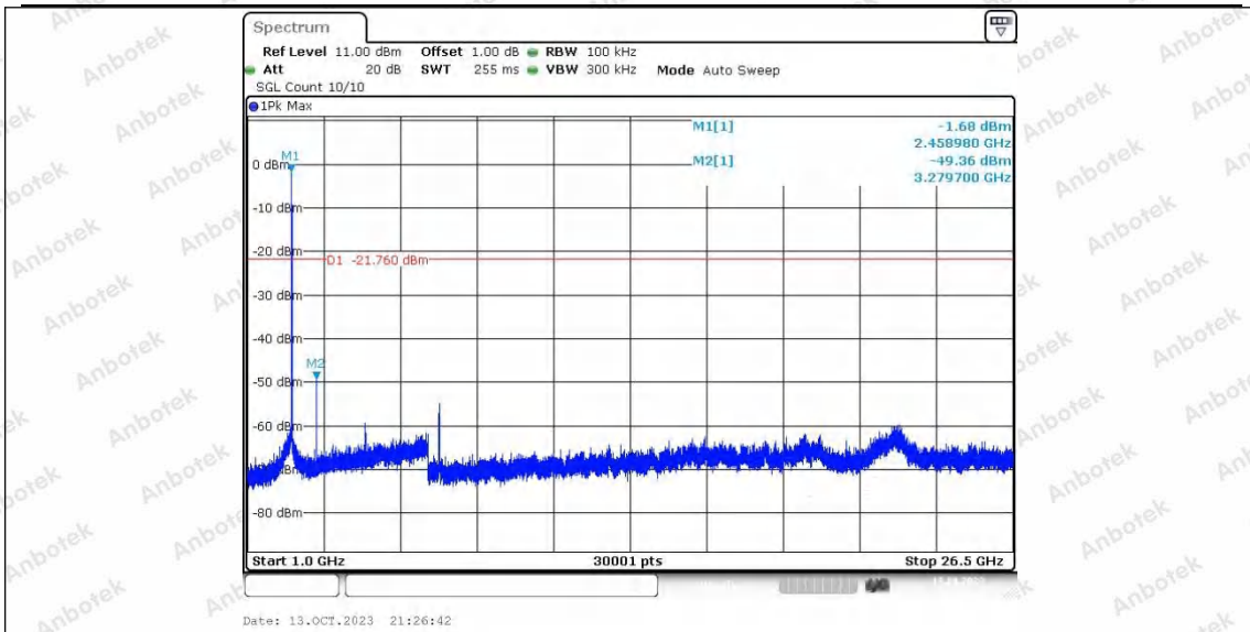
20M_Ant2_2460_0~Reference
