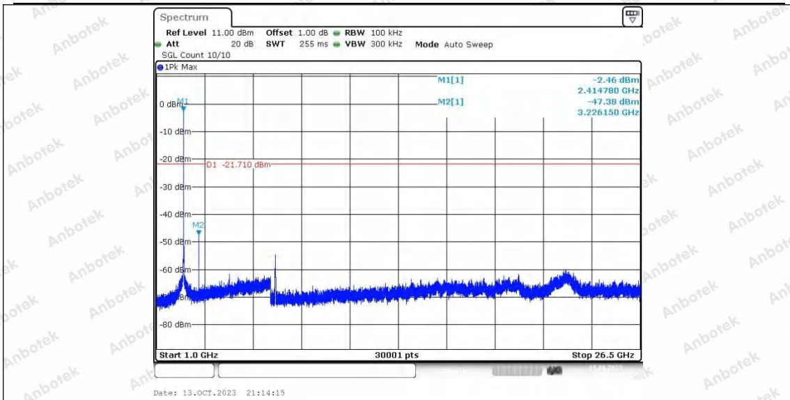
20M_Ant2_2420_0~Reference
