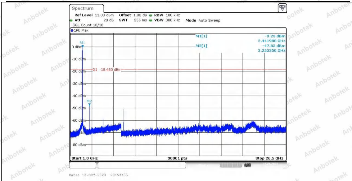
10M_Ant2_2440_0~Reference
