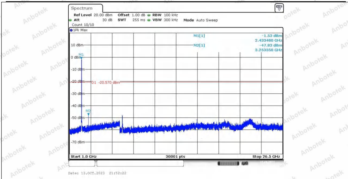
40M_Ant2_2440_0~Reference
