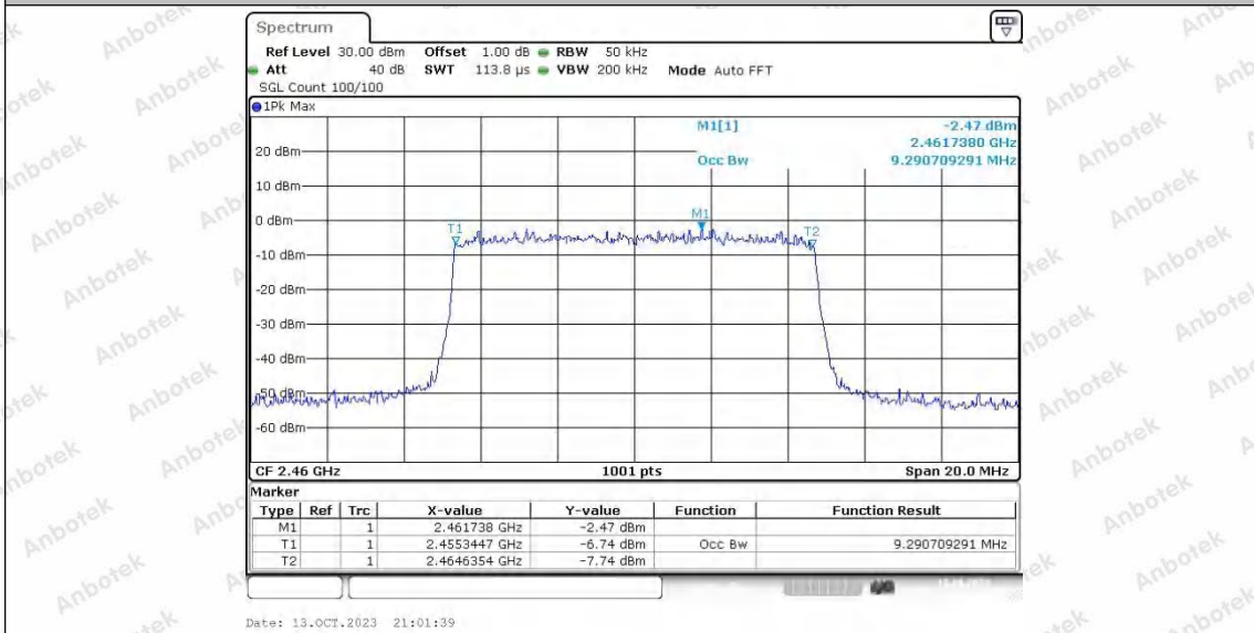
20M_Ant1_2420
