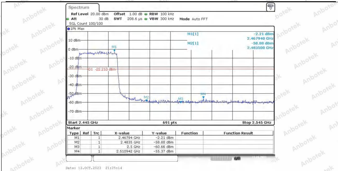
20M_Ant2_High_2460
