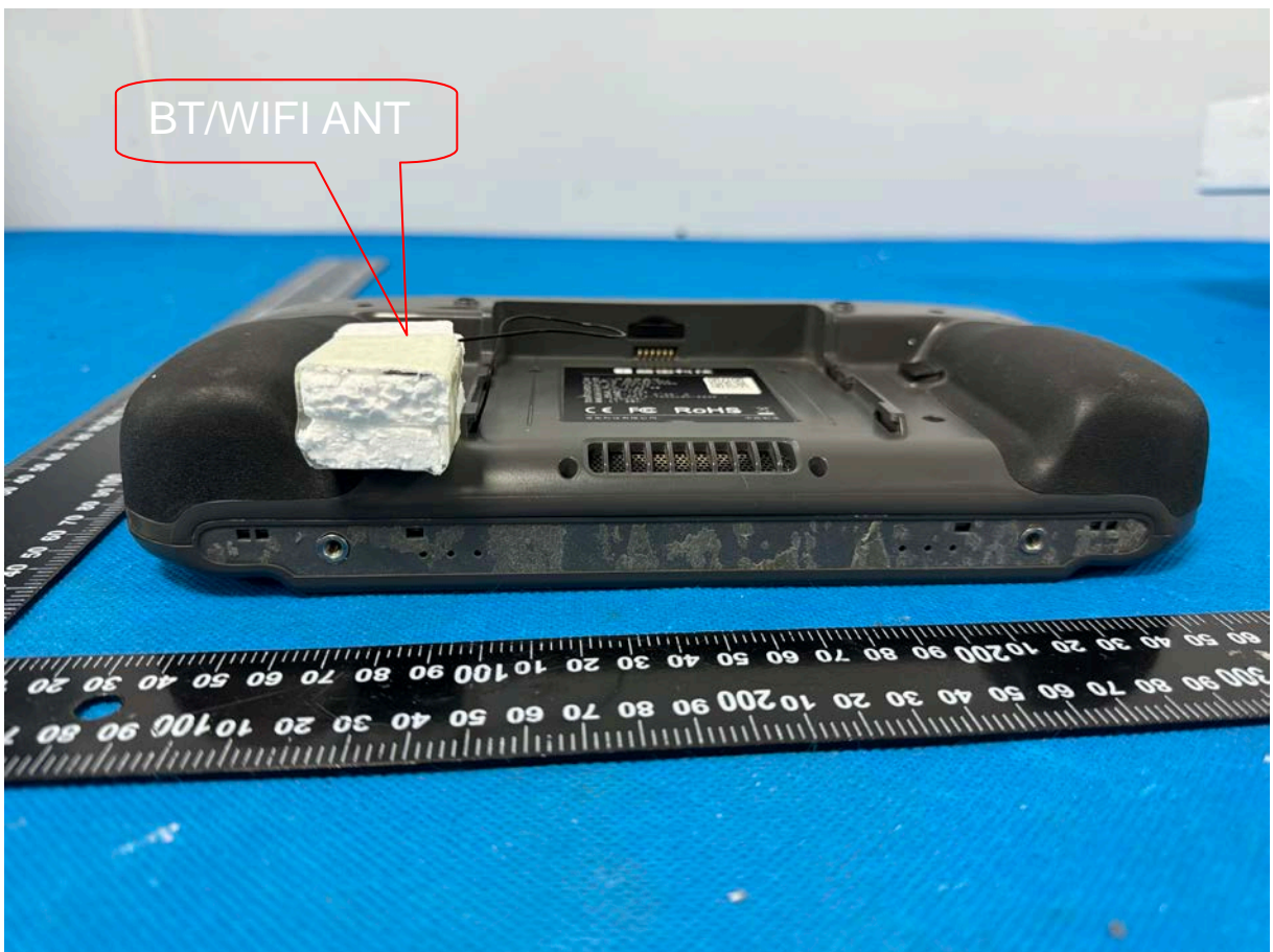
Photo 4 - WIFI / BT ANT location
