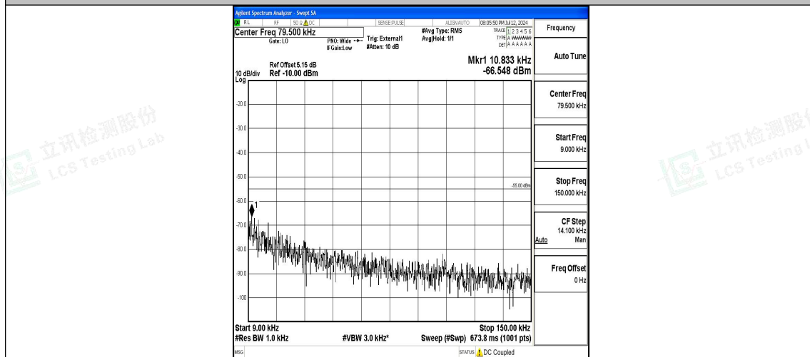
Band41_20MHz_16QAM_41490_1RB#0_0.009~0.15_0.009~0.15
