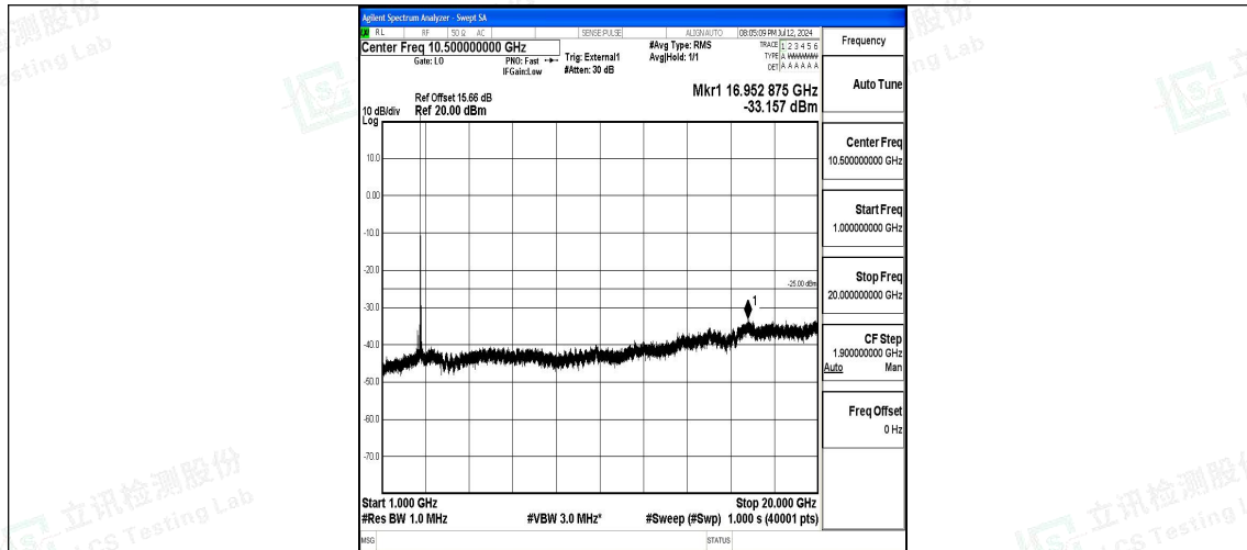
Band41_20MHz_QPSK_41490_1RB#0_1000~20000_1000~20000
