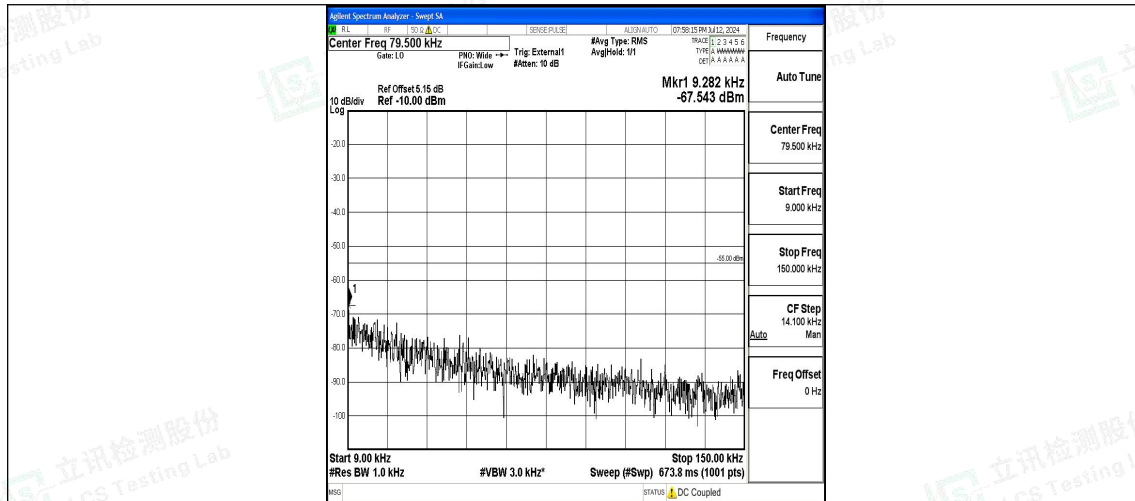
Band41_20MHz_16QAM_39750_1RB#0_0.009~0.15_0.009~0.15
