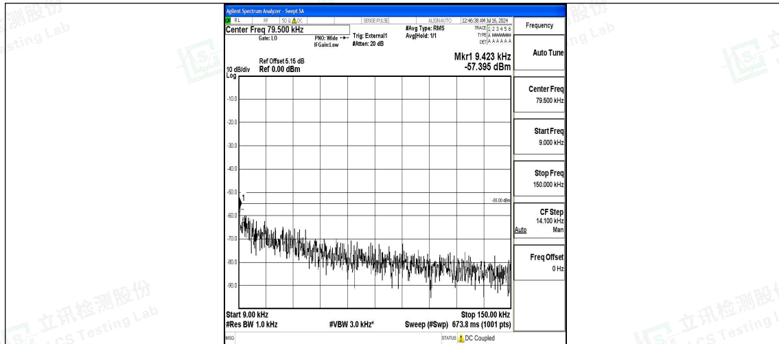
Band38_15MHz_QPSK_38175_1RB#0_0.009~0.15_0.009~0.15
