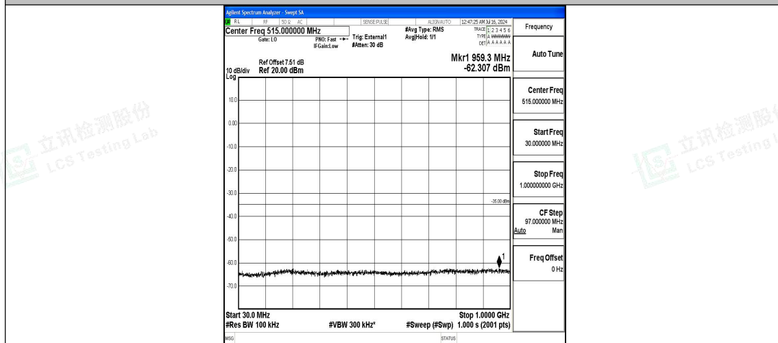
Band38_15MHz_QPSK_38175_1RB#0_30~1000_30~1000
