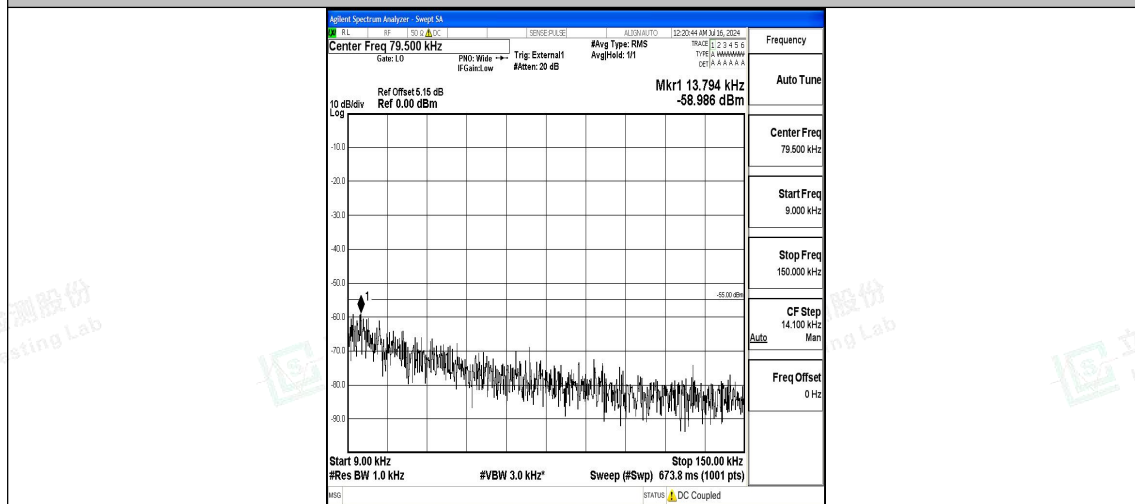
Band38_10MHz_16QAM_38000_1RB#0_0.009~0.15_0.009~0.15
