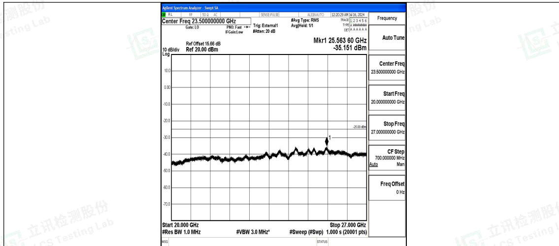
Band38_10MHz_QPSK_38000_1RB#0_20000~27000_20000~27000
