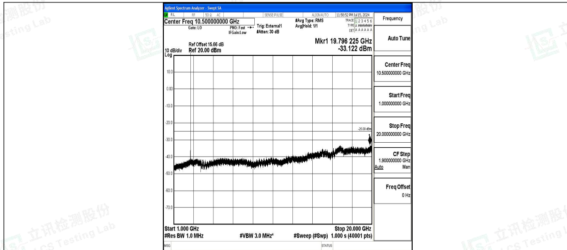
Band38_5MHz_QPSK_38225_1RB#0_1000~20000_1000~20000
