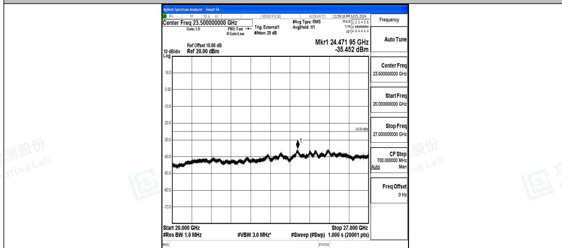
Band38_5MHz_QPSK_38225_1RB#0_20000~27000_20000~27000
