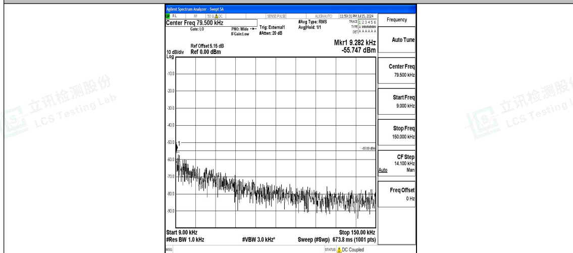
Band38_5MHz_16QAM_38225_1RB#0_0.009~0.15_0.009~0.15
