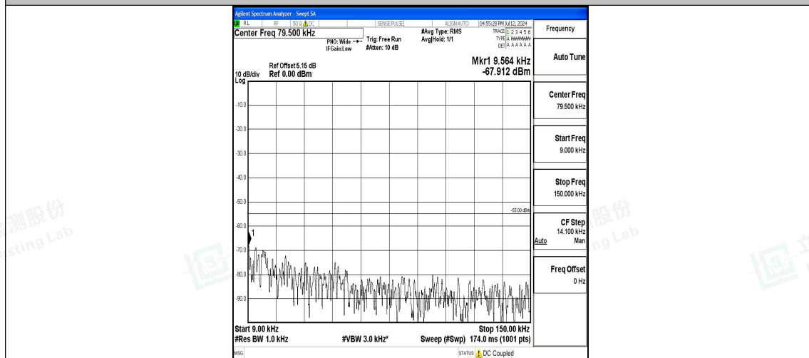
Band7_20MHz_16QAM_21100_1RB#0_0.009~0.15_0.009~0.15
