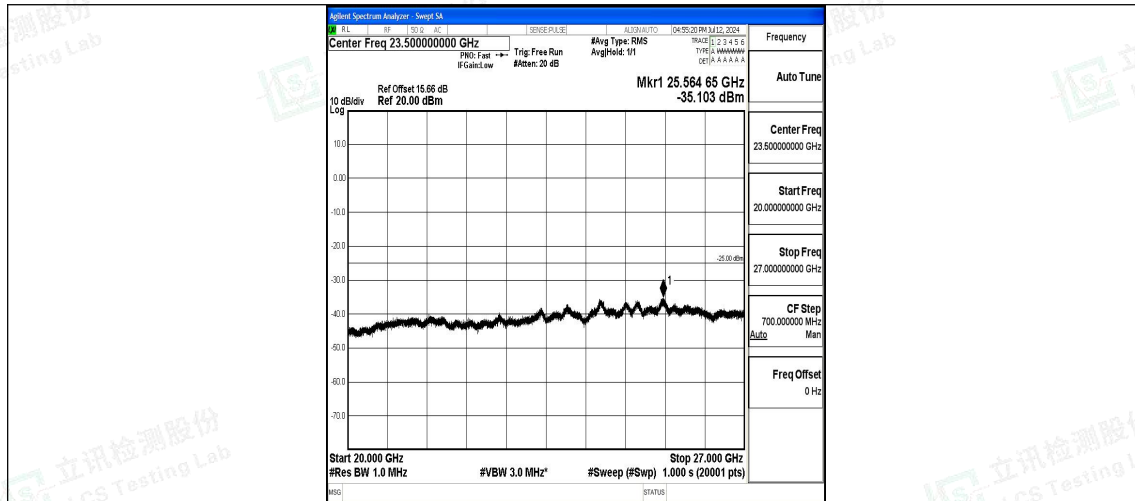
Band7_20MHz_QPSK_21100_1RB#0_20000~27000_20000~27000
