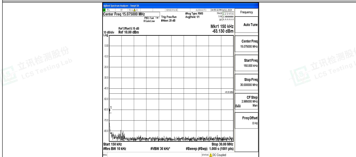
Band7_20MHz_16QAM_21100_1RB#0_0.15~30_0.15~30
