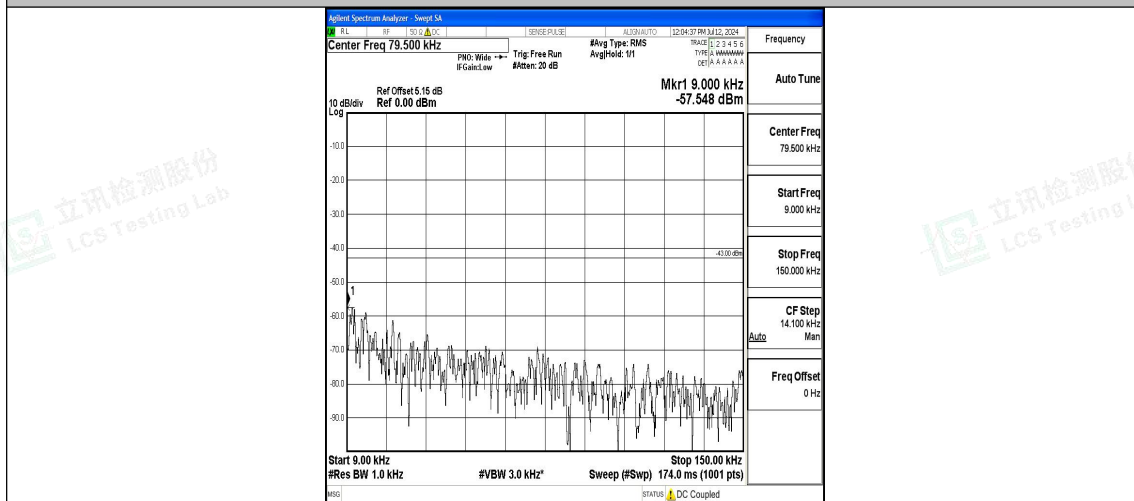
Band2_3MHz_QPSK_18615_1RB#0_0.009~0.15_0.009~0.15
