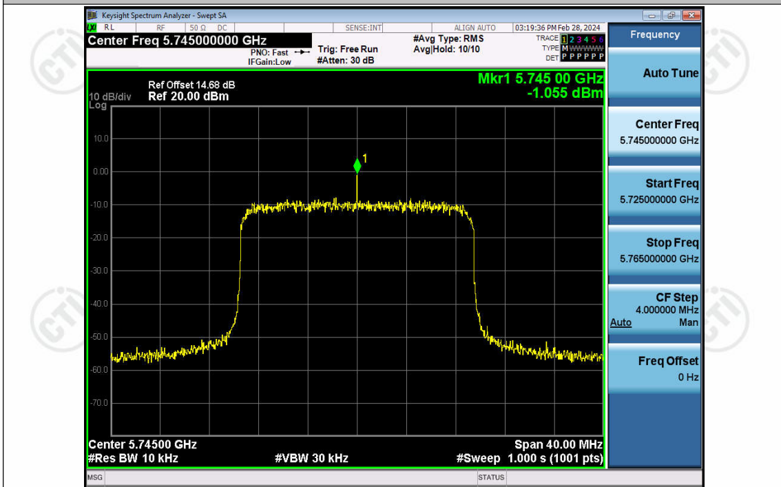
5G Slot 20MHz-Ant1-5745
