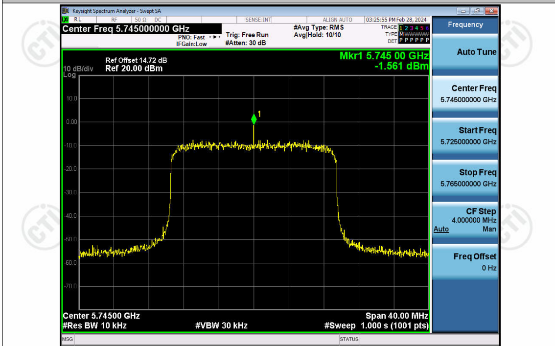
5G Slot 20MHz-Ant2-5745
