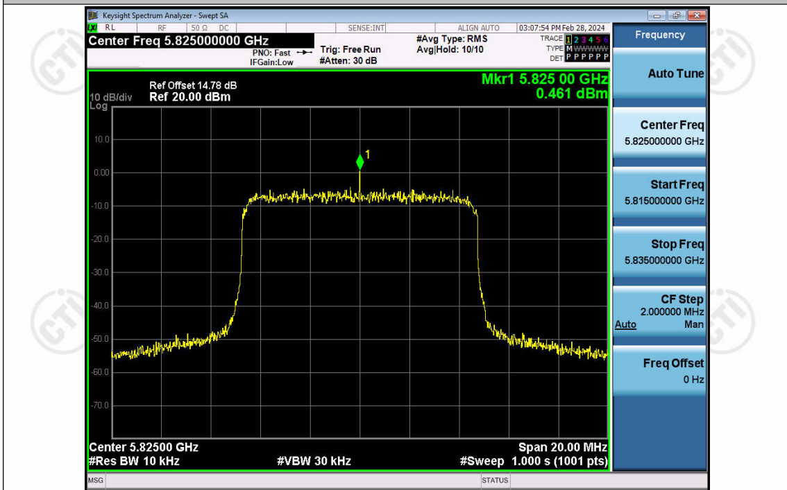
5G Slot 10MHz-Ant2-5825
