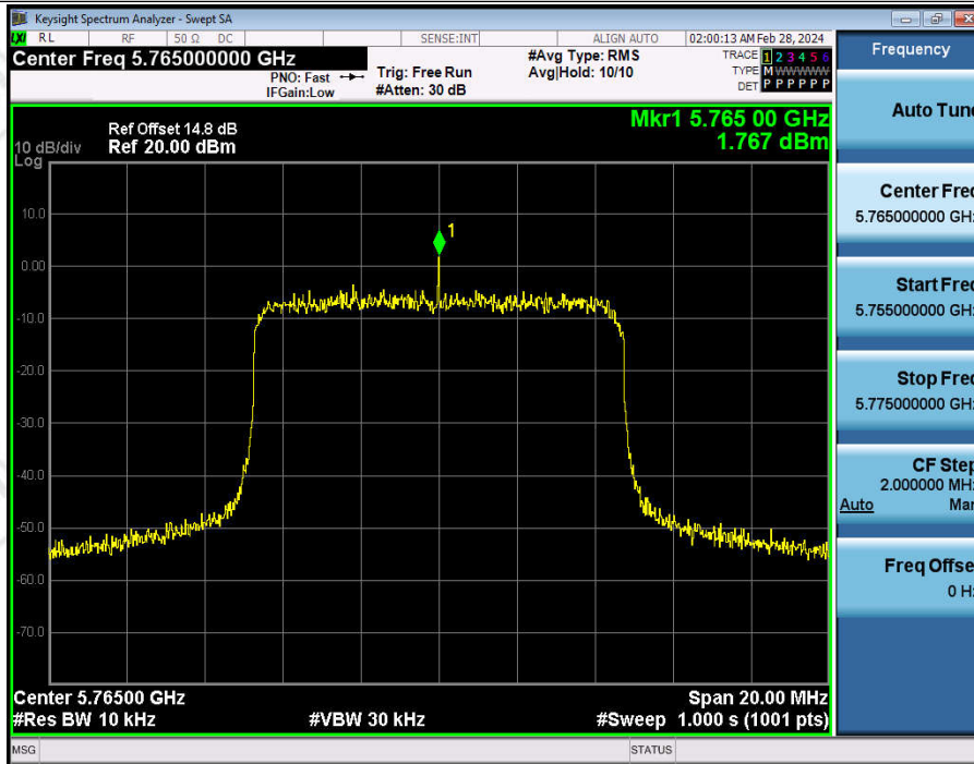
5G Slot 10MHz-Ant2-5765
