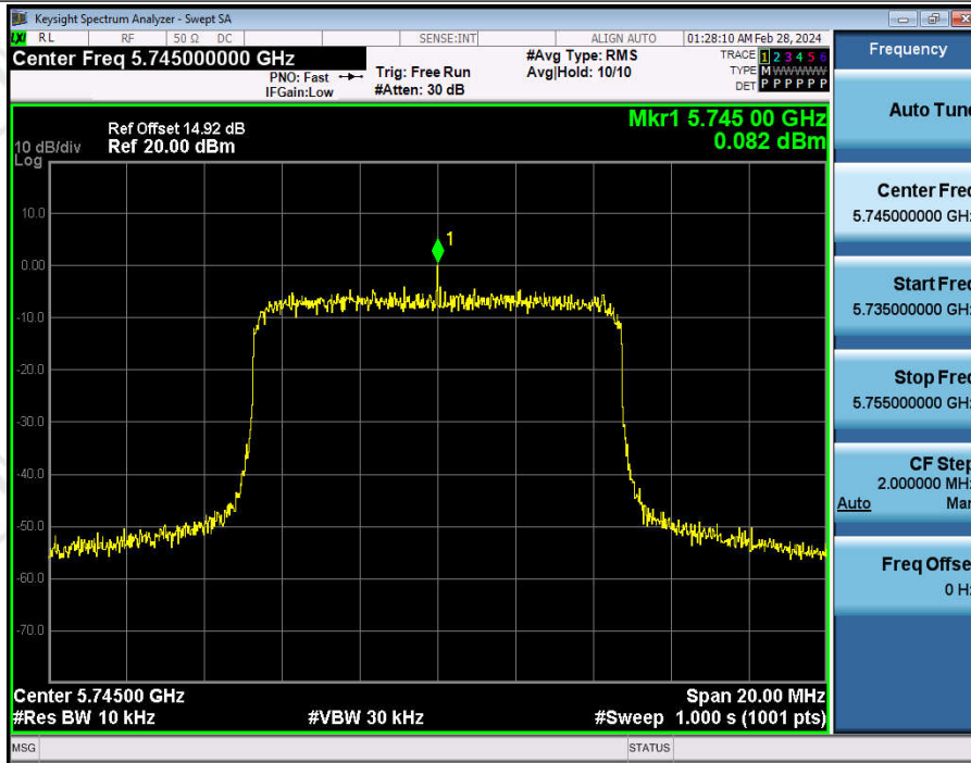
5G Slot 10MHz-Ant2-5745
