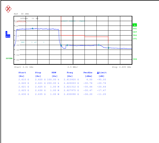
Band38_10MHz_QPSK_38200_50RB#0
