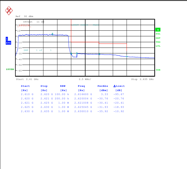
Band38_10MHz_16QAM_38200_50RB#0
