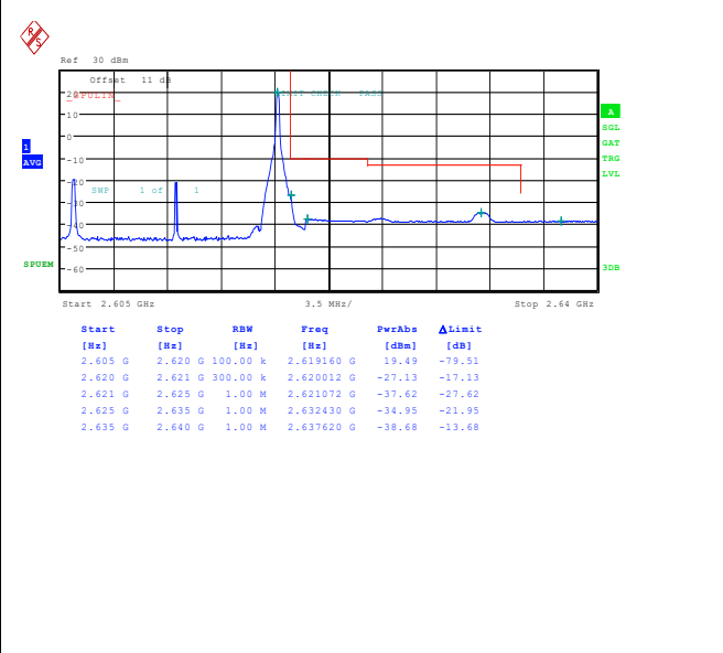
Band38_15MHz_16QAM_38175_1RB#74
