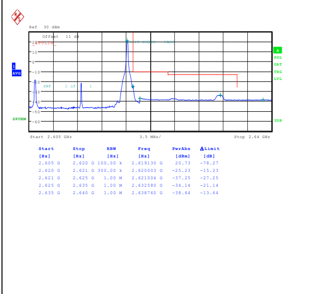
Band38_15MHz_QPSK_38175_1RB#74
