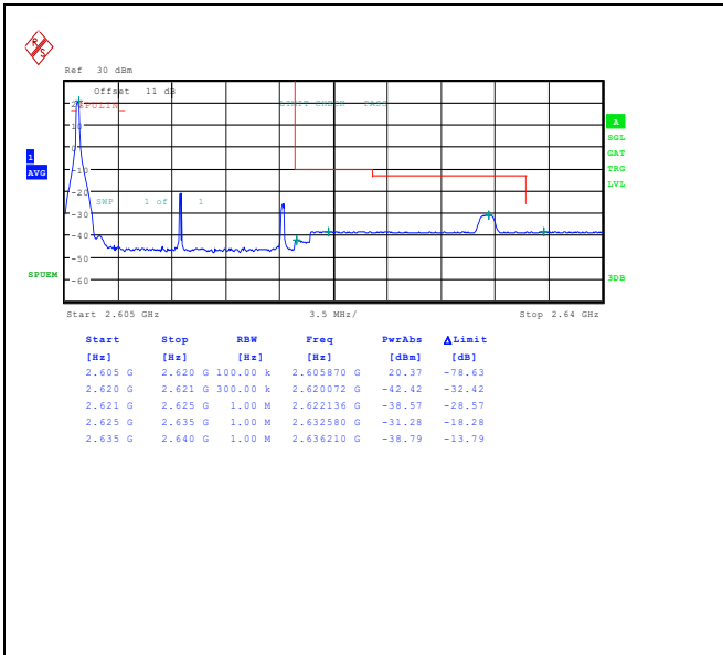
Band38_15MHz_QPSK_38175_1RB#0
