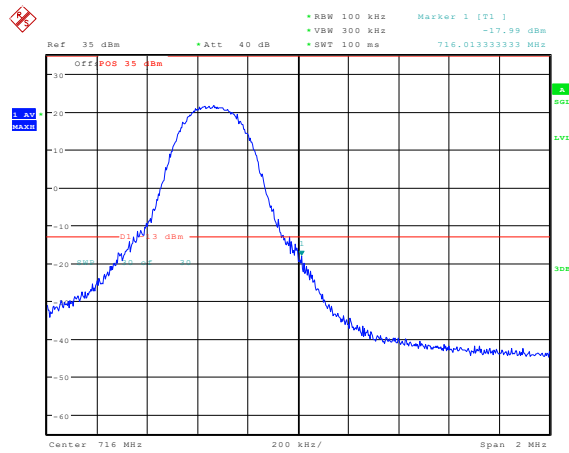
Band12-5MHz-QPSK-23155-1RB#24
