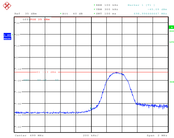
Band12-5MHz-16QAM-23035-1RB#24
