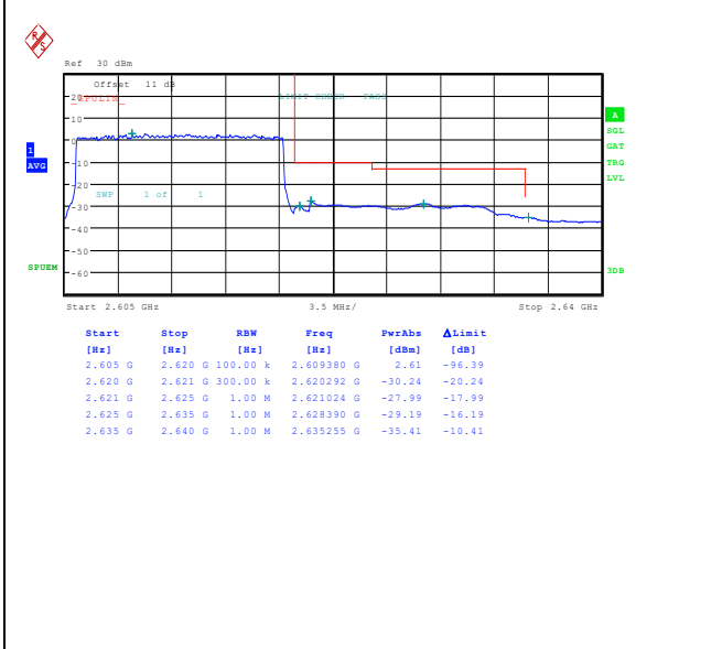
Band38_15MHz_QPSK_38175_1RB#74
