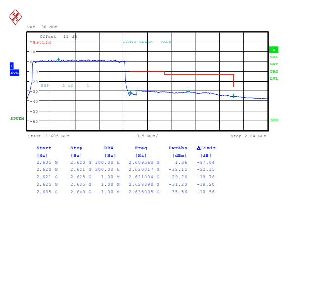
Band38_15MHz_16QAM_38175_1RB#74
