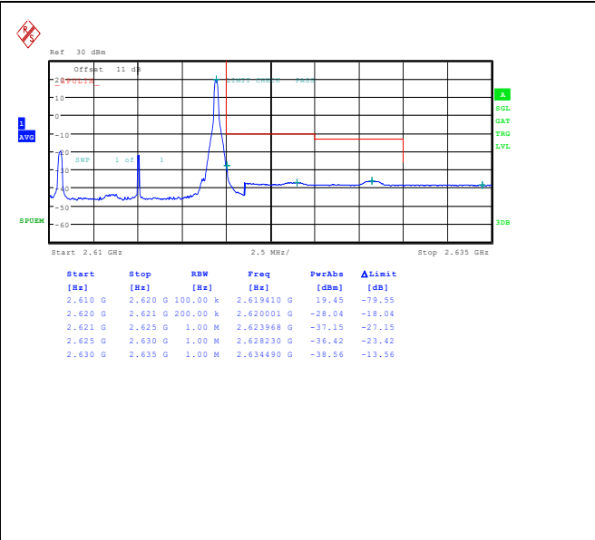
Band38_10MHz_16QAM_38200_1RB#49
