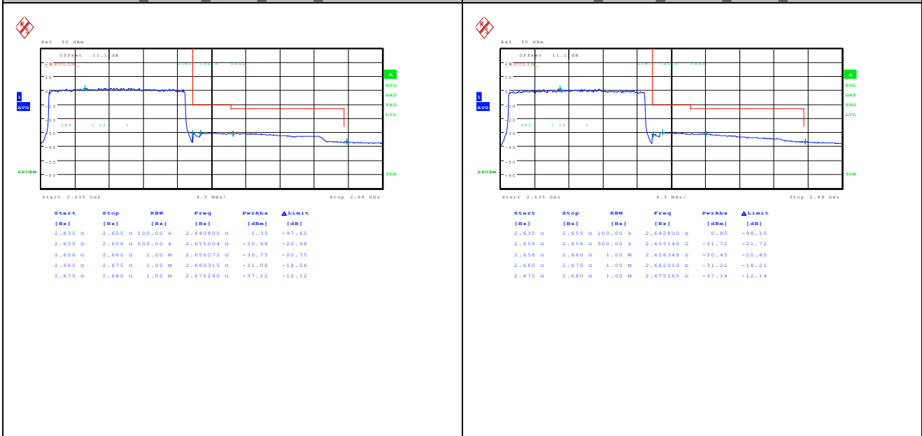
Band41_20MHz_QPSK_41140_100RB#0 Band41_20MHz_16QAM_41140_100RB#0
