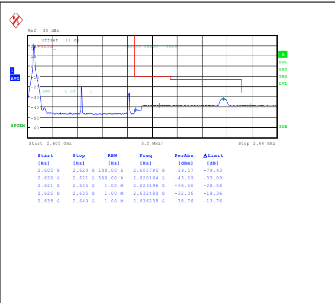
Band38_15MHz_16QAM_38175_1RB#0
