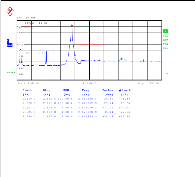
Band38_10MHz_QPSK_38200_1RB#49
