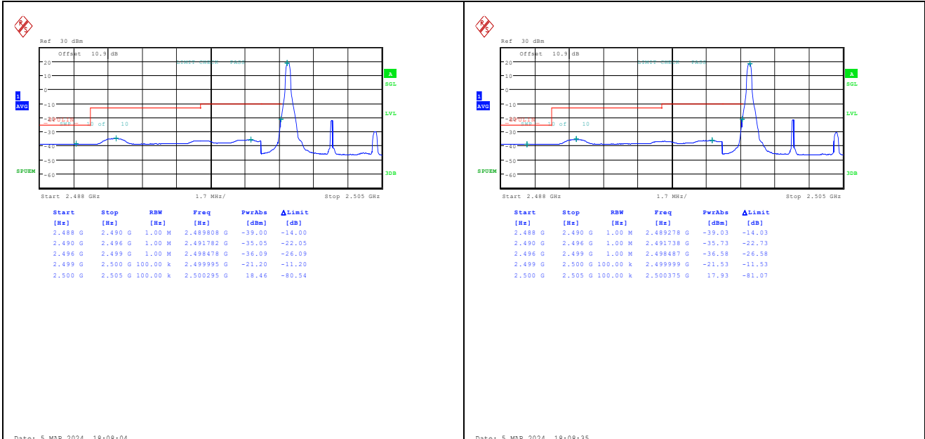
Band7_5MHz_QPSK_20775_1RB#0 Band7_5MHz_16QAM_20775_1RB#0
