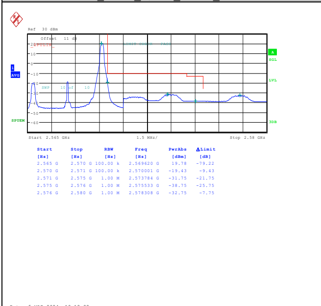
Band7_5MHz_QPSK_21425_1RB#24
