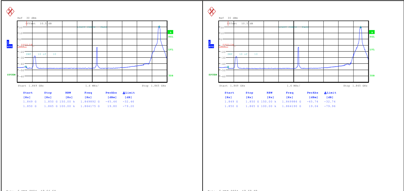
Band2_15MHz_QPSK_18675_1RB#74 Band2_15MHz_16QAM_18675_1RB#74
