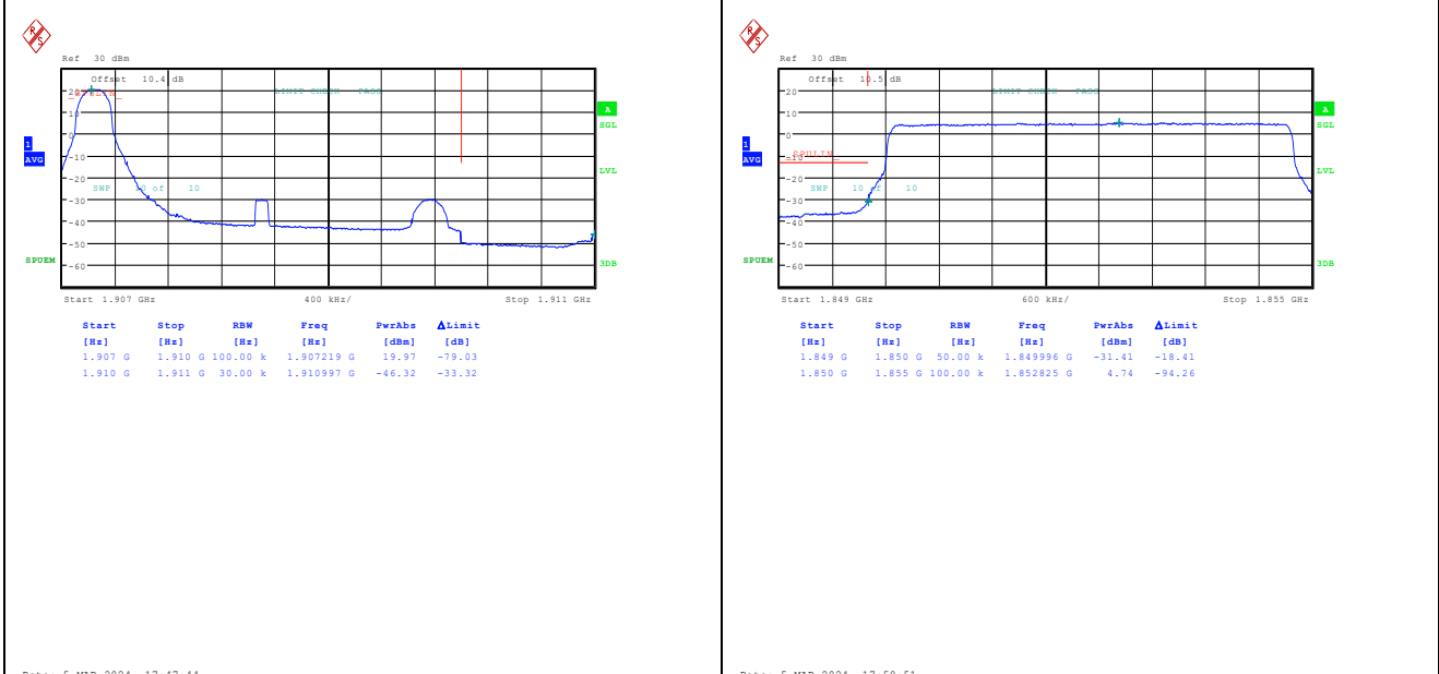
Band2_3MHz_QPSK_19185_1RB#0 Band2_5MHz_16QAM_18625_25RB#0
