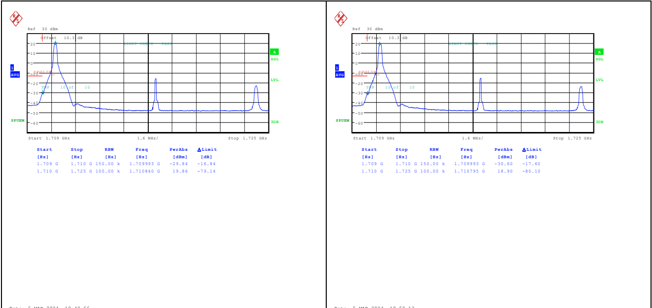
Band4_15MHz_QPSK_2025_1RB#0 Band4_15MHz_16QAM_2025_1RB#0
