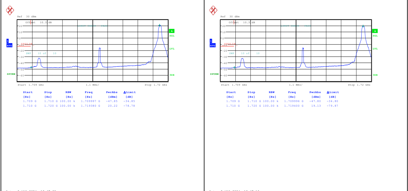
Band4_10MHz_QPSK_2000_1RB#49
