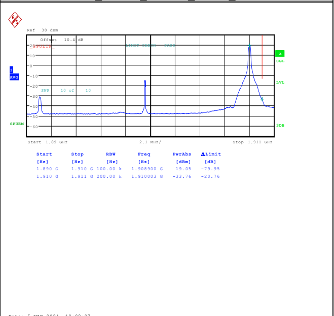
Band2_20MHz_16QAM_19100_1RB#99
