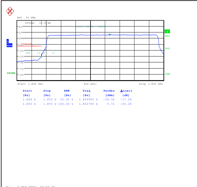
Band2_5MHz_QPSK_18625_25RB#0
