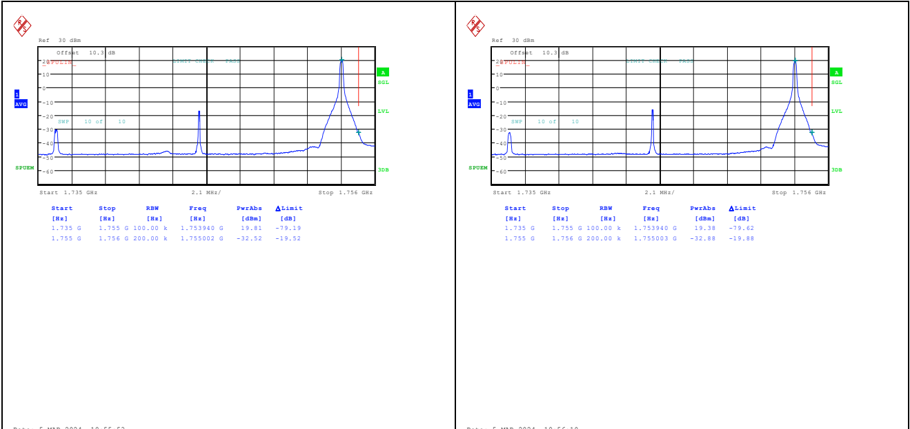
Band4_20MHz_QPSK_20300_1RB#99 Band4_20MHz_16QAM_20300_1RB#99
