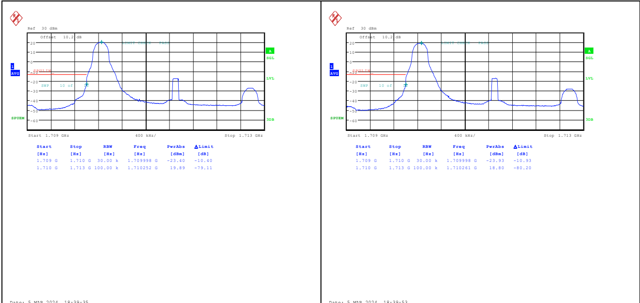
Band4_3MHz_QPSK_19965_1RB#0 Band4_3MHz_16QAM_19965_1RB#0
