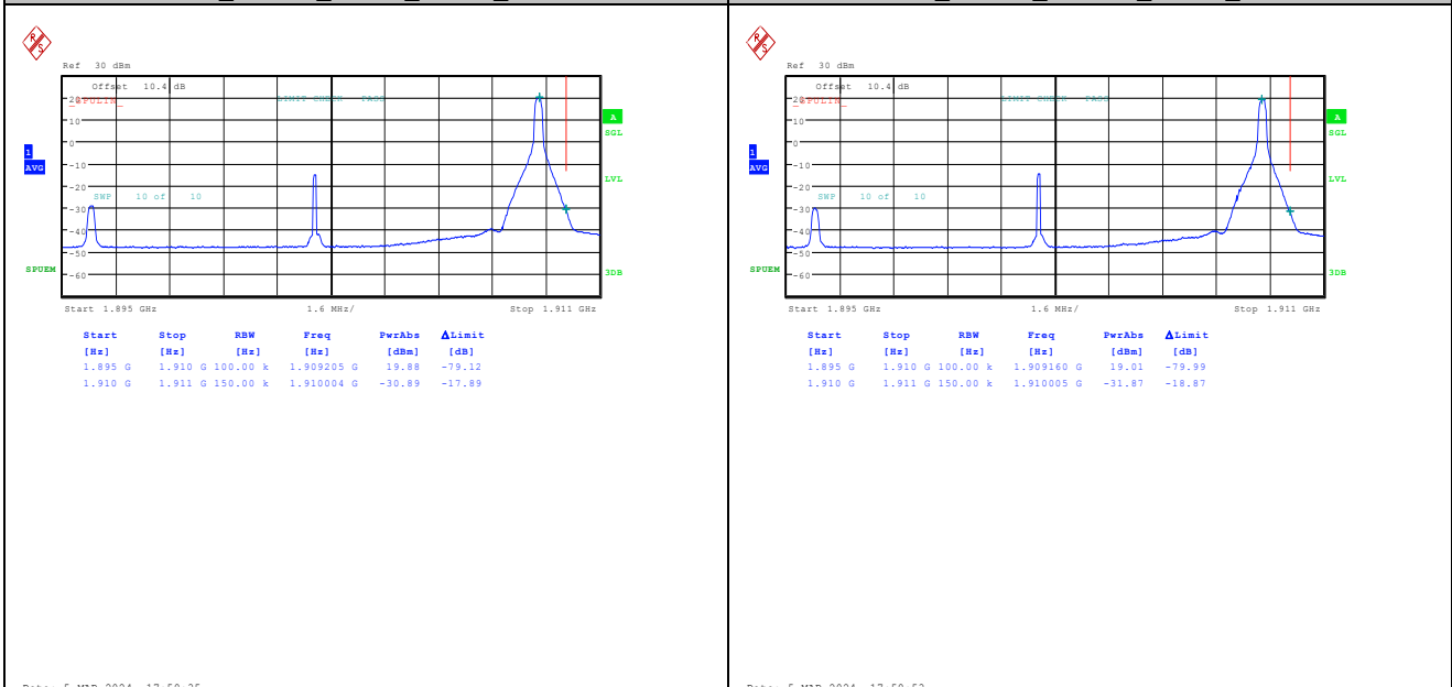
Band2_15MHz_QPSK_19125_1RB#74 Band2_15MHz_16QAM_19125_1RB#74
