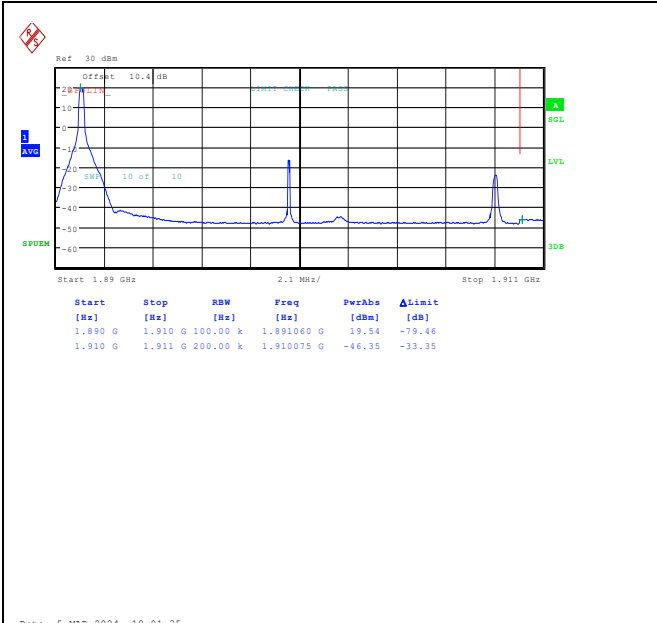
Band2_20MHz_QPSK_19100_1RB#0
