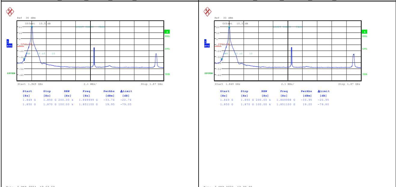
Band2_20MHz_QPSK_18700_1RB#0 Band2_20MHz_16QAM_18700_1RB#0
