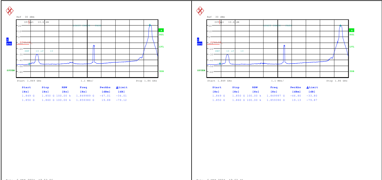
Band2_10MHz_QPSK_18650_1RB#49 Band2_10MHz_16QAM_18650_1RB#49
