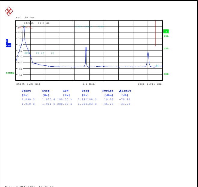
Band2_20MHz_16QAM_19100_1RB#0
