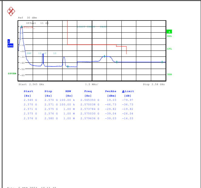
Band7_5MHz_16QAM_21425_1RB#0
