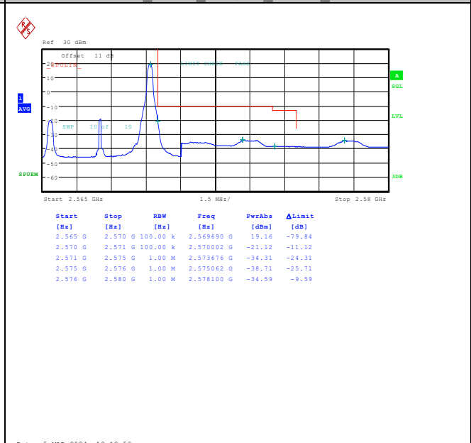
Band7_5MHz_16QAM_21425_1RB#24
