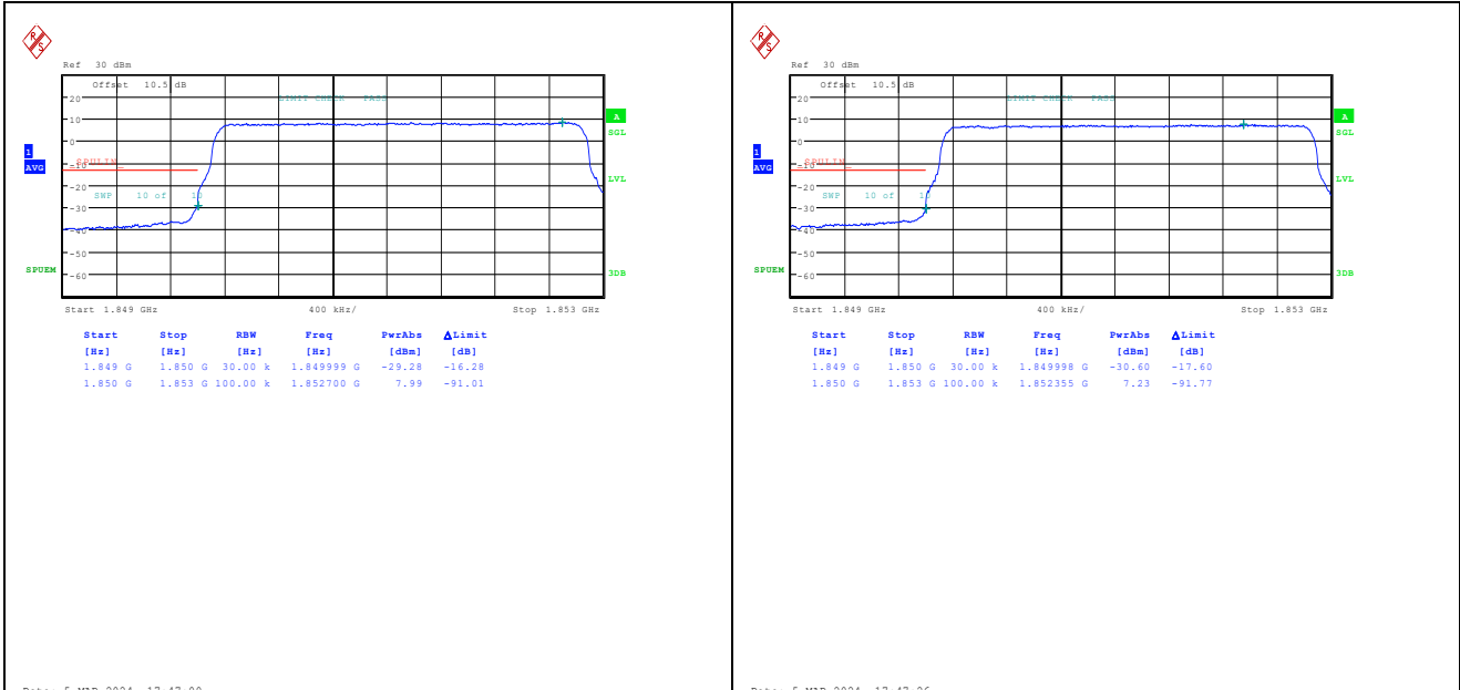
Band2_3MHz_QPSK_18615_15RB#0 Band2_3MHz_16QAM_18615_15RB#0
