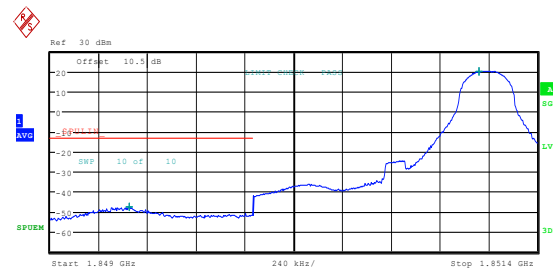
Band2_1.4MHz_16QAM_18607_1RB#0
