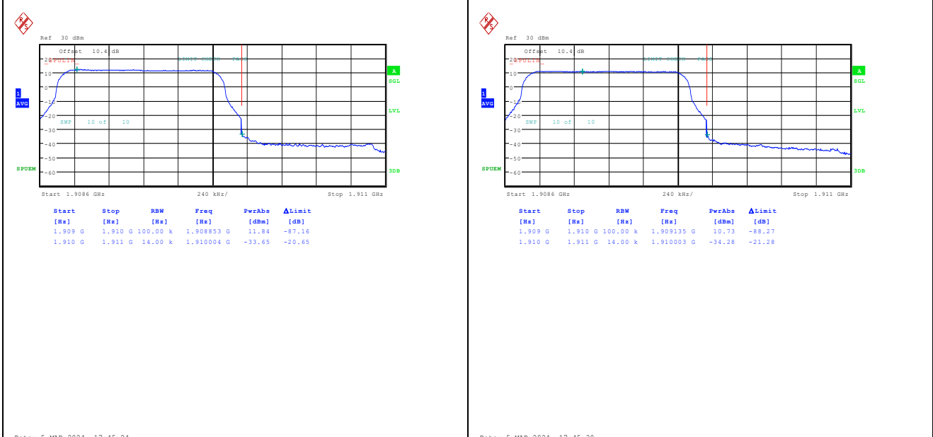
Band2_1.4MHz_QPSK_19193_6RB#0 Band2_1.4MHz_16QAM_19193_6RB#0
