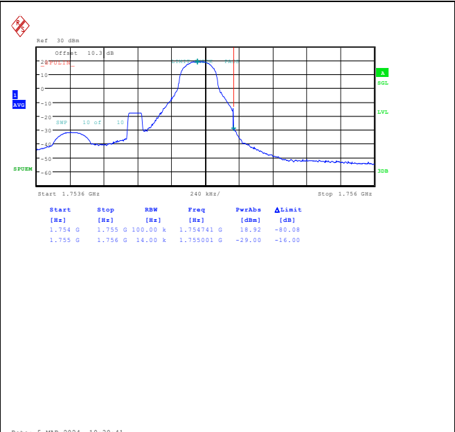
Band4_1.4MHz_16QAM_20393_1RB#5
