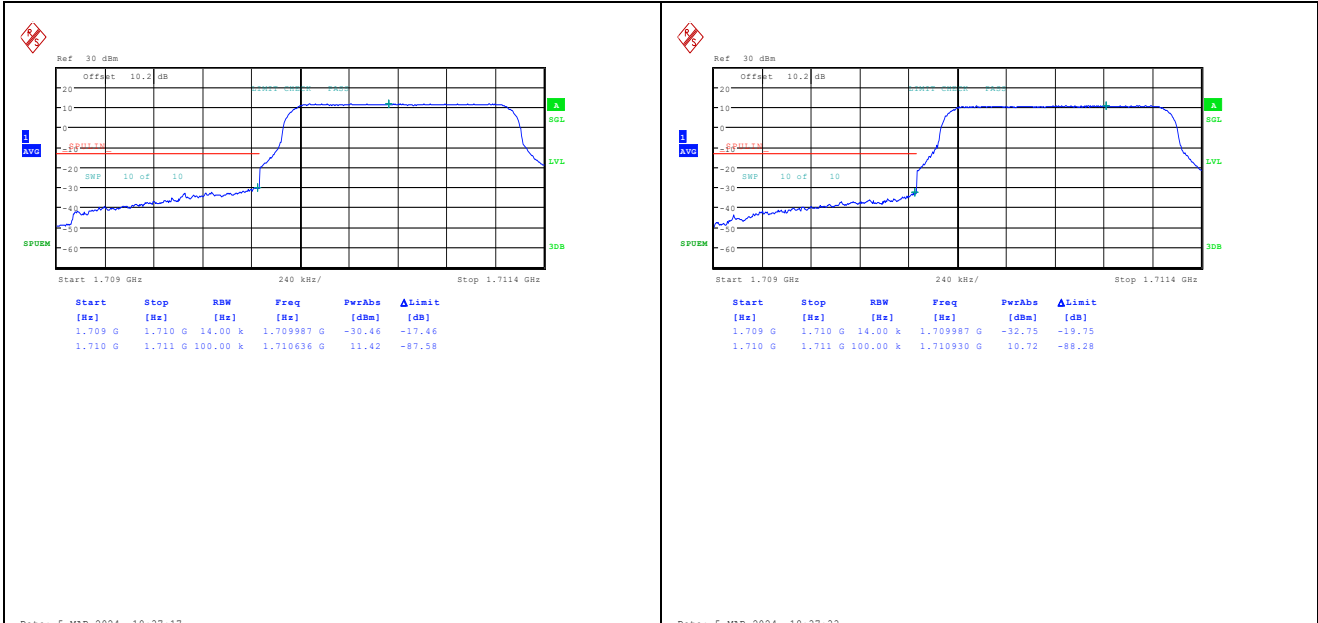
Band4_1.4MHz_QPSK_19957_6RB#0
