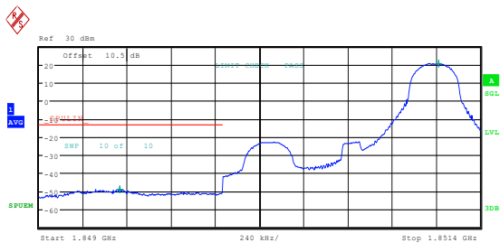
Band2_1.4MHz_QPSK_18607_1RB#0
