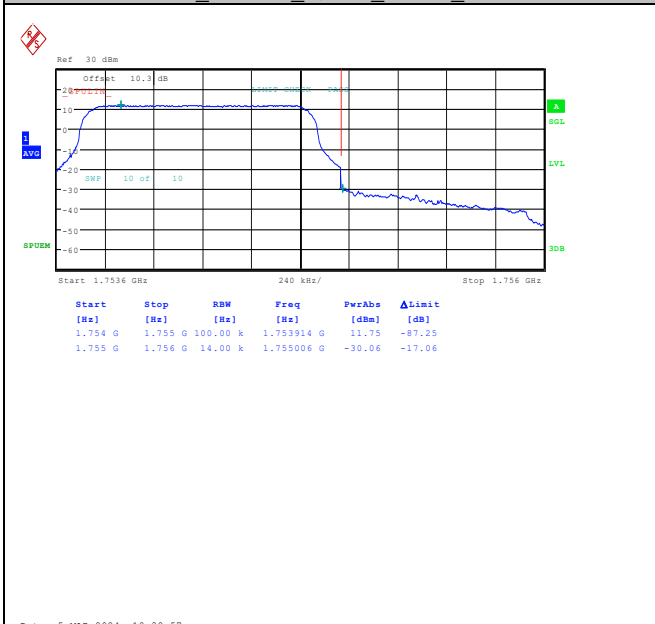
Band4_1.4MHz_QPSK_20393_6RB#0
