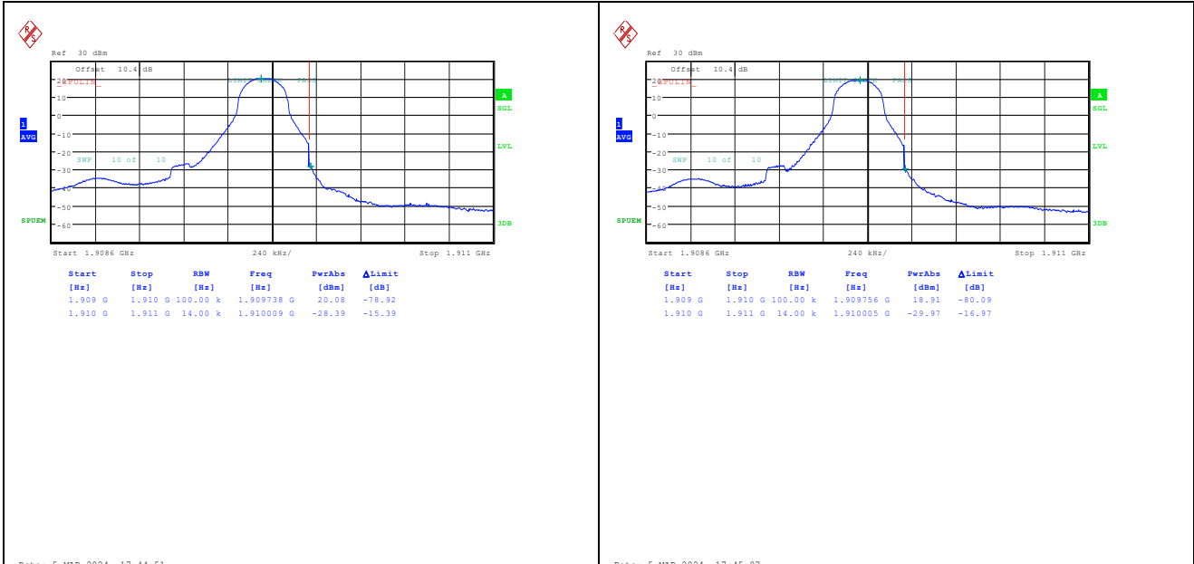
Band2_1.4MHz_QPSK_19193_1RB#5 Band2_1.4MHz_16QAM_19193_1RB#5
