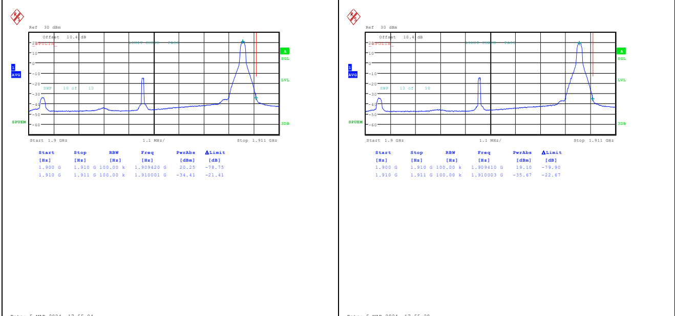
Band2_10MHz_QPSK_19150_1RB#49
