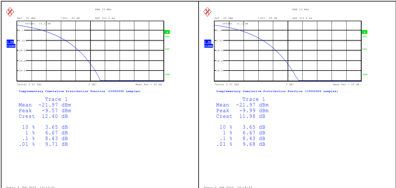
Band38-20MHz-QPSK-38150-1RB#0-PASS | Band38-20MHz-16QAM-38150-1RB#0-PASS
