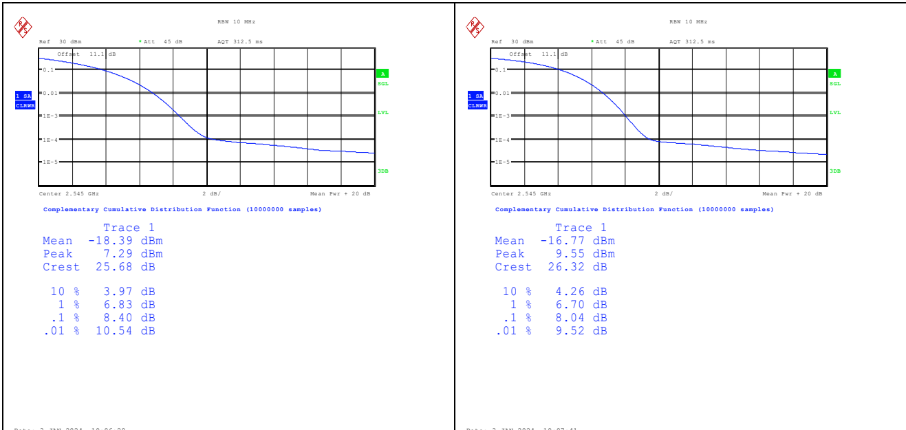
Band41-20MHz-QPSK-40140-1RB#0-PASS Band41-20MHz-16QAM-40140-1RB#0-PASS
