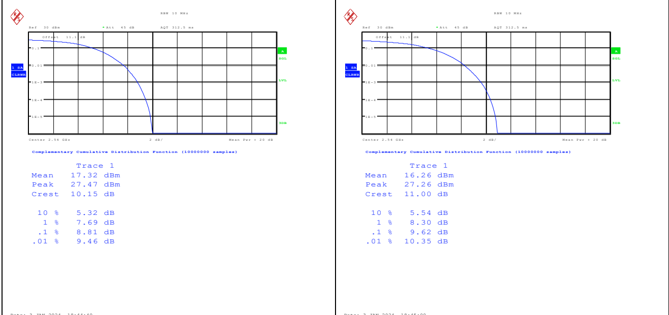
Band41-10MHz-QPSK-40090-50RB#0-PASS Band41-10MHz-16QAM-40090-50RB#0-PASS
