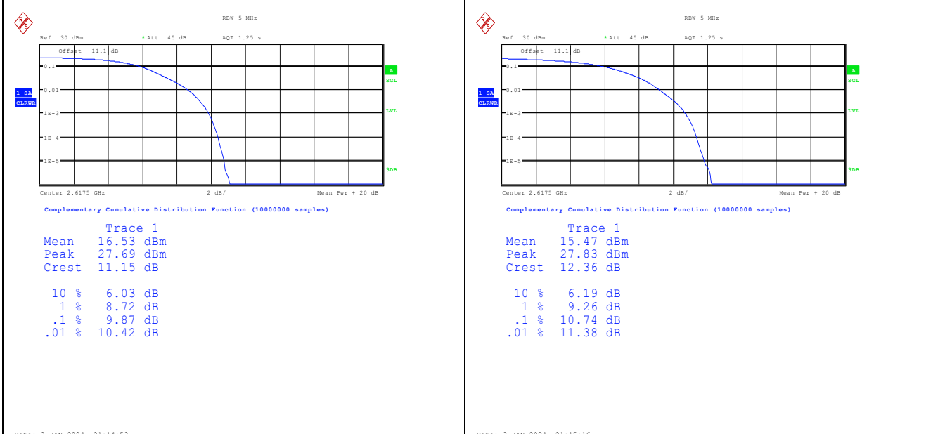
Band38-5MHz-QPSK-38225-25RB#0-PASS Band38-5MHz-16QAM-38225-25RB#0-PASS
