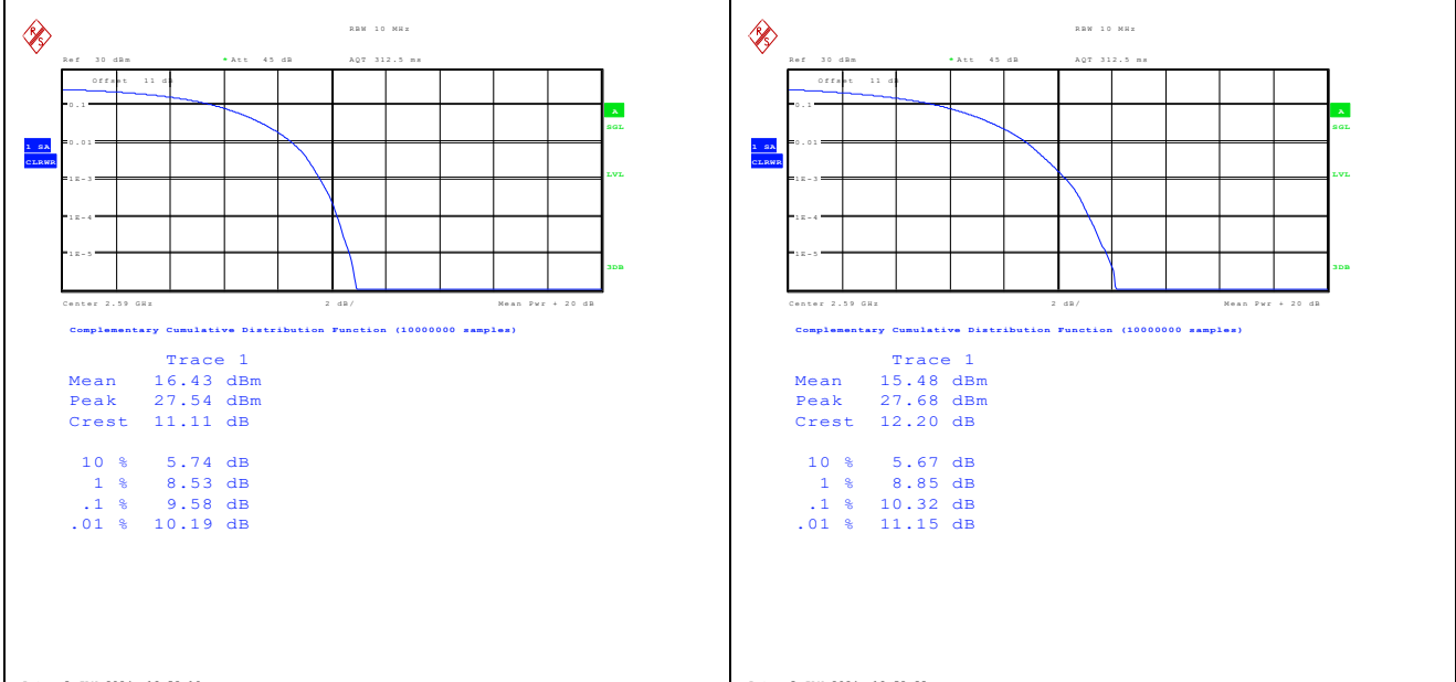
Band41-15MHz-QPSK-40590-75RB#0-PASS Band41-15MHz-16QAM-40590-75RB#0-PASS
