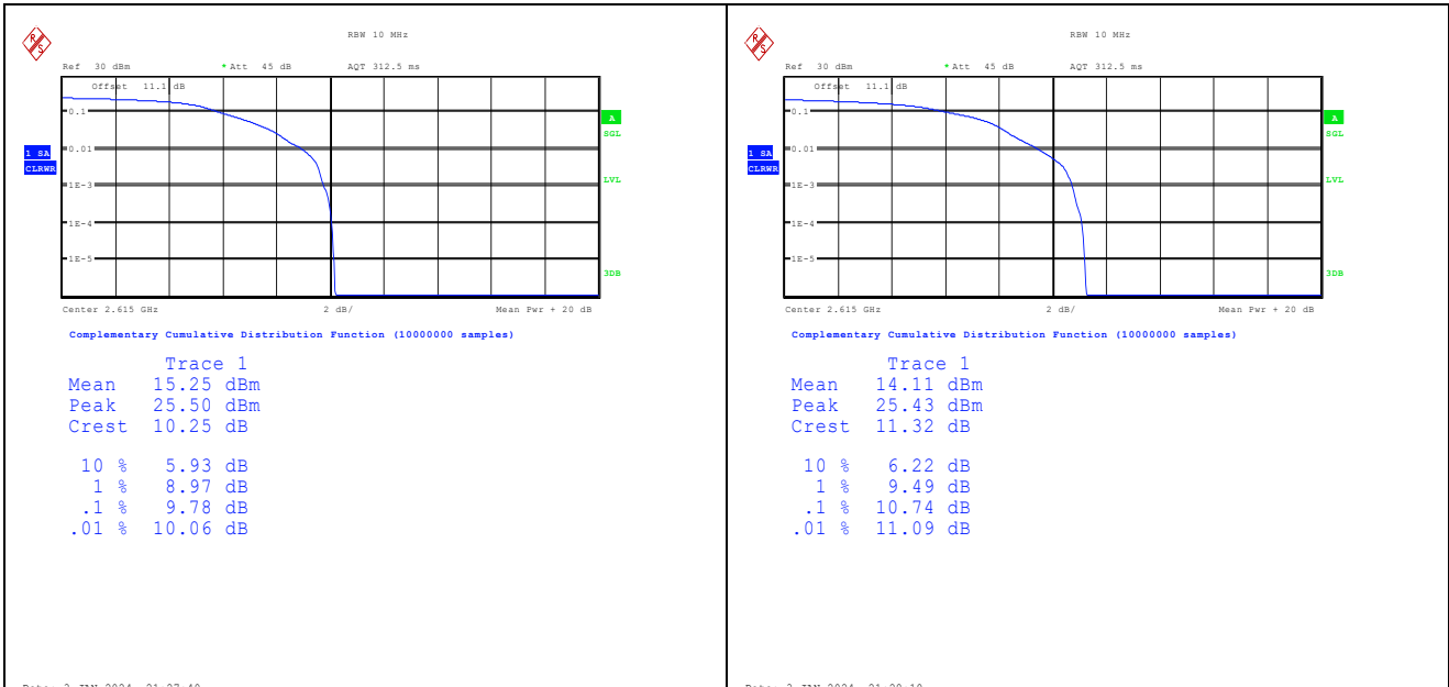
Band38-10MHz-QPSK-38200-1RB#0-PASS Band38-10MHz-16QAM-38200-1RB#0-PASS
