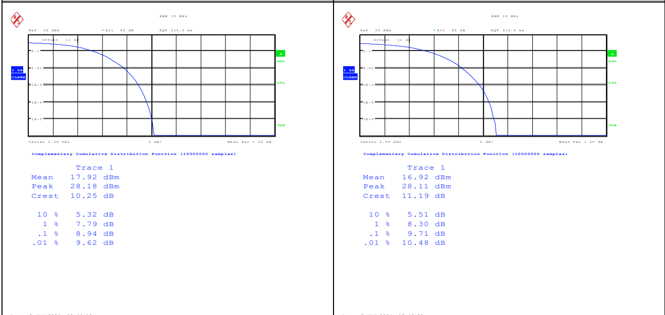
Band41-10MHz-QPSK-40590-50RB#0-PASS Band41-10MHz-16QAM-40590-50RB#0-PASS
