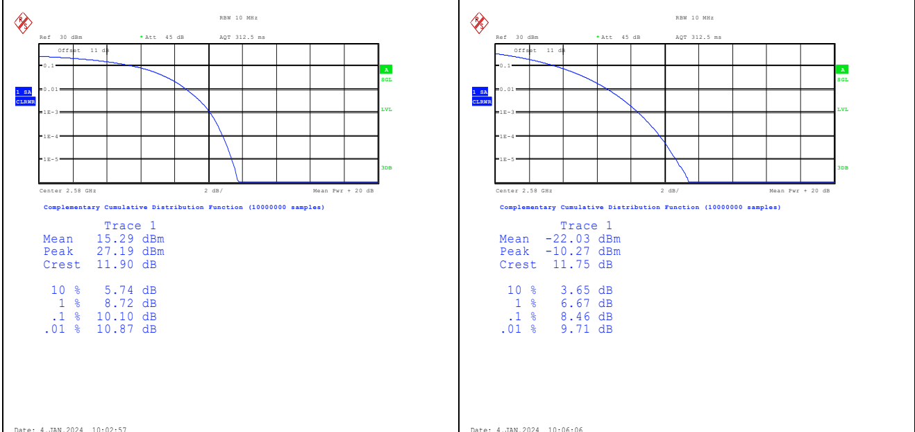
Band38-20MHz-QPSK-37850-100RB#0-PASS Band38-20MHz-16QAM-37850-100RB#0-PASS
