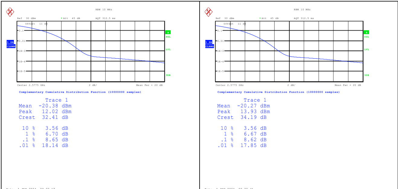
Band38-15MHz-QPSK-37825-1RB#0-PASS Band38-15MHz-16QAM-37825-1RB#0-PASS
