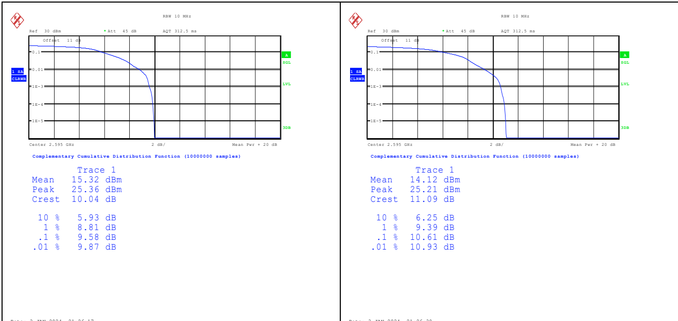
Band38-10MHz-QPSK-38000-1RB#0-PASS | Band38-10MHz-16QAM-38000-1RB#0-PASS
