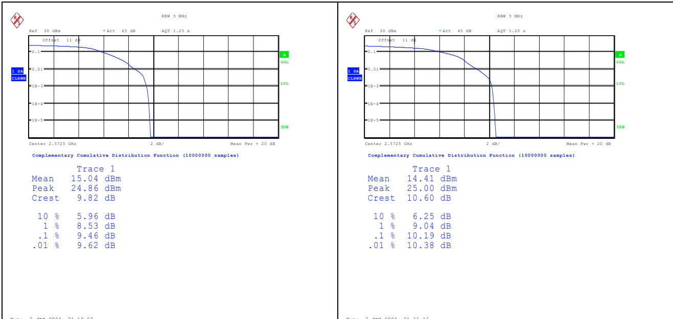
Band38-5MHz-QPSK-37775-1RB#0-PASS Band38-5MHz-16QAM-37775-1RB#0-PASS
