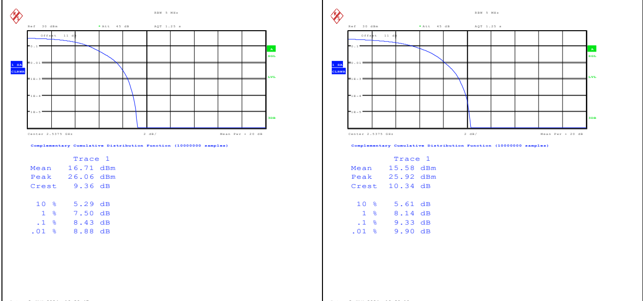
Band41-5MHz-QPSK-40065-25RB#0-PASS Band41-5MHz-16QAM-40065-25RB#0-PASS
