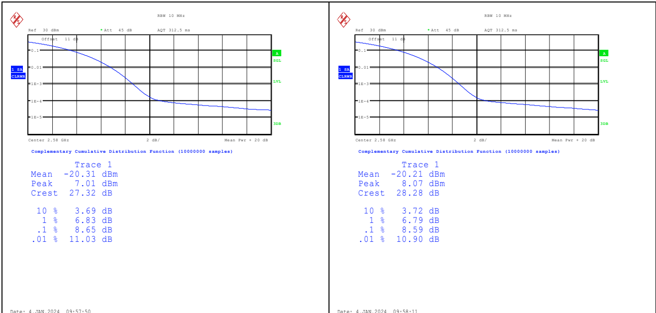
Band38-20MHz-QPSK-37850-1RB#0-PASS Band38-20MHz-16QAM-37850-1RB#0-PASS
