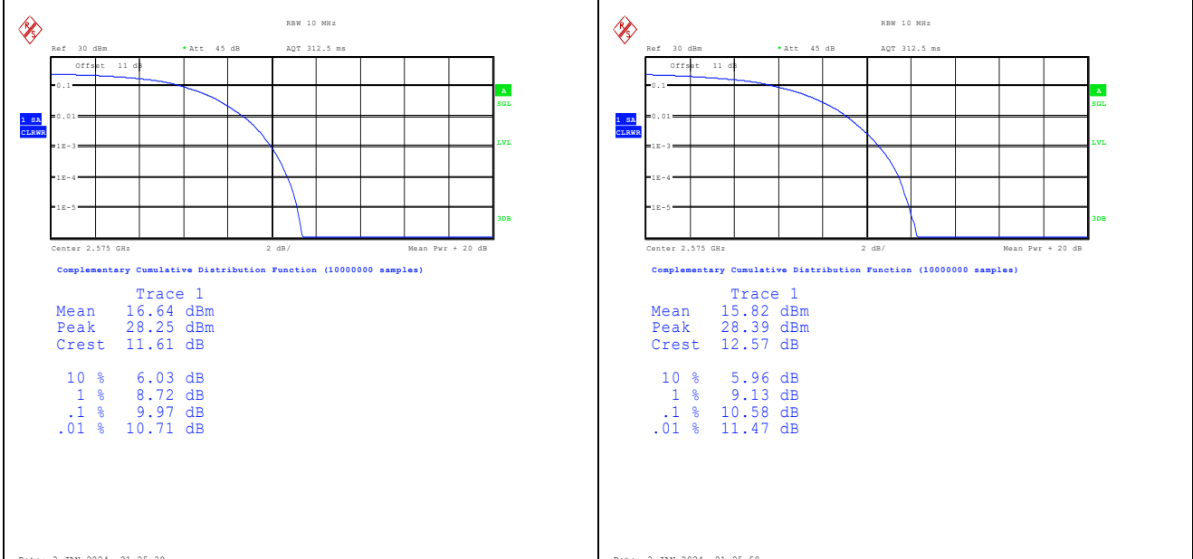
Band38-10MHz-QPSK-37800-50RB#0-PASS Band38-10MHz-16QAM-37800-50RB#0-PASS
