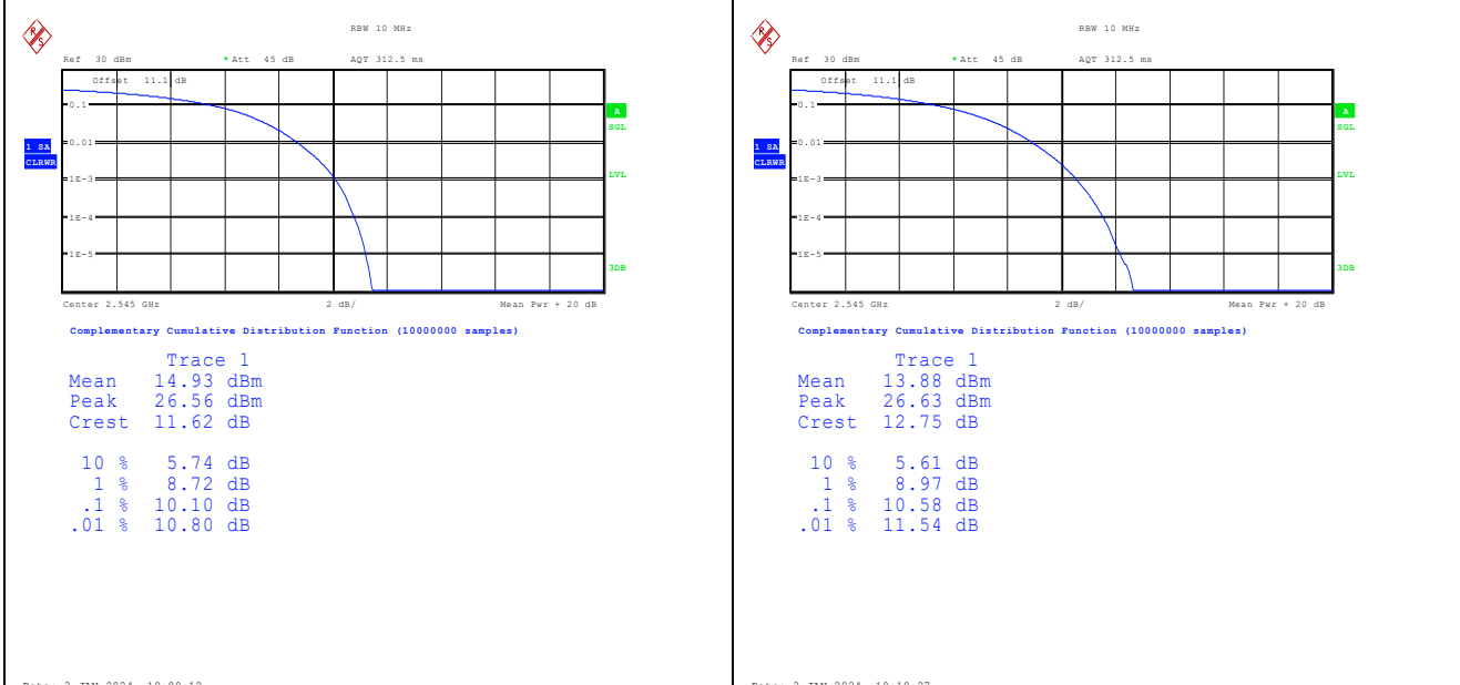
Band41-20MHz-QPSK-40140-100RB#0-PASS Band41-20MHz-16QAM-40140-100RB#0-PASS
