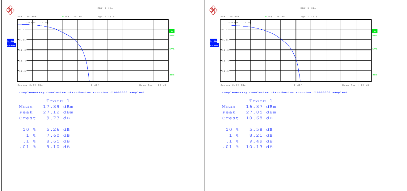
Band41-5MHz-QPSK-40590-25RB#0-PASS Band41-5MHz-16QAM-40590-25RB#0-PASS
