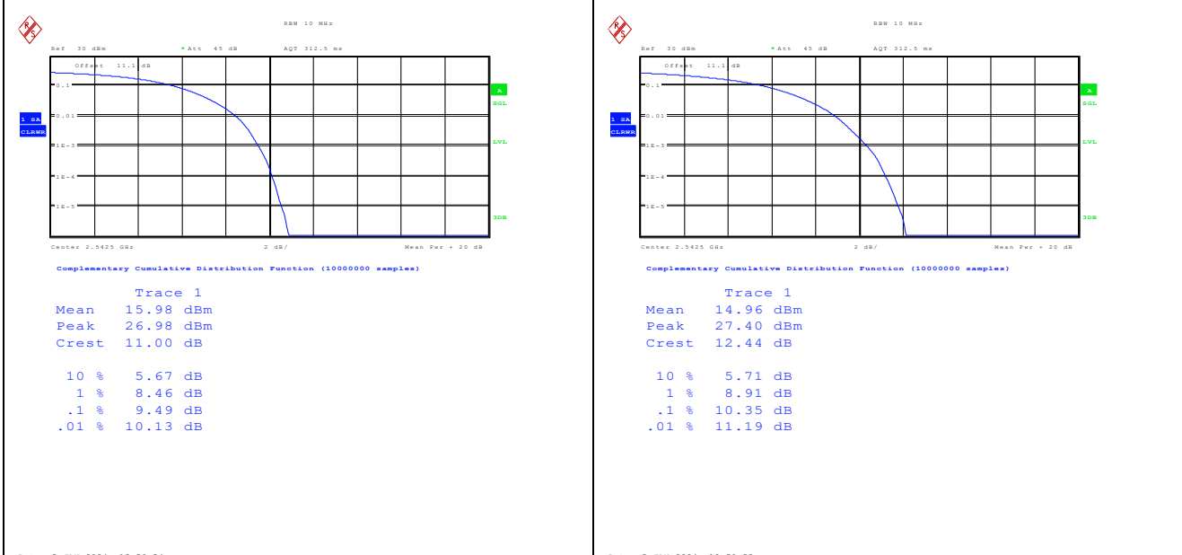
Band41-15MHz-QPSK-40115-75RB#0-PASS Band41-15MHz-16QAM-40115-75RB#0-PASS
