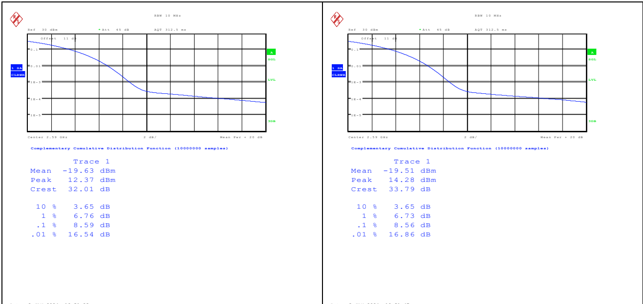
Band41-15MHz-QPSK-40590-1RB#0-PASS Band41-15MHz-16QAM-40590-1RB#0-PASS
