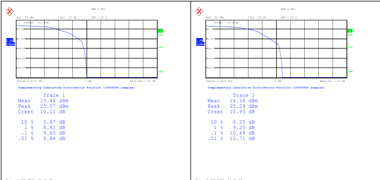
Band38-5MHz-QPSK-38225-1RB#0-PASS Band38-5MHz-16QAM-38225-1RB#0-PASS
