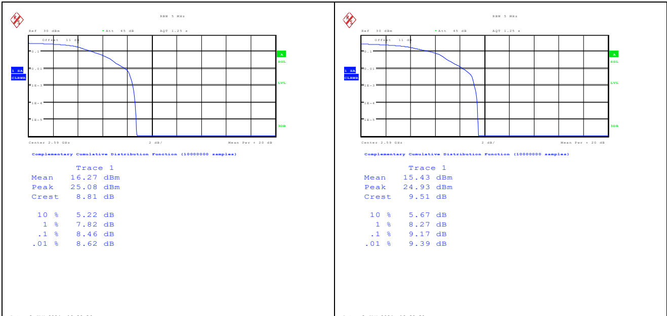
Band41-5MHz-QPSK-40590-1RB#0-PASS Band41-5MHz-16QAM-40590-1RB#0-PASS
