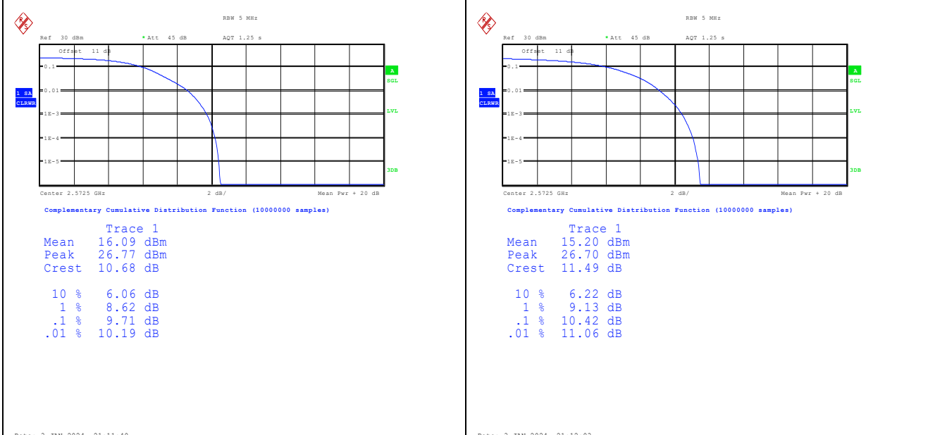
Band38-5MHz-QPSK-37775-25RB#0-PASS Band38-5MHz-16QAM-37775-25RB#0-PASS
