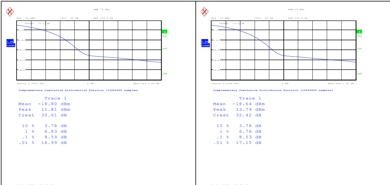
Band41-15MHz-QPSK-40115-1RB#0-PASS Band41-15MHz-16QAM-40115-1RB#0-PASS
