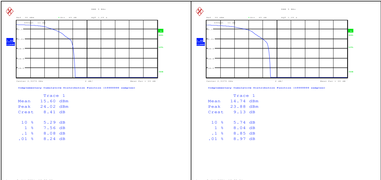
Band41-5MHz-QPSK-40065-1RB#0-PASS Band41-5MHz-16QAM-40065-1RB#0-PASS
