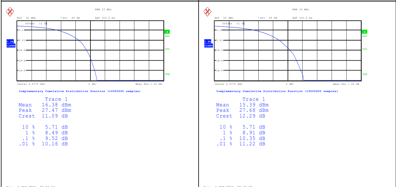
Band38-15MHz-QPSK-37825-75RB#0-PASS Band38-15MHz-16QAM-37825-75RB#0-PASS
