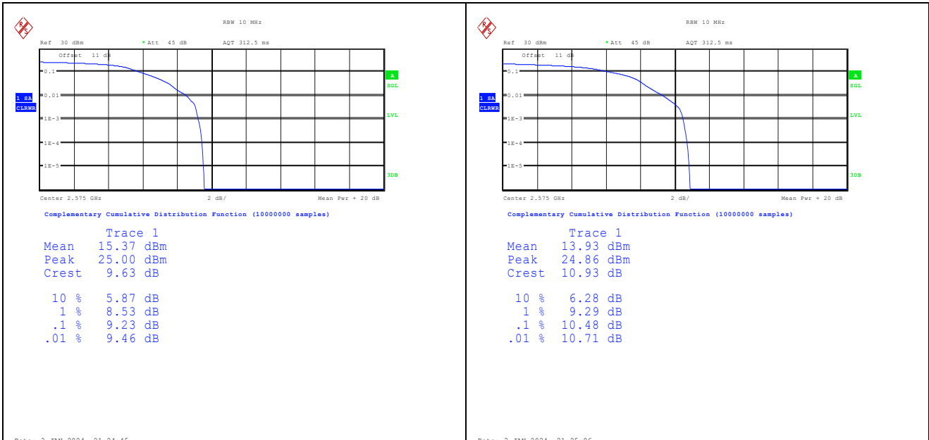
Band38-10MHz-QPSK-37800-1RB#0-PASS Band38-10MHz-16QAM-37800-1RB#0-PASS
