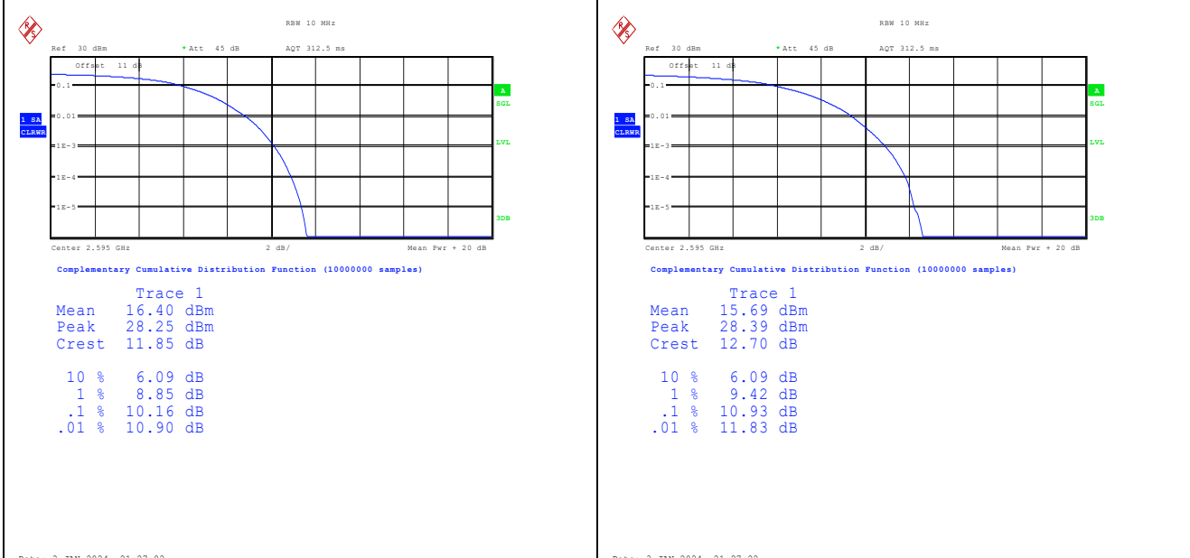
Band38-10MHz-QPSK-38000-50RB#0-PASS | Band38-10MHz-16QAM-38000-50RB#0-PASS
