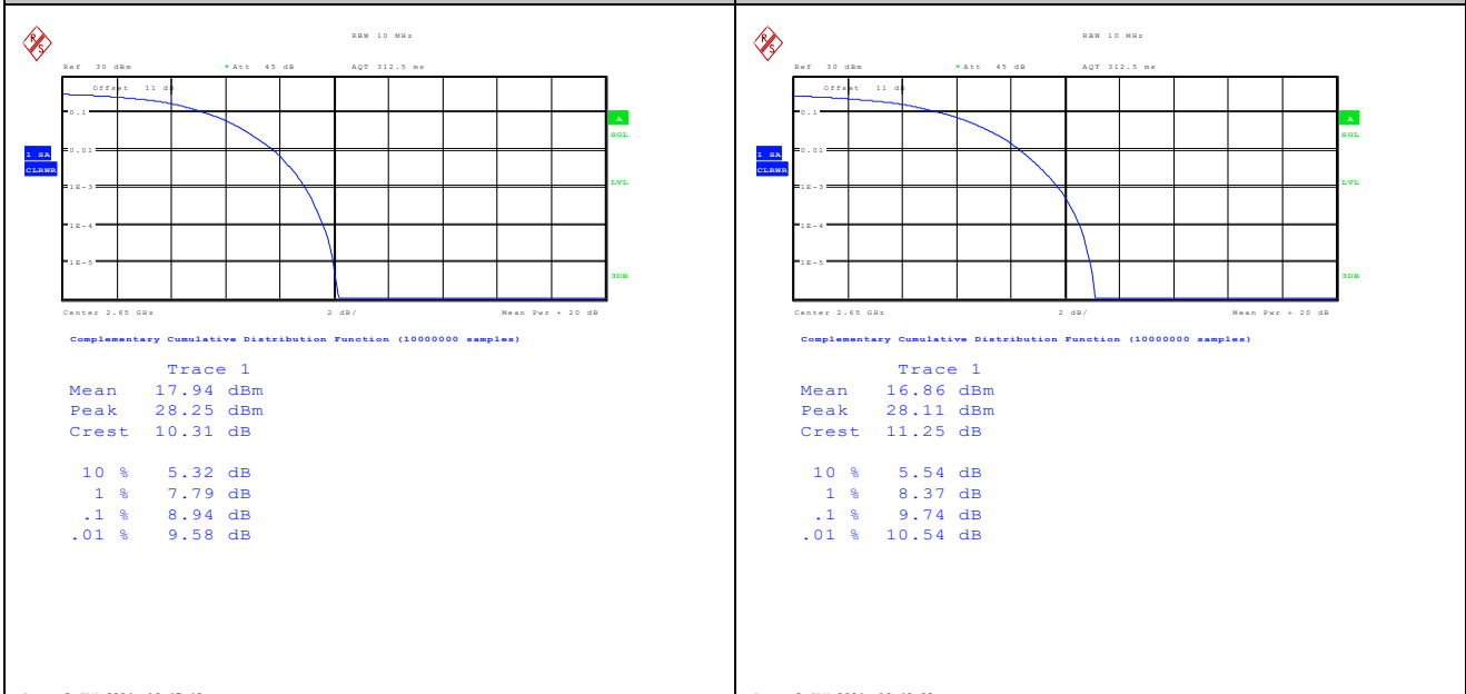
Band41-10MHz-QPSK-41190-50RB#0-PASS Band41-10MHz-16QAM-41190-50RB#0-PASS
