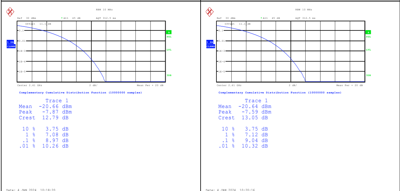
Band38-20MHz-QPSK-38150-100RB#0-PASS | Band38-20MHz-16QAM-38150-100RB#0-PASS
