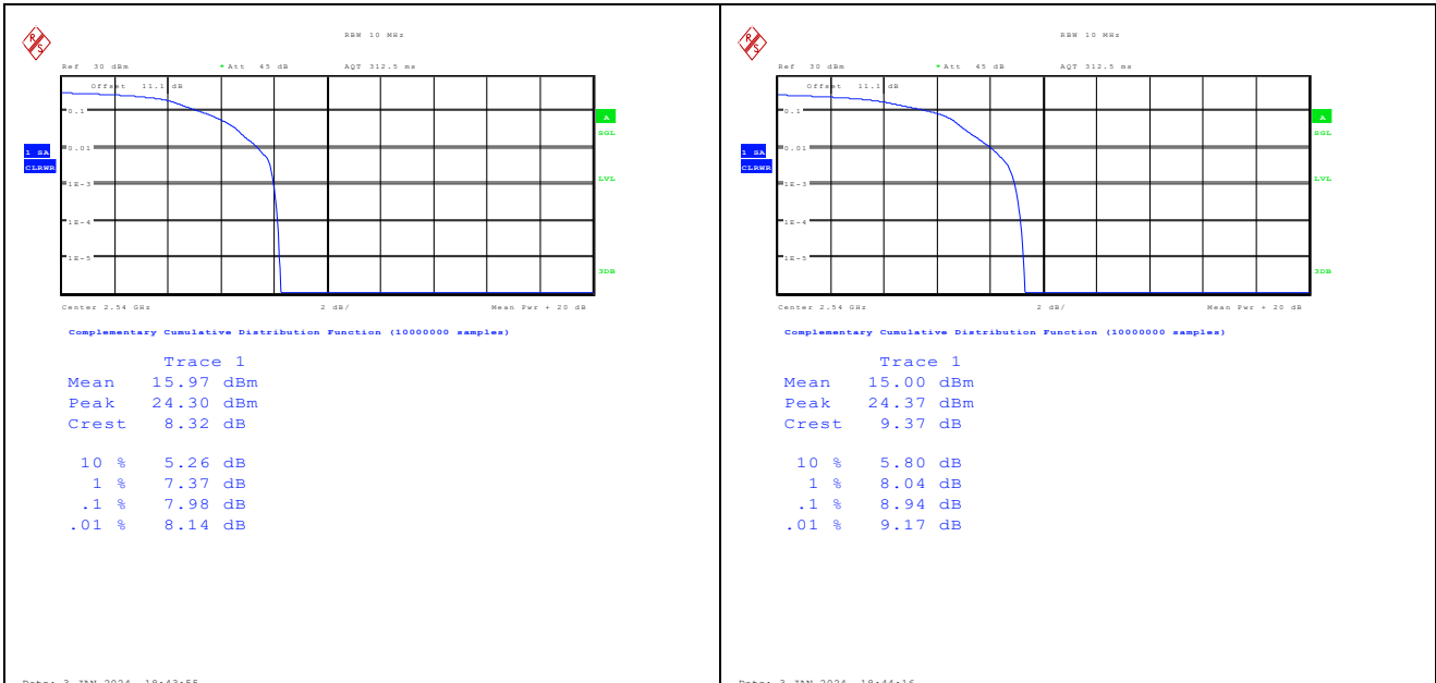
Band41-10MHz-QPSK-40090-1RB#0-PASS Band41-10MHz-16QAM-40090-1RB#0-PASS
