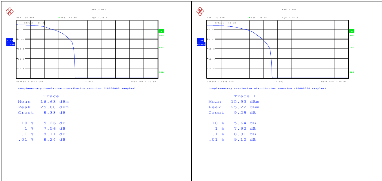
Band41-5MHz-QPSK-41215-1RB#0-PASS Band41-5MHz-16QAM-41215-1RB#0-PASS
