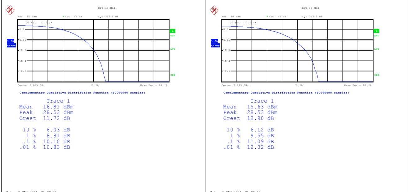
Band38-10MHz-QPSK-38200-50RB#0-PASS Band38-10MHz-16QAM-38200-50RB#0-PASS
