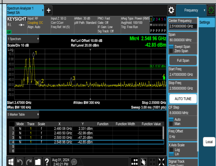
DH5-Ant1-Hop 2480-PASS
