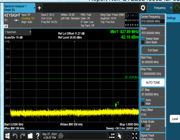
11N40SISO-Ant1-2437-30~1000-PASS
