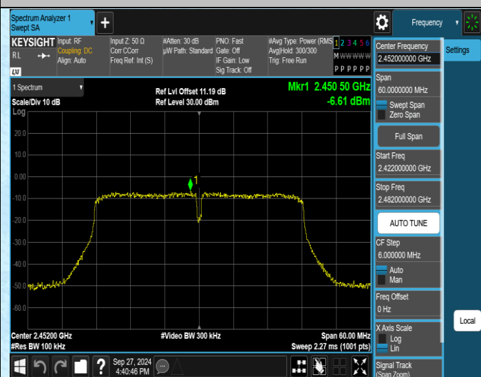
11N40SISO-Ant1-2452-0~Reference-PASS
