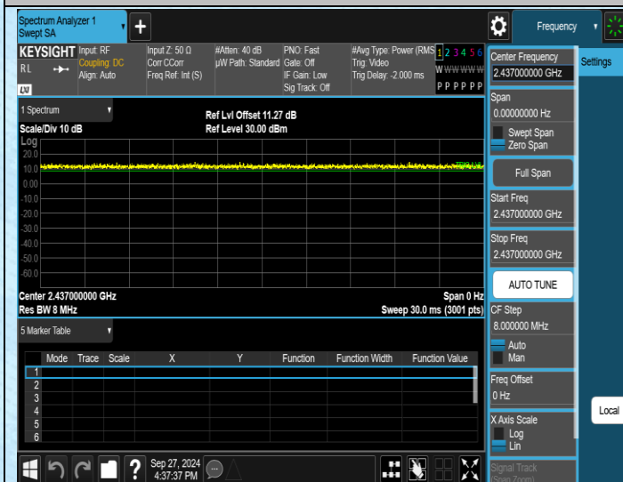
NTVN-11N40SISO-Ant1-2437
