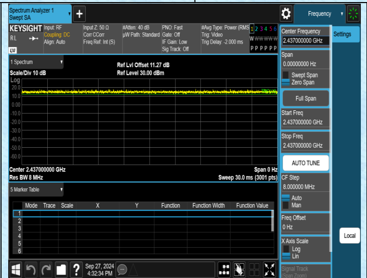
NTVN-11N20SISO-Ant1-2437
