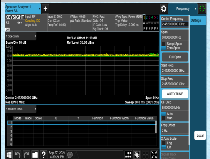
NTVN-11N40SISO-Ant1-2452
