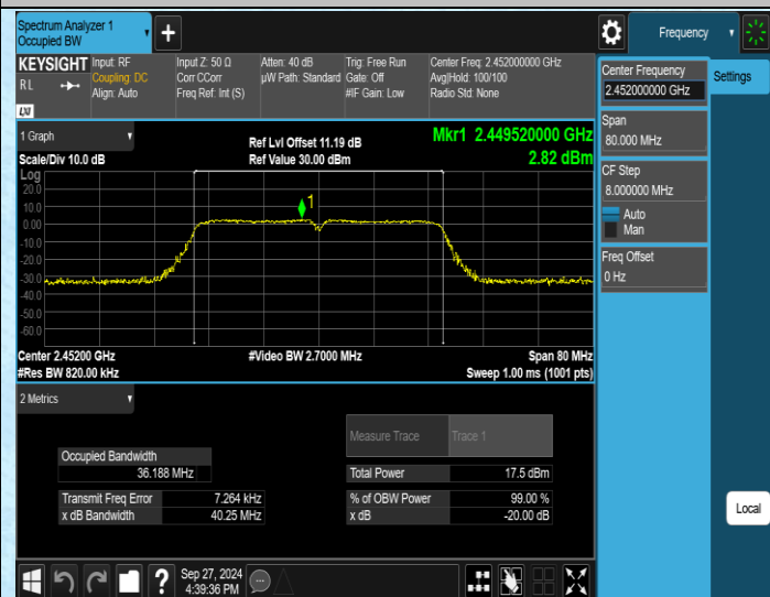
11N40SISO-Ant1-2452
