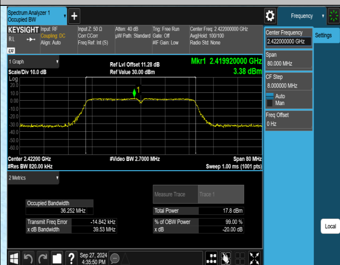
11N40SISO-Ant1-2422
