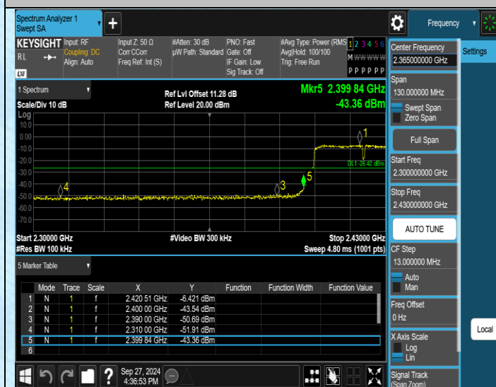
11N40SISO-Ant1-2422-PASS
