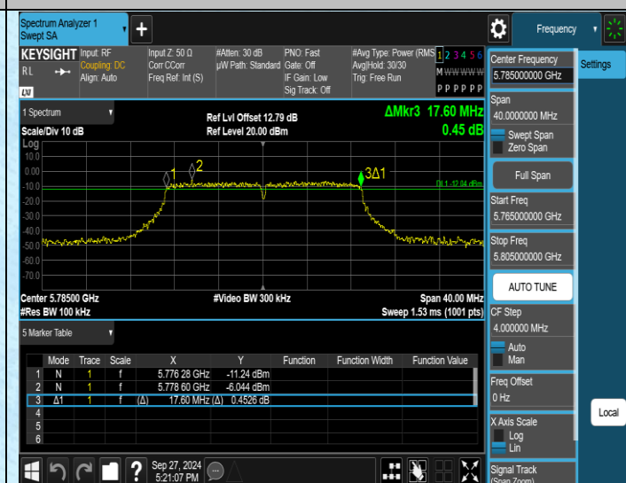
11AC20SISO-Ant1-5785-PASS
