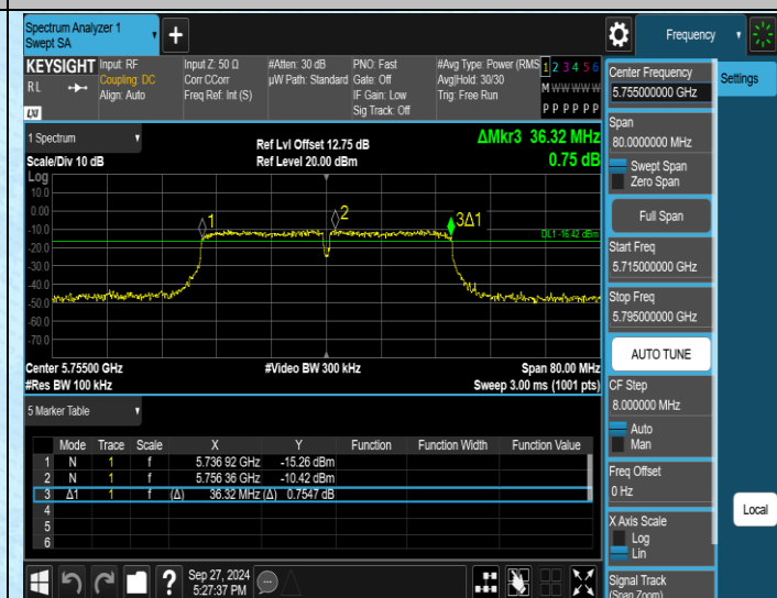
11AC40SISO-Ant1-5755-PASS
