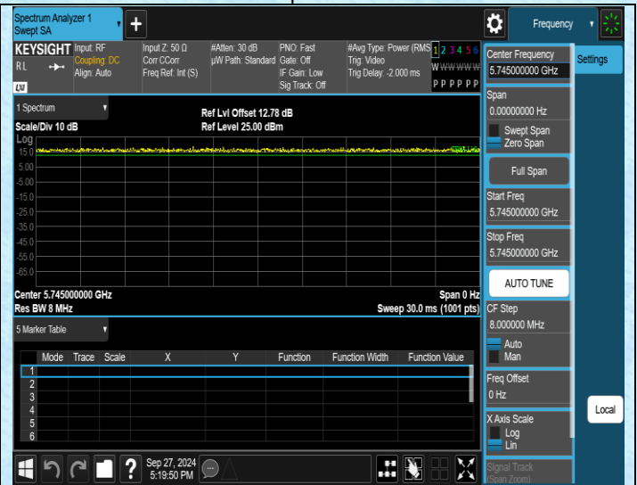
NTNV-11AC20SISO-Ant1-5745
