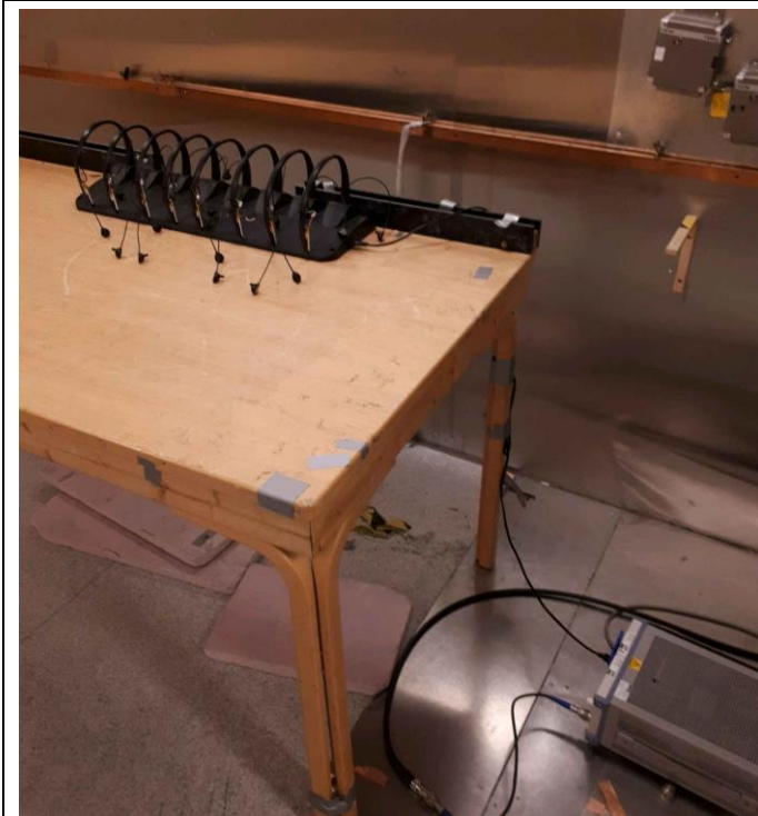
Conducted emissions mains AC
