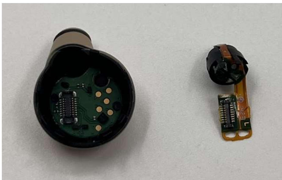
Bottom Half Assembly Angle 7 - Speaker Removed
