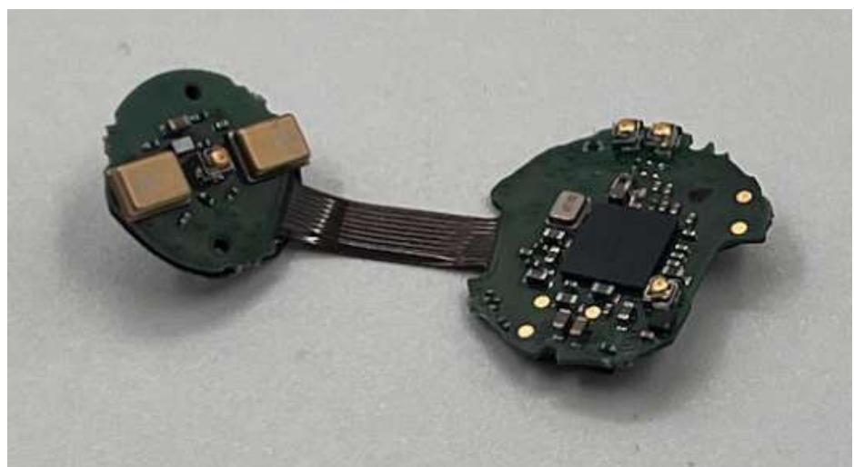
Disassembly Angle 10
