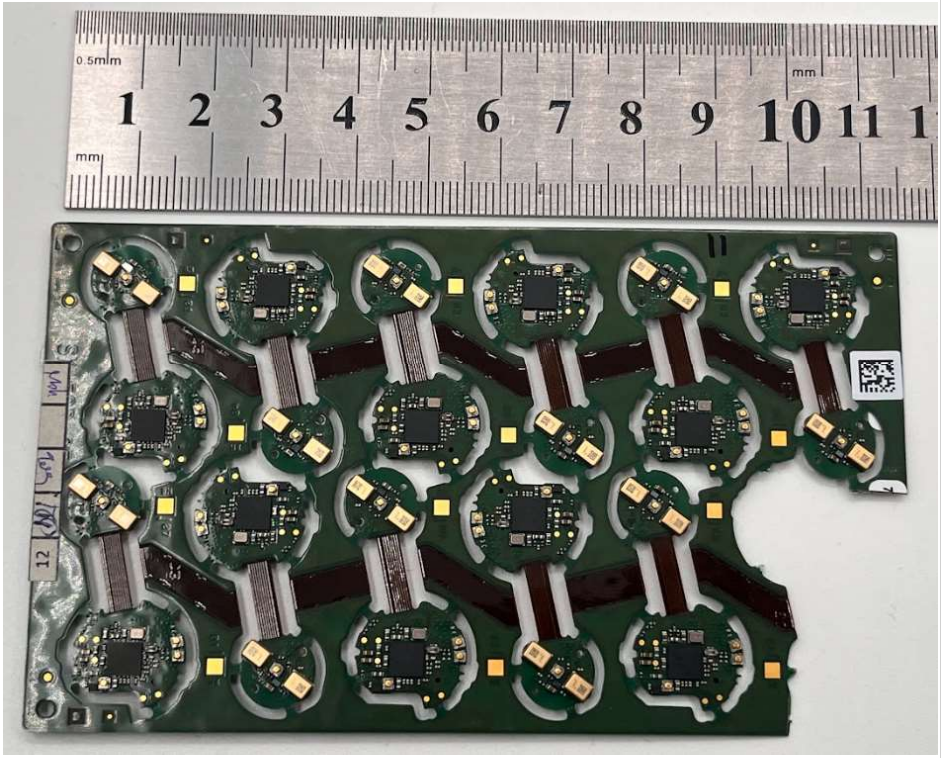
Right Mainboard Panel Top Side
