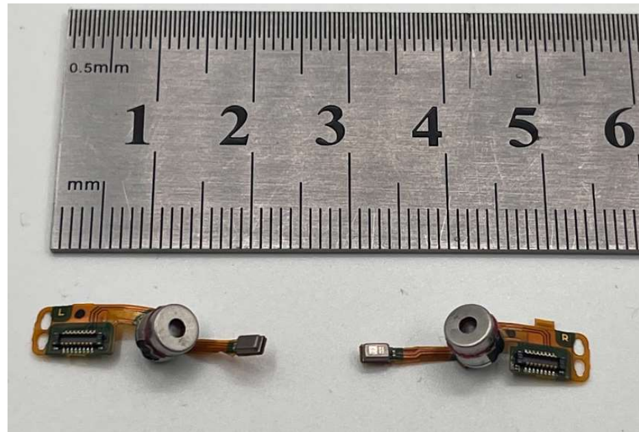
Left and Right Flex PCBs Top Side, from left to right
