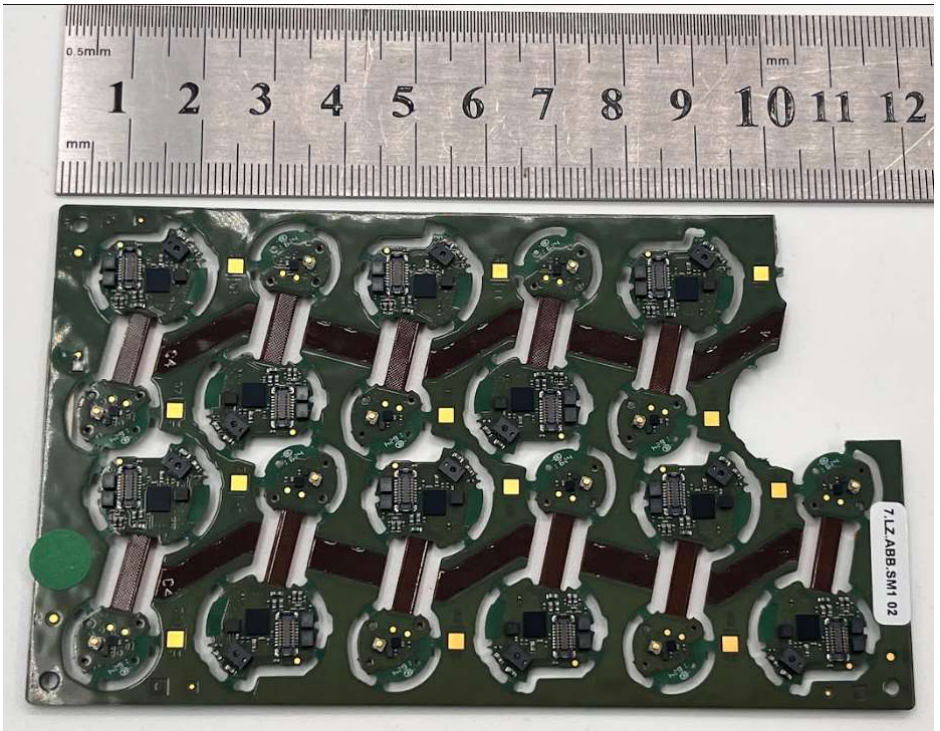
Right Mainboard Panel Bottom Side
