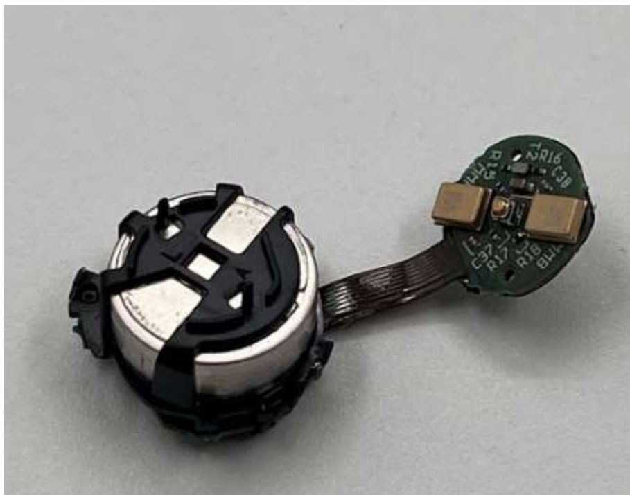
Battery Assembly Angle 6 - Unfolding
