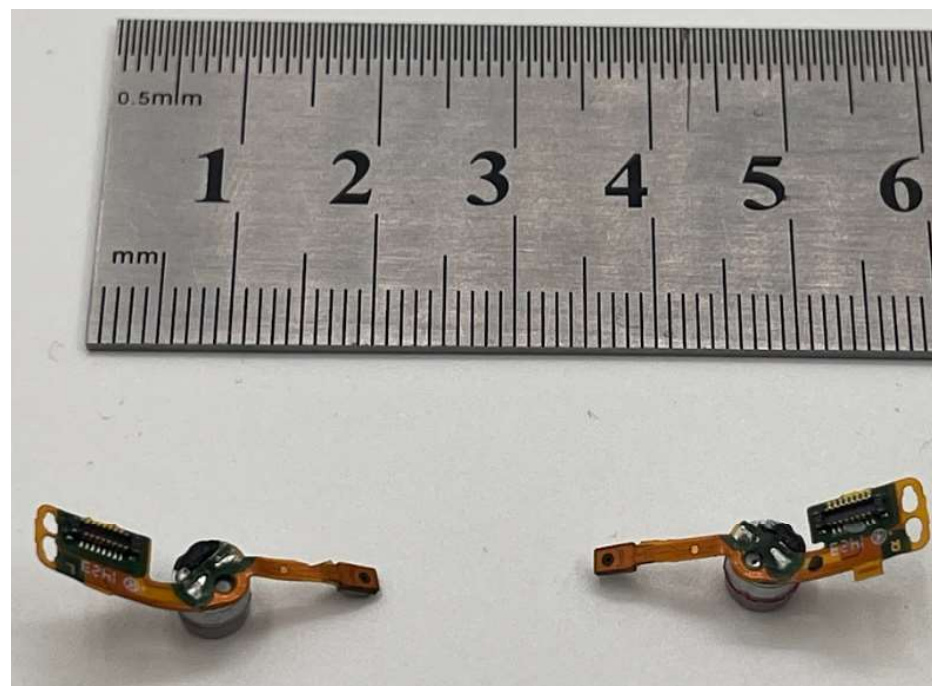
Left and Right Flex PCBs Bottom Side, from left to right
