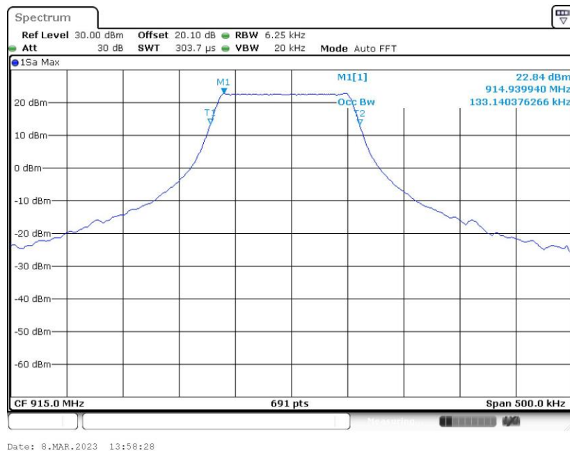
99% Occupied Bandwidth Plot on Channel 65
