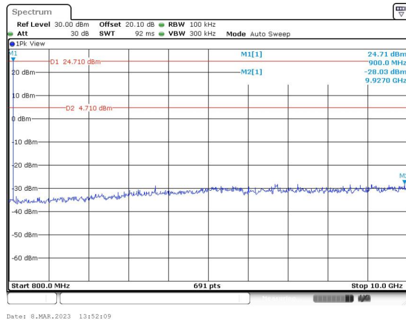
CSE Plot on Ch 2 between 800 MHz ~ 10 GHz
