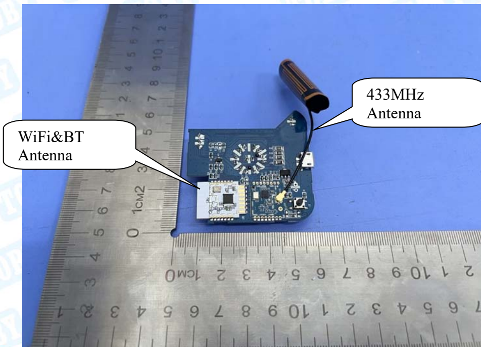
Photo 7 Internal of PCB
