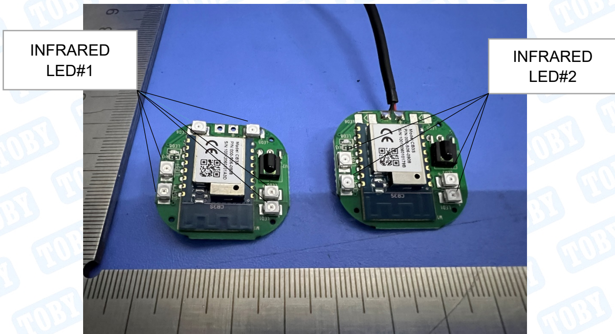
Photo 6 Appearance of PCB
