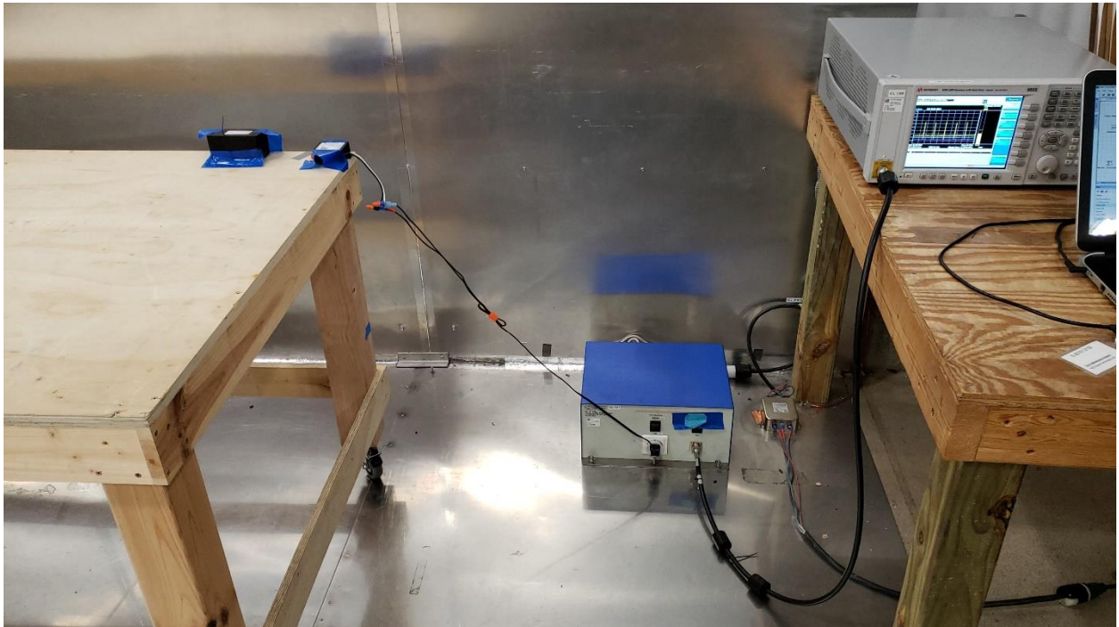
AC Line Conducted Emissions Setup
