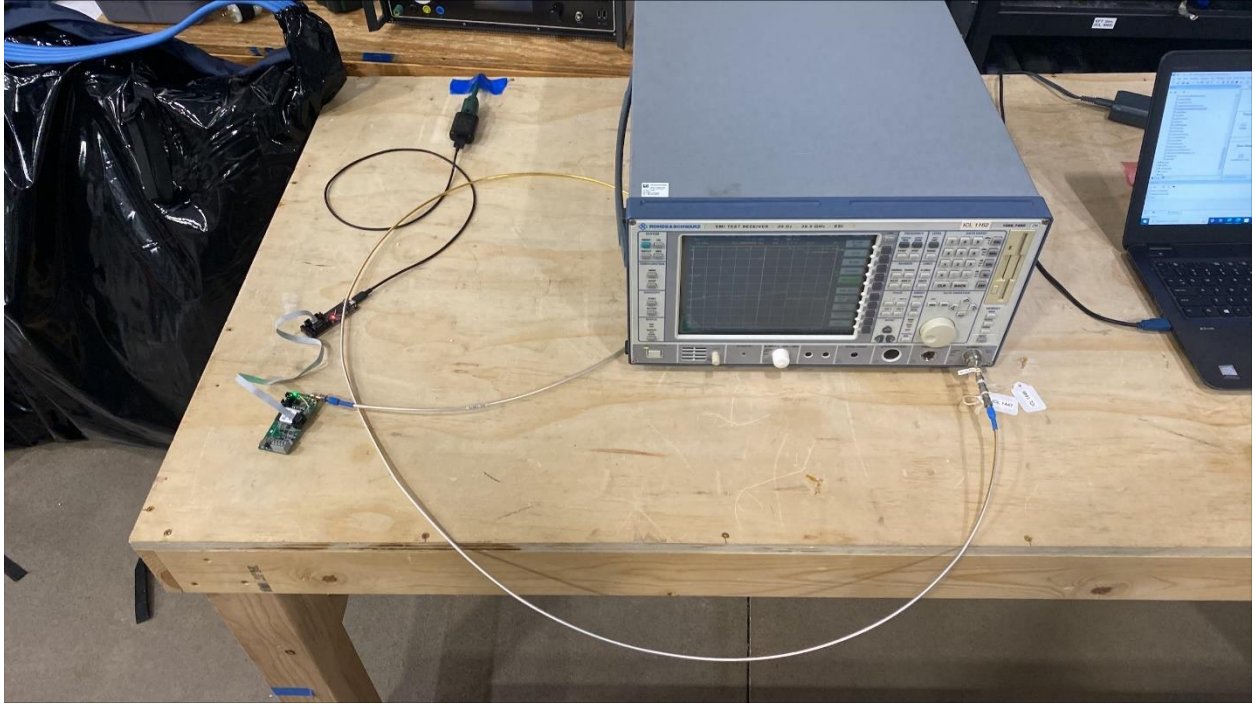
Antenna Port Conducted RF Measurements
