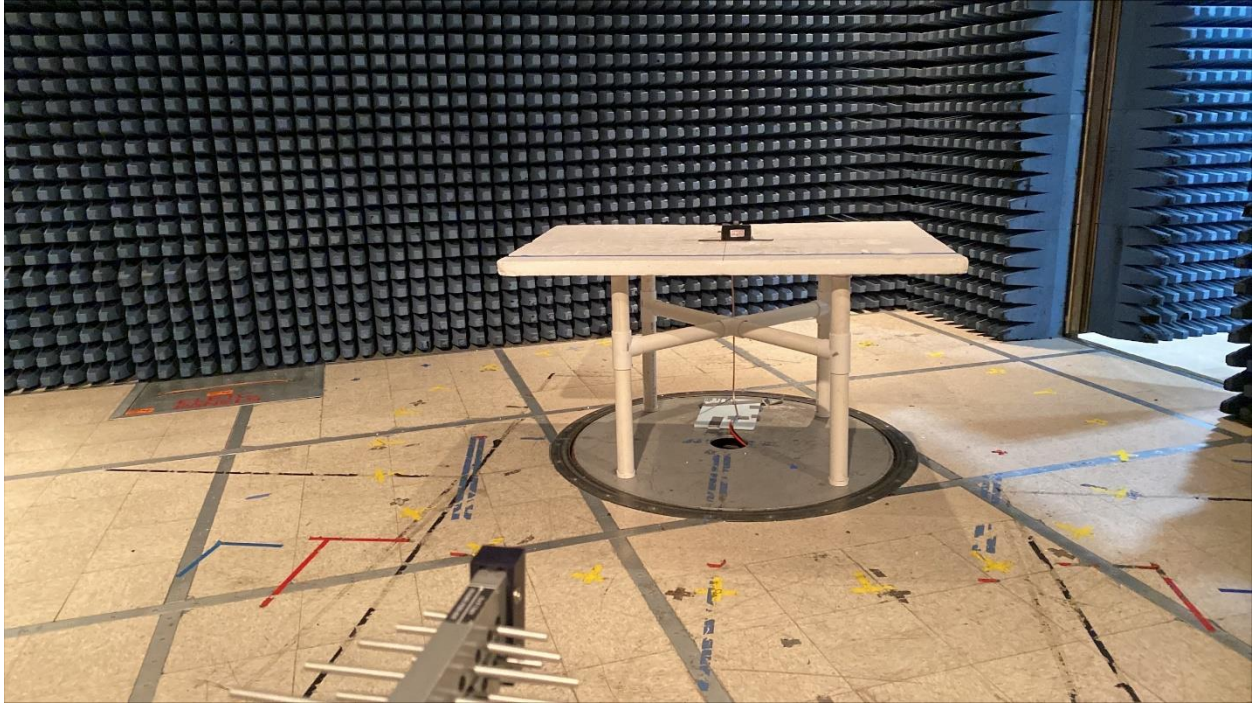
Radiated Emissions Setup: 30MHz to 1GHz
