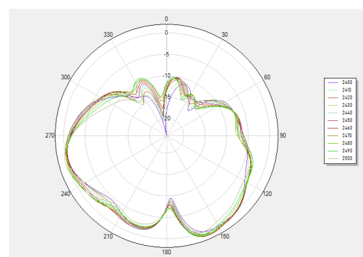
phi 90 2D
