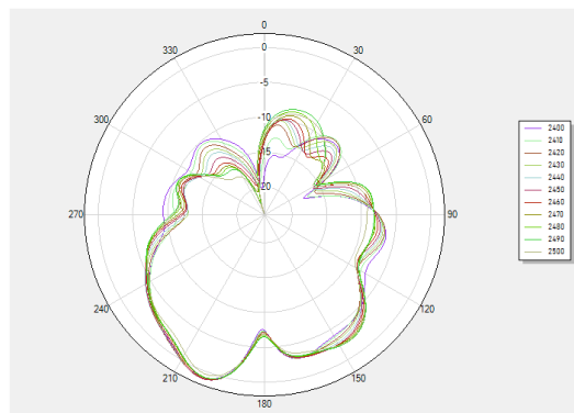
phi 0 2D
