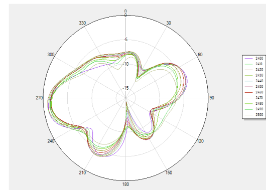
Theta 90 2D
